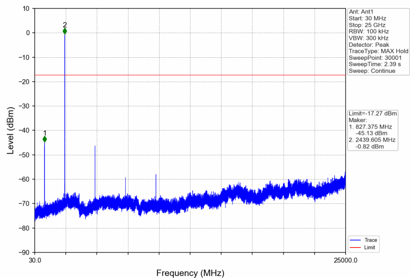
2M_MCH_2440MHz_Ant1_NTN
