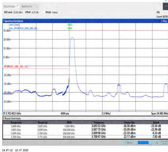
1-N77-3700-3980-PC1.5-30-15-L-1-DFT-PI2BPSK-Edge_1RB_Left-1@0-Ant3-1--PASS-see graph
