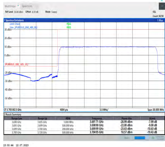
1-N77-3700-3980-PC1.5-30-20-L-3-DFT-PI2BPSK-Out_er_Full-50@0-Ant3-1--PASS-see graph
