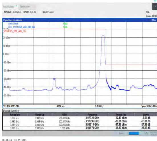
1-N77-3700-3980-PC1.5-30-20-H-2-DFT-PI2BPSK-Ed ge_1RB_Right-1@50-Ant3-1--PASS-see graph
