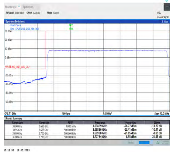
1-N77-3700-3980-PC1.5-30-30-L-3-DFT-PI2BPSK-Outer_Full-75@0-Ant3-1--PASS-see graph
