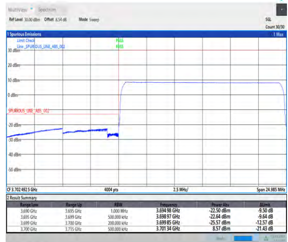
1-N77-3700-3980-PC1.5-30-15-L-6-CP-QPSK-Out er_Full-38@0-Ant3-1--PASS-see graph
