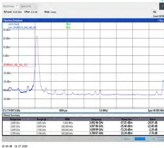
1-N77-3700-3980-PC1.5-30-40-L-1-DFT-PI2BPSK-Edge_1RB_Left-1@0-Ant3-1--PASS-see graph
