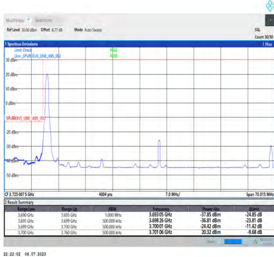
1-N77-3700-3980-PC1-30-60-L-1-DFT-PI2BPSK-Edge_1RB_Left-1@0-Ant3-1--PASS-see graph
