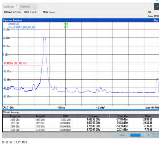
1-N77-3700-3980-PC1.5-30-30-L-1-DFT-PI2BPSK-Edge_1RB_Left-1@0-Ant3-1--PASS-see graph
