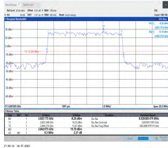
1-N77-3700-3980-PC1.5-30-10-M-2-DFT-PI2BPSK- Outer_Full-24@0-Ant3-8.928-9.30-≤10-PASS
