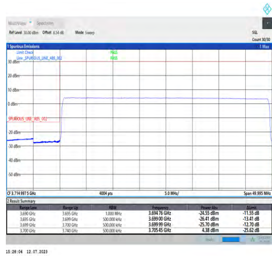
1-N77-3700-3980-PC1.5-30-40-L-6-CP-QPSK-Out er_Full-100@0-Ant3-1--PASS-see graph
