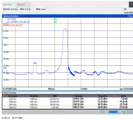
1-N77-3700-3980-PC1.5-30-10-H-5-CP-QPSK-Edge_1RB_Right-1@23-Ant3-1--PASS-see graph
