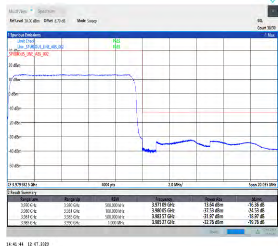
1-N77-3700-3980-PC1.5-30-10-H-3-DFT-PI2BPSK -Outer_Full-24@0-Ant3-1--PASS-see graph
