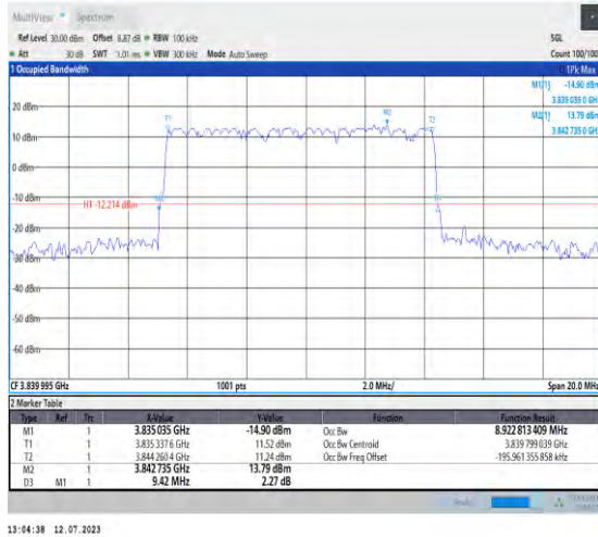
1-N77-3700-3980-PC1.5-30-10-M-1-DFT-QPSK-Out er_Full-24@0-Ant3-8.923-9.420-≤10-PASS
