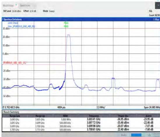
1-N77-3700-3980-PC1.5-30-15-L-4-CP-QPSK-Edge_1 RB_Left-1@0-Ant3-1--PASS-see graph
