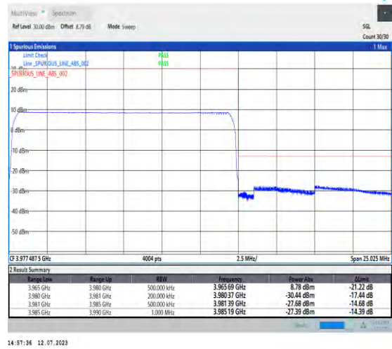
1-N77-3700-3980-PC1.5-30-15-H-6-CP-QPSK-Out_er_Full-38@0-Ant3-1--PASS-see graph
