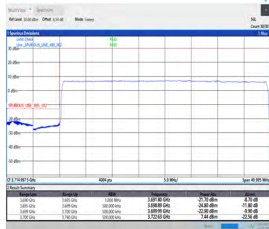
1-N77-3700-3980-PC1.5-30-40-L-3-DFT-PI2BPSK-Outer_Full-100@0-Ant3-1--PASS-see graph
