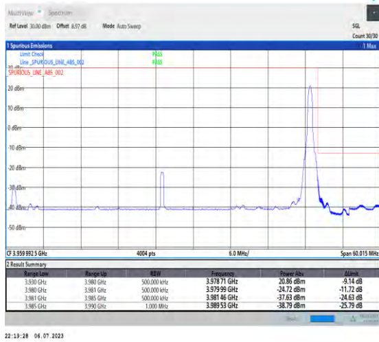
1-N77-3700-3980-PC1-30-50-H-5-CP-QPSK-Edge_1 RB_Right-1@132-Ant3-1--PASS-see graph
