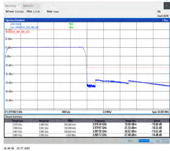
1-N77-3700-3980-PC1.5-30-10-H-6-CP-QPSK-Out_er_Full-24@0-Ant3-1--PASS-see graph
