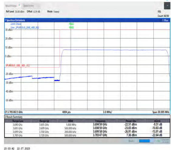
1-N77-3700-3980-PC1.5-30-20-L-6-CP-QPSK-Out er_Full-51@0-Ant3-1--PASS-see graph
