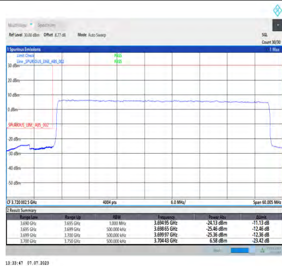
1-N77-3700-3980-PC1-30-50-L-3-DFT-PI2BPSK-Out_er_Full-128@0-Ant3-1--PASS-see graph
