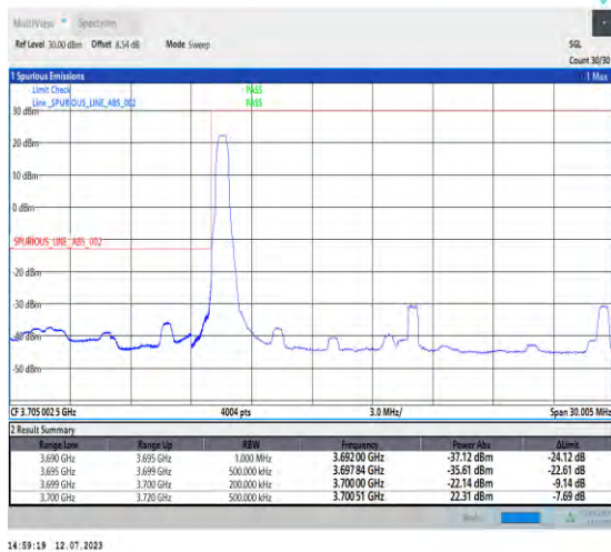
1-N77-3700-3980-PC1.5-30-20-L-1-DFT-PI2BPSK-Edge_1RB_Left-1@0-Ant3-1--PASS-see graph
