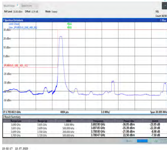
1-N77-3700-3980-PC1.5-30-20-L-4-CP-QPSK-Edge_1 RB_Left-1@0-Ant3-1--PASS-see graph
