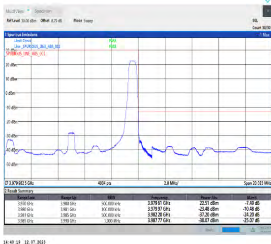
1-N77-3700-3980-PC1.5-30-10-H-2-DFT-PI2BPSK-Ed ge_1RB_Right-1@23-Ant3-1--PASS-see graph
