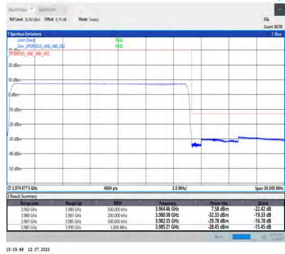
1-N77-3700-3980-PC1.5-30-20-H-6-CP-QPSK-Out_er_Full-51@0-Ant3-1--PASS-see graph
