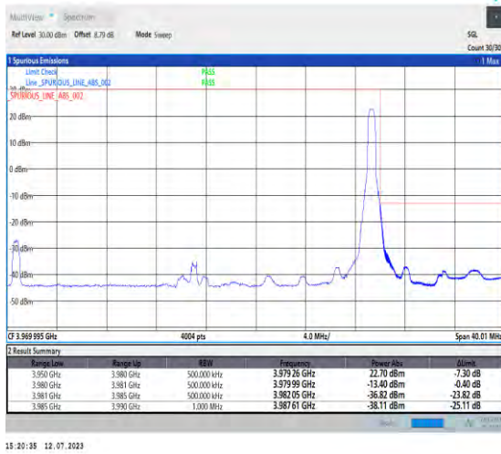
1-N77-3700-3980-PC1.5-30-30-H-5-CP-QPSK-Edge_1RB_Right-1@77-Ant3-1--PASS-see graph
