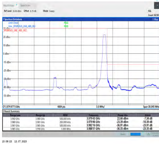
1-N77-3700-3980-PC1.5-30-20-H-5-CP-QPSK-Edge_1RB_Right-1@50-Ant3-1--PASS-see graph
