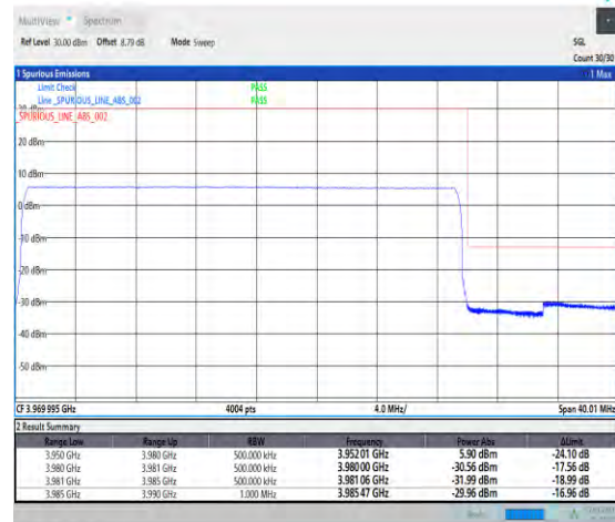
1-N77-3700-3980-PC1.5-30-30-H-6-CP-QPSK-Outer_Full-75@0-Ant3-1--PASS-see graph
