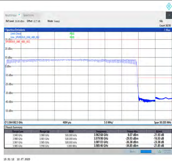
1-N77-3700-3980-PC1.5-30-40-H-3-DFT-PI2BPSK -Outer_Full-100@0-Ant3-1--PASS-see graph
