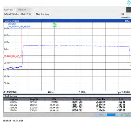
1-N77-3700-3980-PC1-30-60-L-3-DFT-PI2BPSK-Outer_Full-162@0-Ant3-1--PASS-see graph
