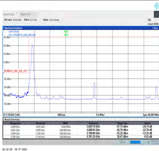
1-N77-3700-3980-PC1-30-50-L-1-DFT-PI2BPSK-Edge_1RB_Left-1@0-Ant3-1--PASS-see graph
