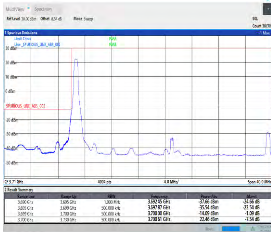
1-N77-3700-3980-PC1.5-30-30-L-4-CP-QPSK-Edge_1 RB_Left-1@0-Ant3-1--PASS-see graph
