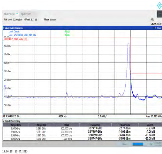
1-N77-3700-3980-PC1.5-30-40-H-5-CP-QPSK-Edge_1RB_Right-1@105-Ant3-1--PASS-see graph
