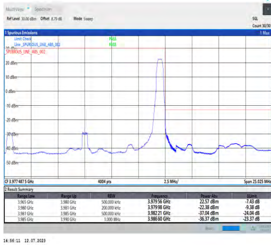
1-N77-3700-3980-PC1.5-30-15-H-5-CP-QPSK-Edge_1RB_Right-1@37-Ant3-1--PASS-see graph
