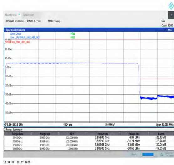
1-N77-3700-3980-PC1.5-30-40-H-6-CP-QPSK-Out_er_Full-100@0-Ant3-1--PASS-see graph
