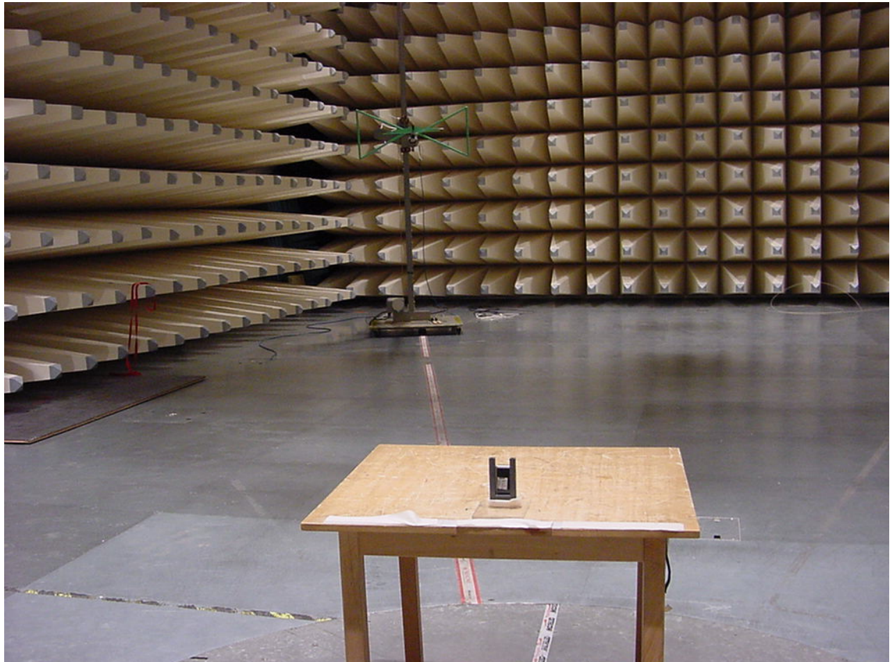
Photo 1: Radiated Emissions
