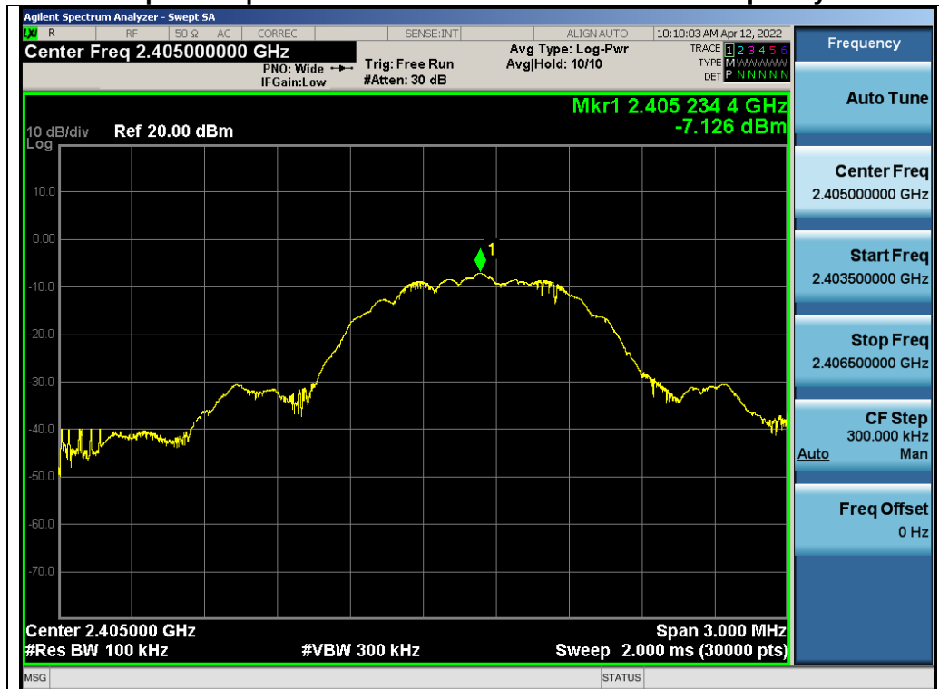
Test_Graph_GFSK_ANT1_2405_1Mbps_Reference Level
