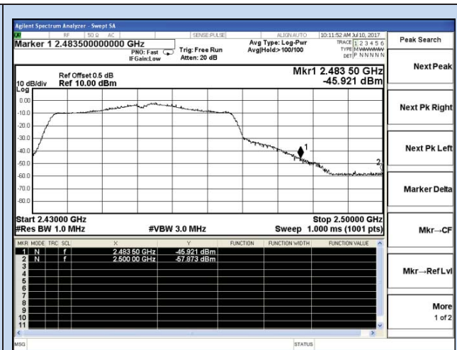
Channel 11 / 2452 MHz – Peak
