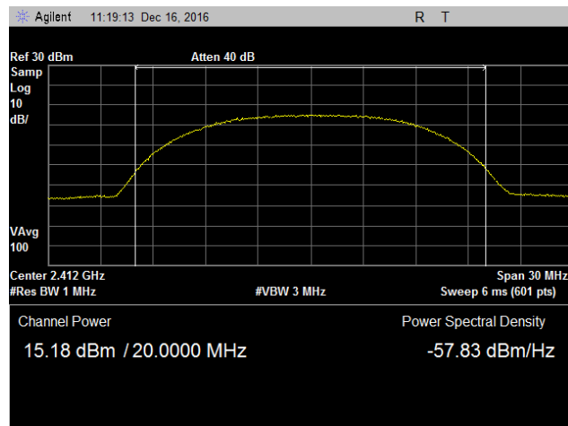
Plot 53. Peak Power Output, Low Channel, 802.11b, Antenna 1, 13 dBi Antenna
