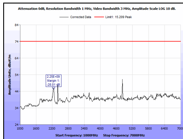
Plot 94. Radiated Spurious Emissions, Low Channel, 802.11g, 1 GHz – 7 GHz, Peak, 9 dBi Antenna
