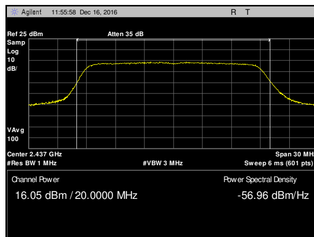
Plot 72. Peak Power Output, Mid Channel, 802.11n 20 MHz, Antenna 2, 13 dBi Antenna
