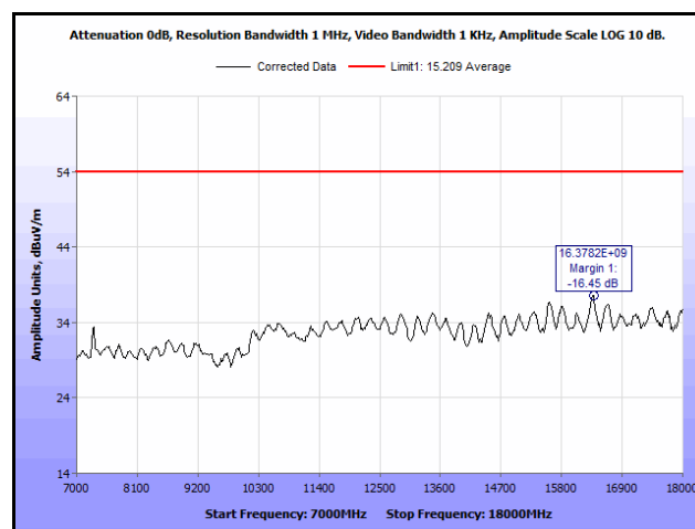
Plot 100. Radiated Spurious Emissions, Mid Channel, 802.11g, 7 GHz – 18 GHz, Average, 9 dBi Antenna
