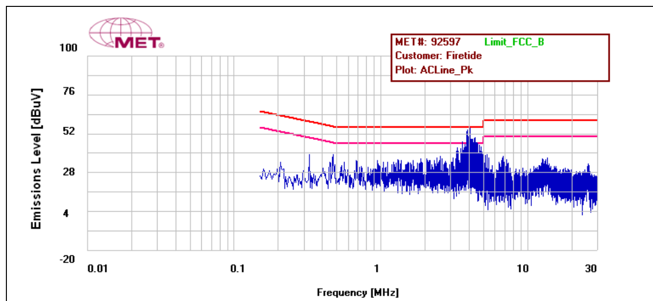
Plot 1. Conducted Emissions, 15.207(a), Phase Line, 9 dBi Antenna
