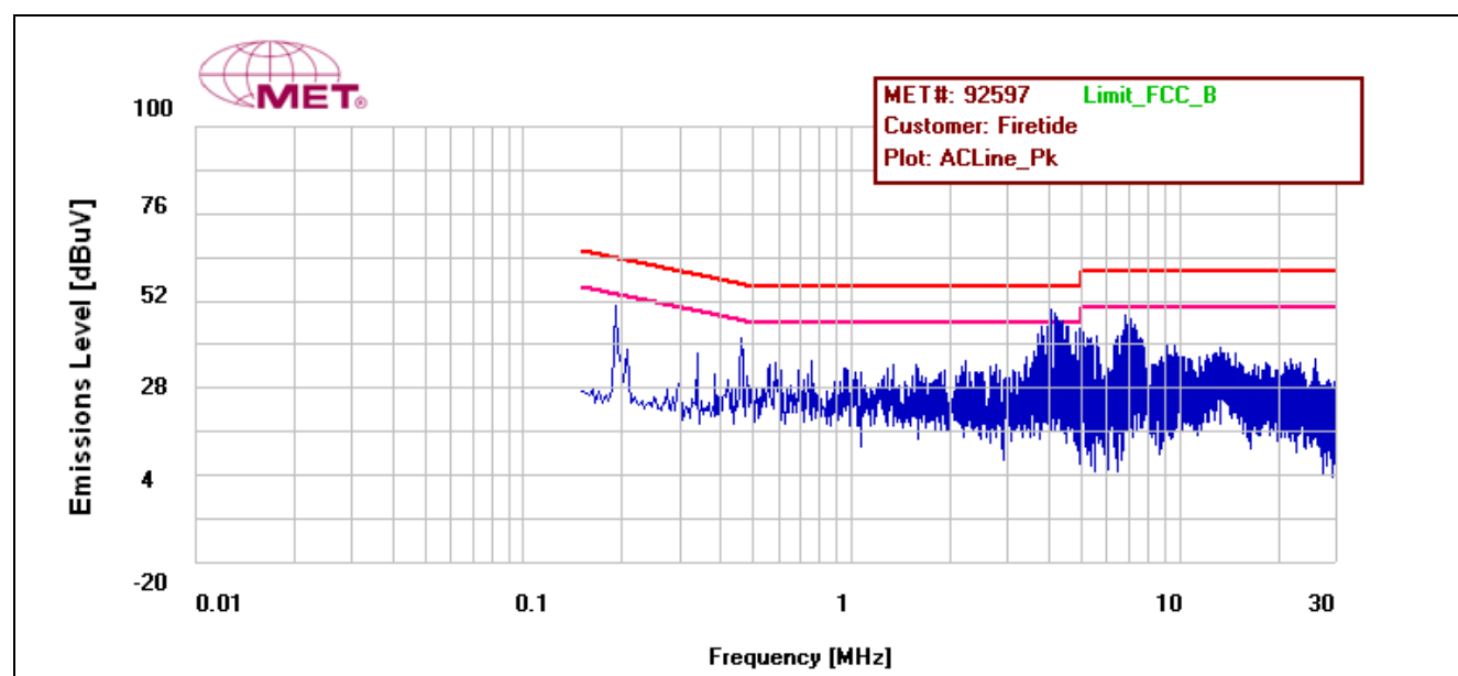
Plot 3. Conducted Emissions, 15.207(a), Phase Line, 13 dBi Antenna
