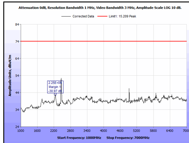
Plot 89. Radiated Spurious Emissions, High Channel, 802.11b, 1 GHz – 7 GHz, Peak, 9 dBi Antenna
