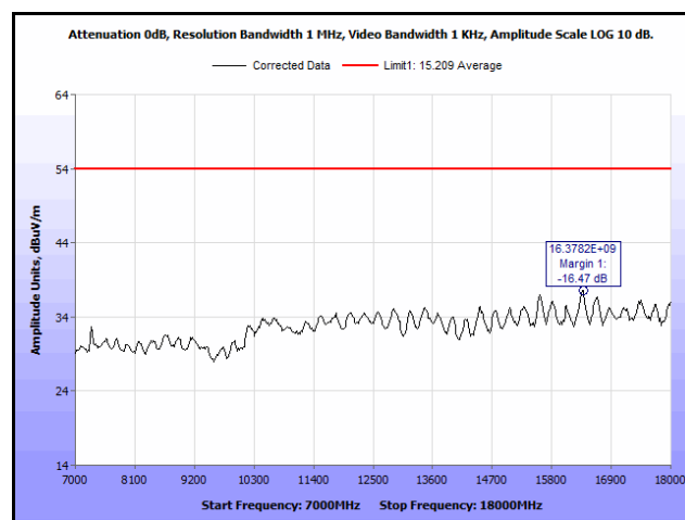
Plot 115. Radiated Spurious Emissions, Mid Channel, 802.11n 20 MHz, 7 GHz – 18 GHz, Average, 9 dBi Antenna
