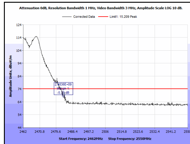
Plot 220. Radiated Restricted Band Edge, High Channel, 802.11g, Peak, 13 dBi Antenna
