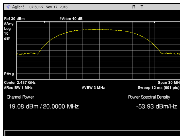
Plot 42. Peak Power Output, Mid Channel, 802.11b, Antenna 2, 9 dBi Antenna
