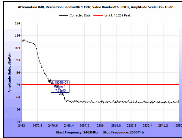
Plot 204. Radiated Restrictred Band Edge, High Channel, 802.11g, Peak, 9 dBi Antenna
