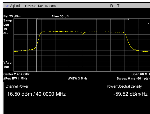
Plot 75. Peak Power Output, Mid Channel, 802.11n 40 MHz, Antenna 2, 13 dBi Antenna
