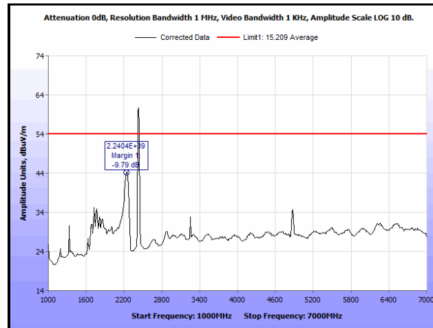
Plot 173. Radiated Spurious Emissions, Mid Channel, 802.11n 20 MHz, 1 GHz – 7 GHz, Average, 13 dBi Antenna
