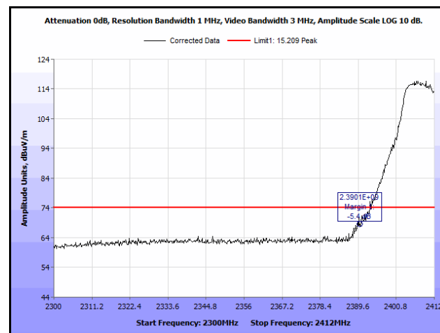
Plot 222. Radiated Restricted Band Edge, Low Channel, 802.11n 20 MHz, Peak, 13 dBi Antenna
