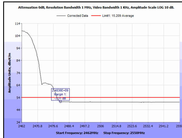
Plot 199. Radiated Restricted Band Edge, High Channel, 802.11b, Average, 9 dBi Antenna
