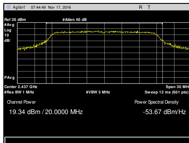
Plot 48. Peak Power Output, Mid Channel, 802.11n 20 MHz, Antenna 2, 9 dBi Antenna
