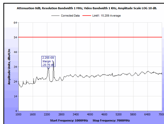
Plot 118. Radiated Spurious Emissions, High Channel, 802.11n 20 MHz, 1 GHz – 7 GHz, Average, 9 dBi Antenna
