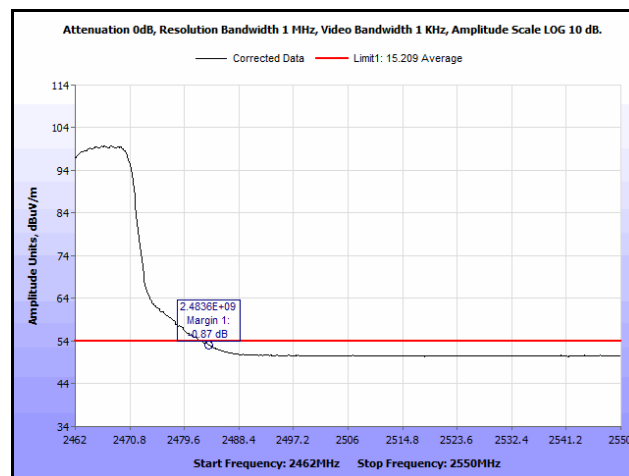
Plot 207. Radiated Restricted Band Edge, High Channel, 802.11n 20 MHz, Average, 9 dBi Antenna
