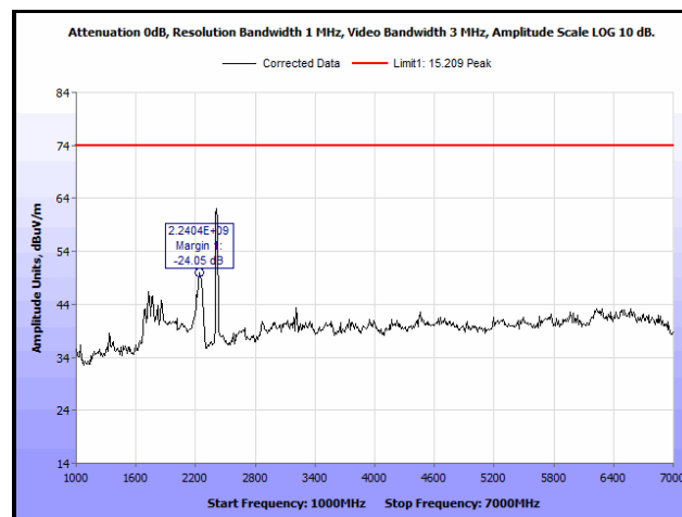
Plot 154. Radiated Spurious Emissions, Low Channel, 802.11g, 1 GHz – 7 GHz, Peak, 13 dBi Antenna
