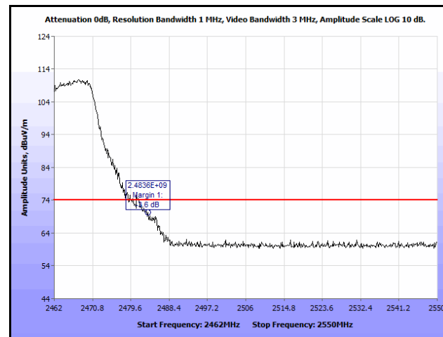
Plot 208. Radiated Restricted Band Edge, High Channel, 802.11n 20 MHz, Peak, 9 dBi Antenna
