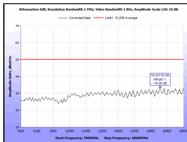
Plot 145. Radiated Spurious Emissions, Mid Channel, 802.11b, 7 GHz – 18 GHz, Average, 13 dBi Antenna
