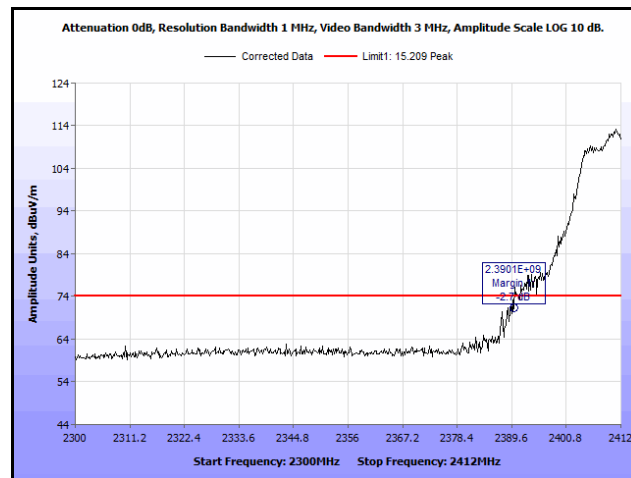
Plot 202. Radiated Restricted Band Edge, Low Channel, 802.11g, Peak, 9 dBi Antenna
