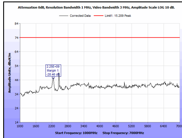
Plot 119. Radiated Spurious Emissions, High Channel, 802.11n 20 MHz, 1 GHz – 7 GHz, Peak, 9 dBi Antenna
