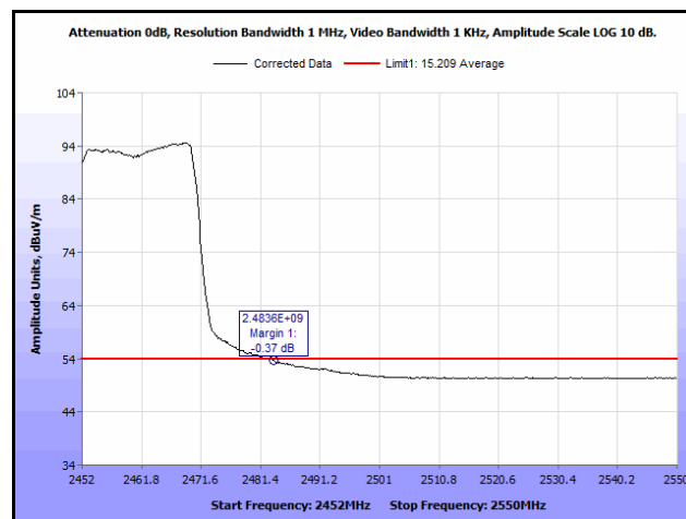
Plot 211. Radiated Restricted Band Edge, High Channel, 802.11n 40 MHz, Average, 9 dBi Antenna
