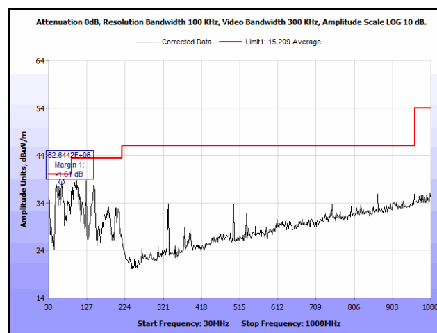
Plot 187. Radiated Spurious Emissions, Mid Channel, 802.11n 40 MHz, 30 MHz – 1 GHz, 13 dBi Antenna
