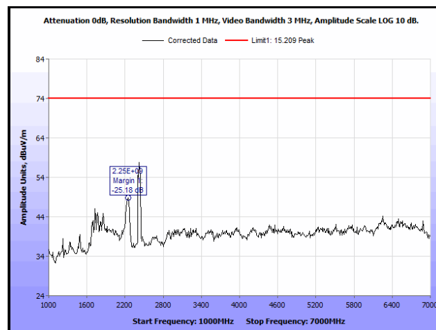
Plot 184. Radiated Spurious Emissions, Low Channel, 802.11n 40 MHz, 1 GHz – 7 GHz, Peak, 13 dBi Antenna
