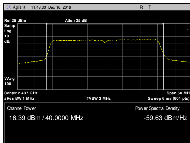
Plot 63. Peak Power Output, Mid Channel, 802.11n 40 MHz, Antenna 1, 13 dBi Antenna
