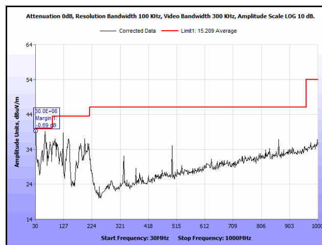
Plot 112. Radiated Spurious Emissions, Mid Channel, 802.11n 20 MHz, 30 MHz – 1 GHz, 9 dBi Antenna
