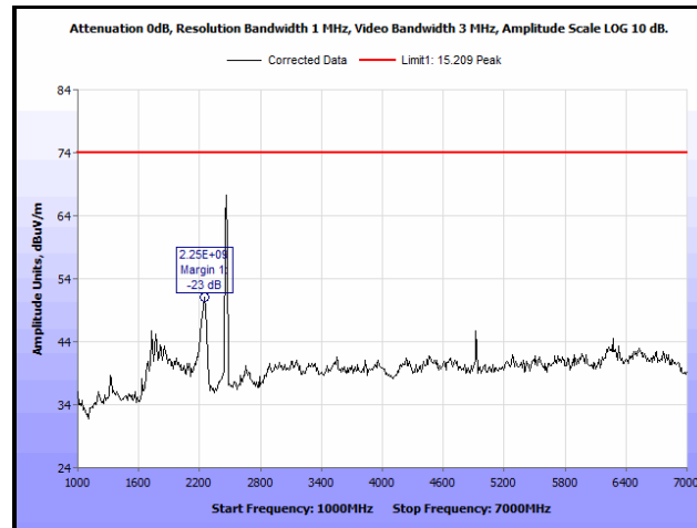
Plot 149. Radiated Spurious Emissions, High Channel, 802.11b, 1 GHz – 7 GHz, Peak, 13 dBi Antenna
