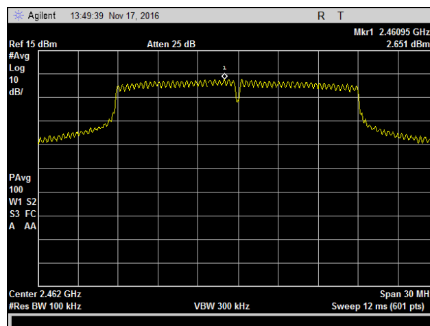
Plot 374. Peak Power Spectral Density, High Channel, 802.11g, Antenna 2, 9 dBi
