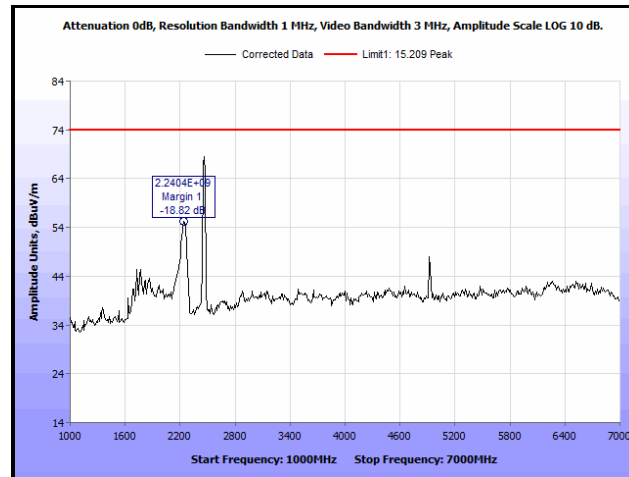
Plot 164. Radiated Spurious Emissions, High Channel, 802.11g, 1 GHz – 7 GHz, Peak, 13 dBi Antenna
