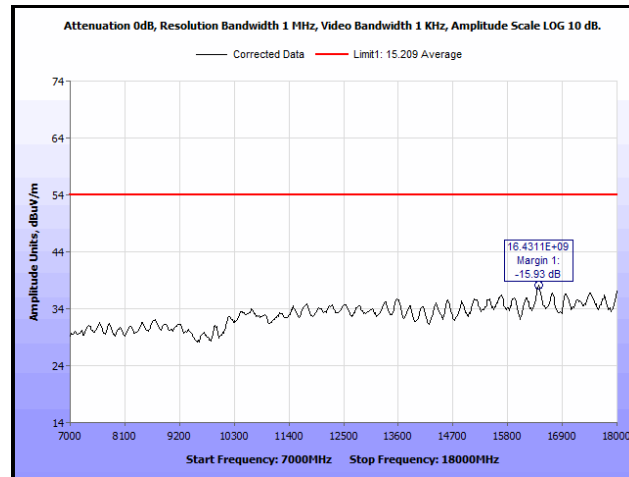
Plot 170. Radiated Spurious Emissions, Low Channel, 802.11n 20 MHz, 7 GHz – 18 GHz, Average, 13 dBi Antenna
