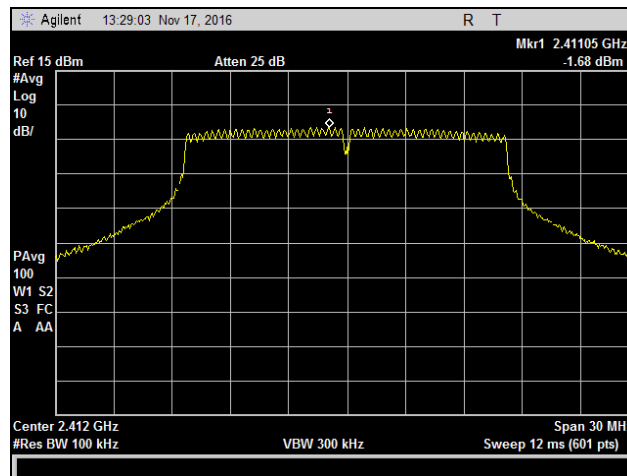
Plot 372. Peak Power Spectral Density, Low Channel, 802.11g, Antenna 2, 9 dBi
