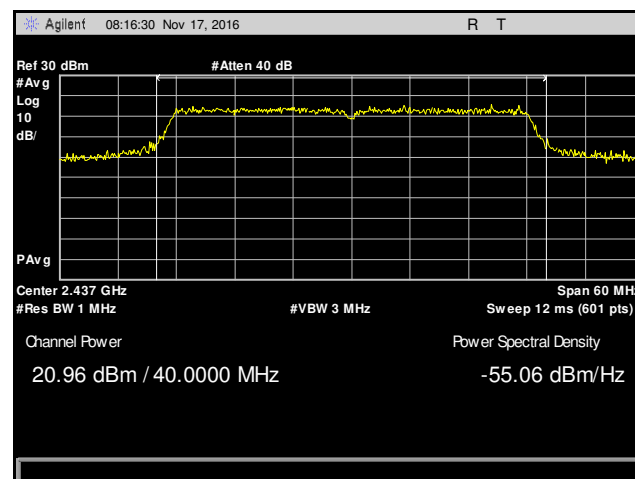
Plot 51. Peak Power Output, Mid Channel, 802.11n 40 MHz, Antenna 2, 9 dBi Antenna
