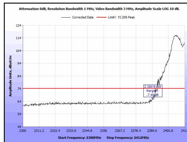
Plot 218. Radiated Restricted Band Edge, Low Channel, 802.11g, Peak, 13 dBi Antenna
