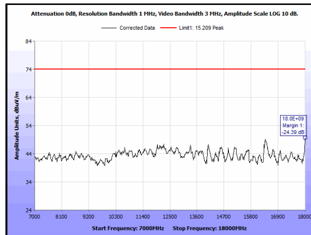
Plot 171. Radiated Spurious Emissions, Low Channel, 802.11n 20 MHz, 7 GHz – 18 GHz, Peak, 13 dBi Antenna
