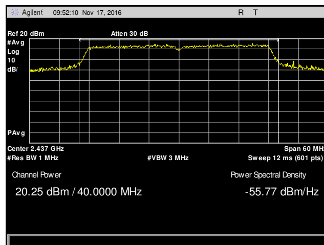
Plot 39. Peak Power Output, Mid Channel, 802.11n 40 MHz, Antenna 1, 9 dBi Antenna
