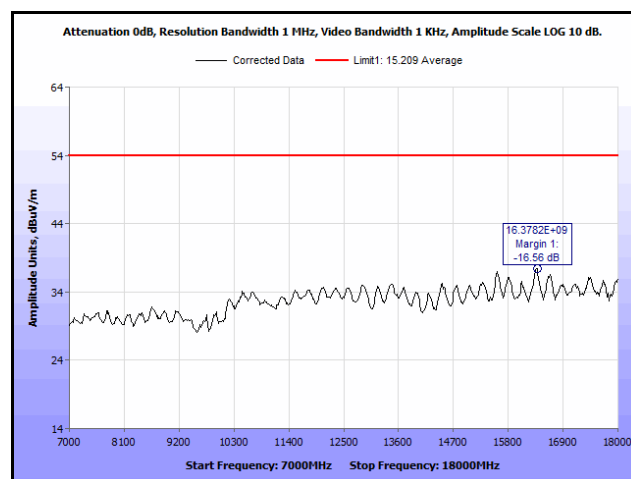
Plot 85. Radiated Spurious Emissions, Mid Channel, 802.11b, 7 GHz – 18 GHz, Average, 9 dBi Antenna
