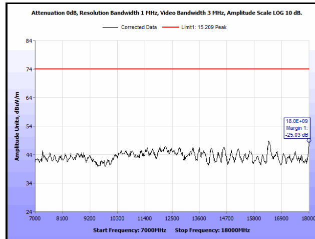
Plot 176. Radiated Spurious Emissions, Mid Channel, 802.11n 20 MHz, 7 GHz – 18 GHz, Peak, 13 dBi Antenna
