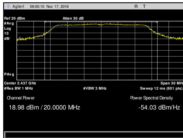
Plot 33. Peak Power Output, Mid Channel, 802.11g, Antenna 1, 9 dBi Antenna
