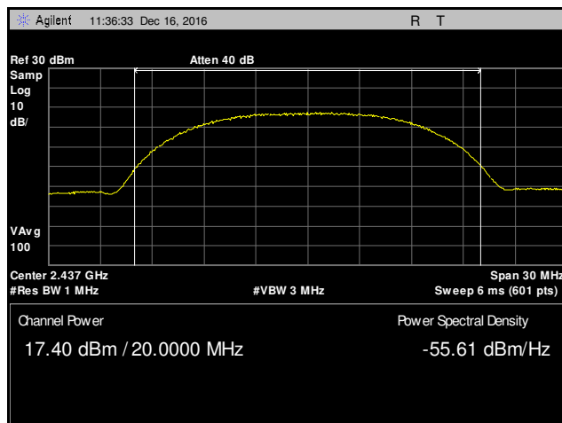
Plot 54. Peak Power Output, Mid Channel, 802.11b, Antenna 1, 13 dBi Antenna
