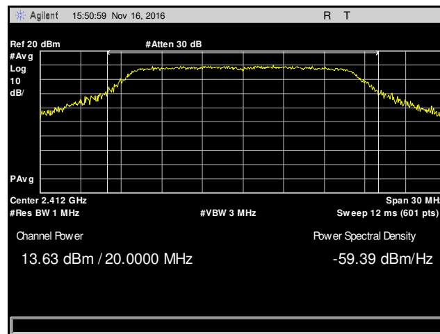
Plot 68. Peak Power Output, Low Channel, 802.11g, Antenna 2, 13 dBi Antenna
