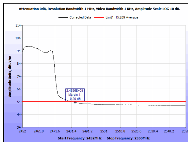
Plot 227. Radiated Restricted Band Edge, High Channel, 802.11n 40 MHz, Average, 13 dBi Antenna
