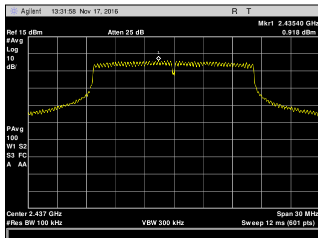
Plot 373. Peak Power Spectral Density, Mid Channel, 802.11g, Antenna 2, 9 dBi
