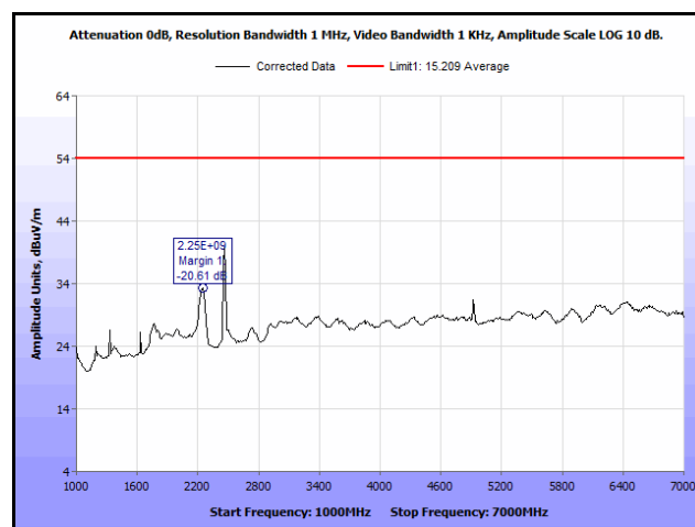
Plot 103. Radiated Spurious Emissions, High Channel, 802.11g, 1 GHz – 7 GHz, Average, 9 dBi Antenna
