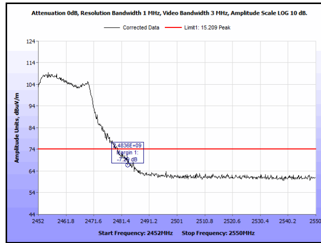
Plot 228. Radiated Restricted Band Edge, High Channel, 802.11n 40 MHz, Peak, 13 dBi Antenna
