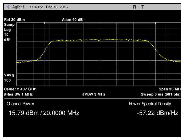
Plot 60. Peak Power Output, Mid Channel, 802.11n 20 MHz, Antenna 1, 13 dBi Antenna
