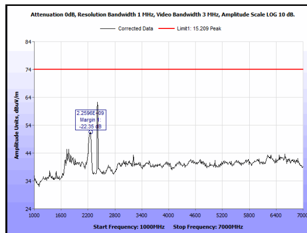
Plot 169. Radiated Spurious Emissions, Low Channel, 802.11n 20 MHz, 1 GHz – 7 GHz, Peak, 13 dBi Antenna
