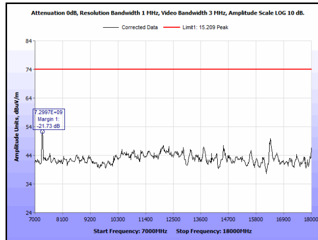
Plot 101. Radiated Spurious Emissions, Mid Channel, 802.11g, 7 GHz – 18 GHz, Peak, 9 dBi Antenna
