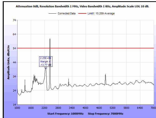
Plot 158. Radiated Spurious Emissions, Mid Channel, 802.11g, 1 GHz – 7 GHz, Average, 13 dBi Antenna
