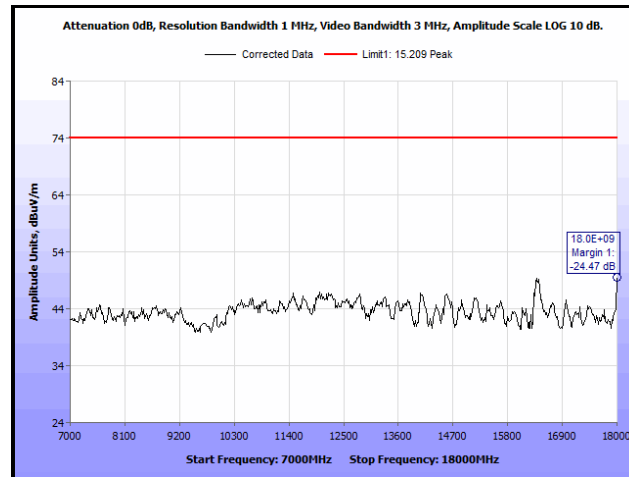
Plot 146. Radiated Spurious Emissions, Mid Channel, 802.11b, 7 GHz – 18 GHz, Peak, 13 dBi Antenna
