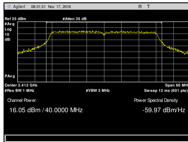
Plot 50. Peak Power Output, Low Channel, 802.11n 40 MHz, Antenna 2, 9 dBi Antenna
