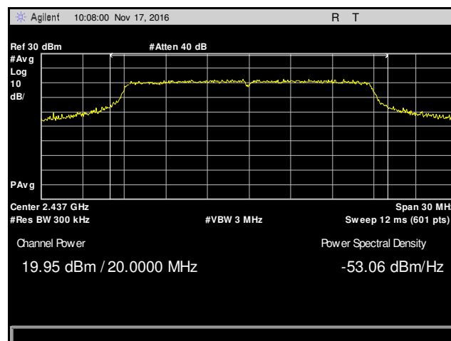
Plot 36. Peak Power Output, Mid Channel, 802.11n 20 MHz, Antenna 1, 9 dBi Antenna
