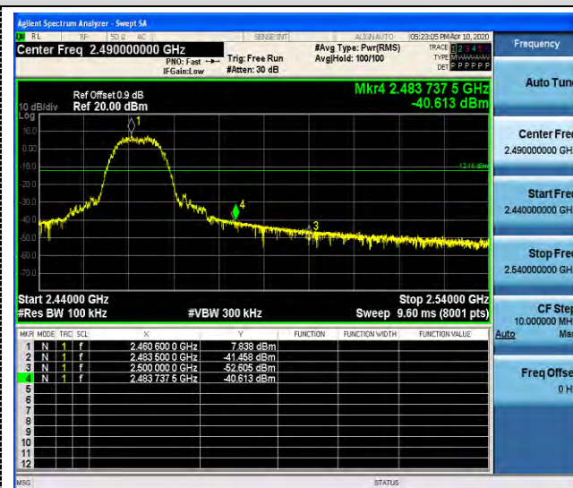
Right bandedge
