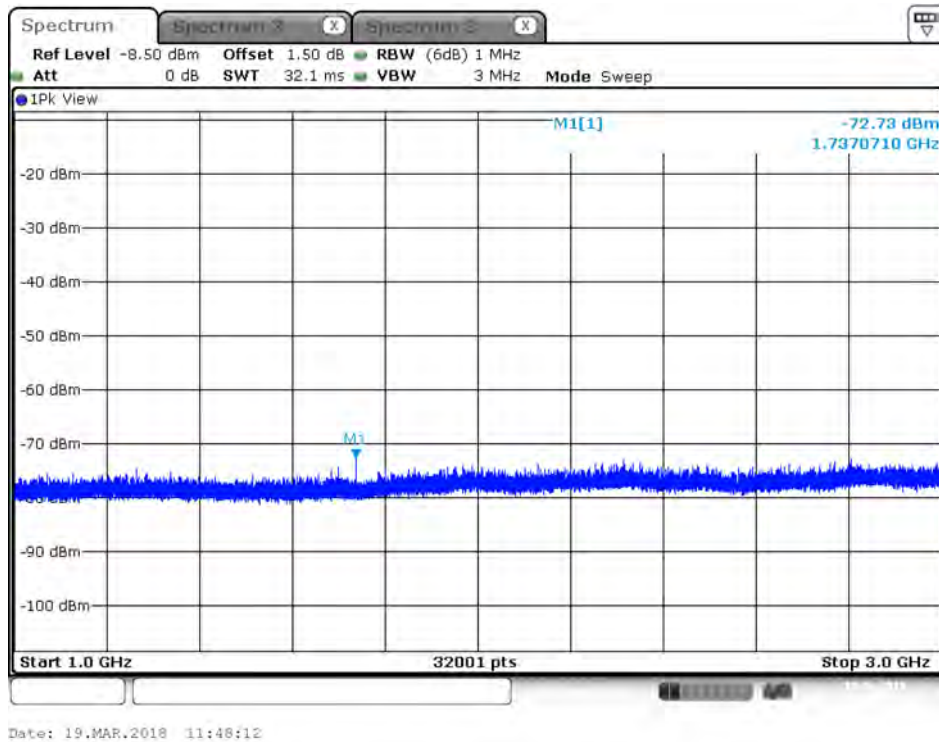
Plot on IEEE 802.11ac Nss1 MCS0 VHT20 / 5580 MHz / Peak / Port 1 / 1GHz~3GHz
