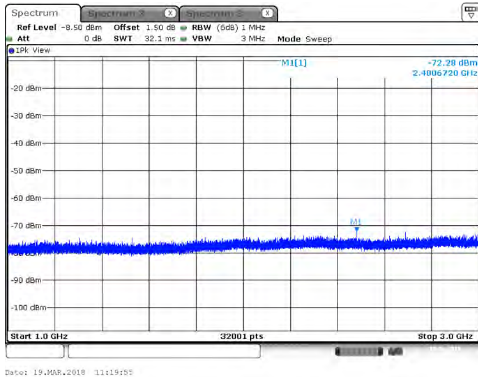
Plot on IEEE 802.11ac Nss1 MCS0 VHT20 / 5500 MHz / Peak / Port 1 / 1GHz~3GHz
