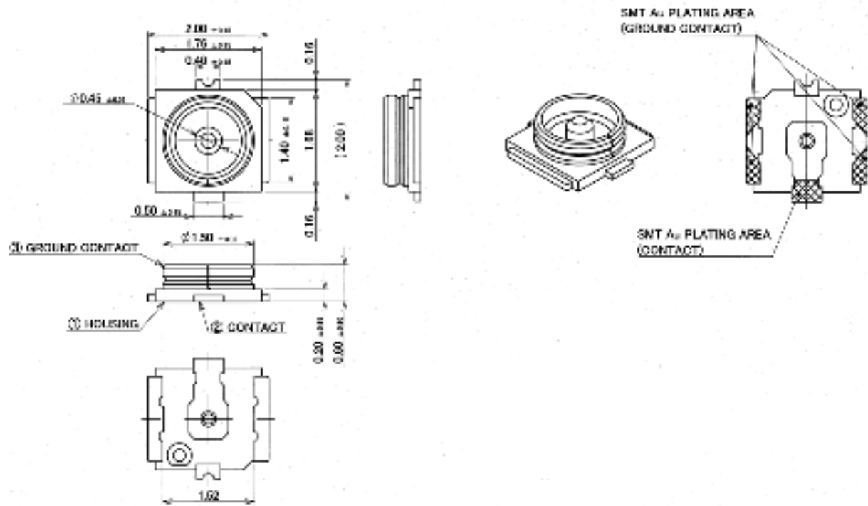
Figure 25: Dimensions of the Receptacle (Unit: mm)
