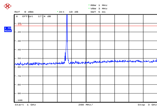
WCDMA Band IV CH-Middle 1GHz ~3GHz
