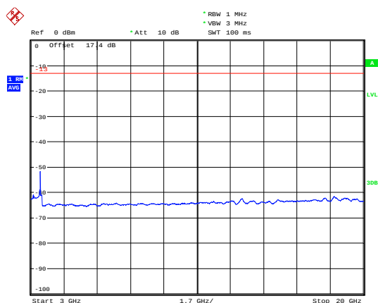
LTE Band 4 5MHz CH-Middle 3GHz~20GHz
