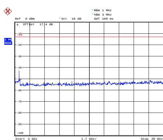
WCDMA Band IV CH-Middle 3GHz ~20GHz
