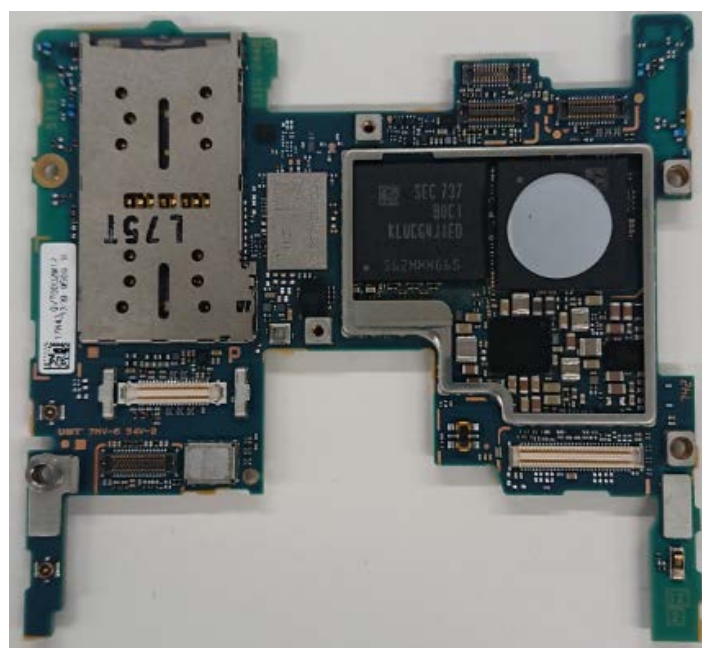
Internal PWB without Shield cases (Front-side)
