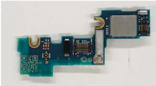
Internal Main_ANT-1-PWB (Front-side)
