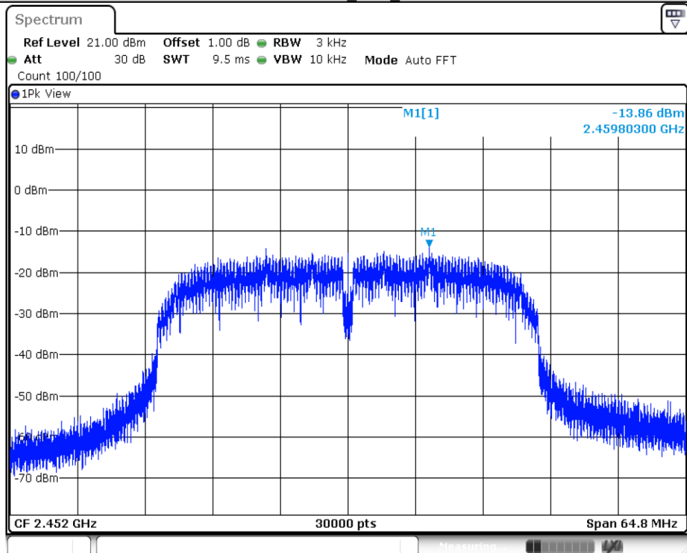
11N40SISO_Ant1_2452
