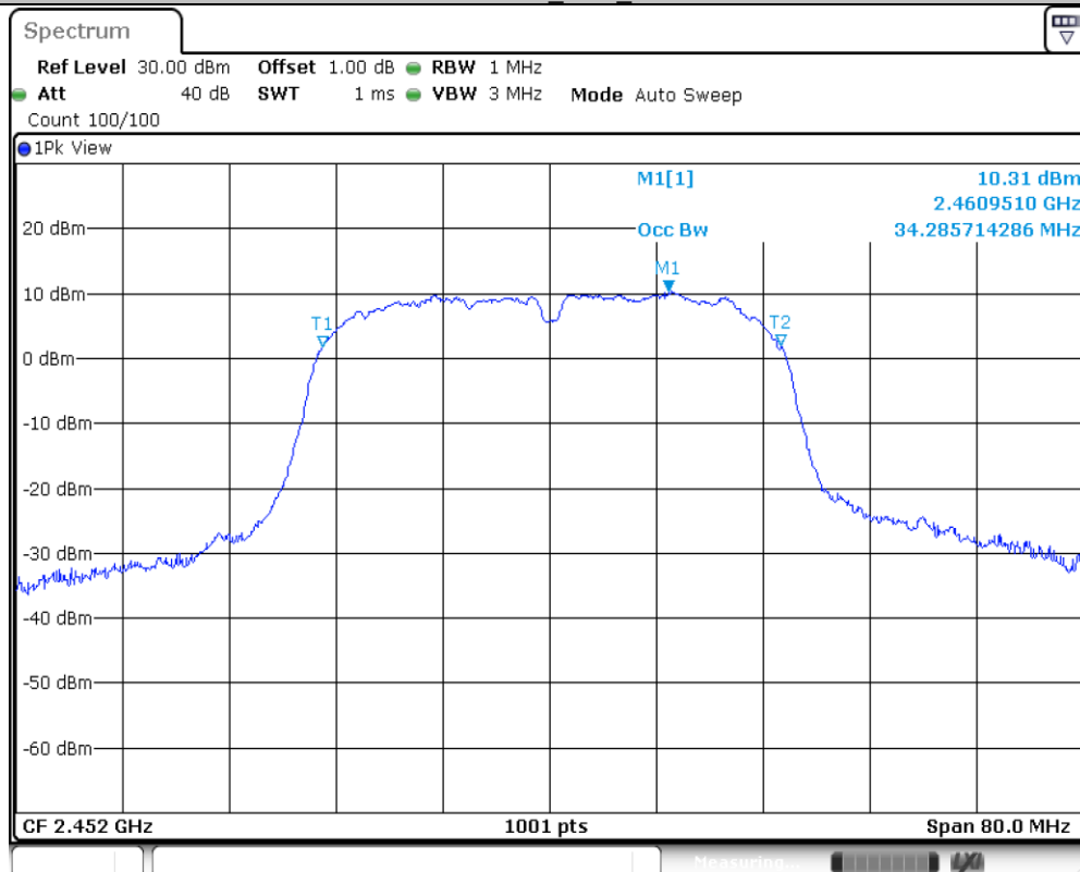
11N40SISO_Ant1_2452
