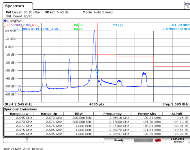
Band7_15MHz_16QAM_21375_75RB#0
