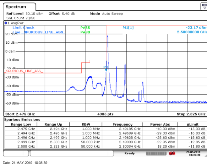
Band7_5MHz_QPSK_20775_25RB#0
