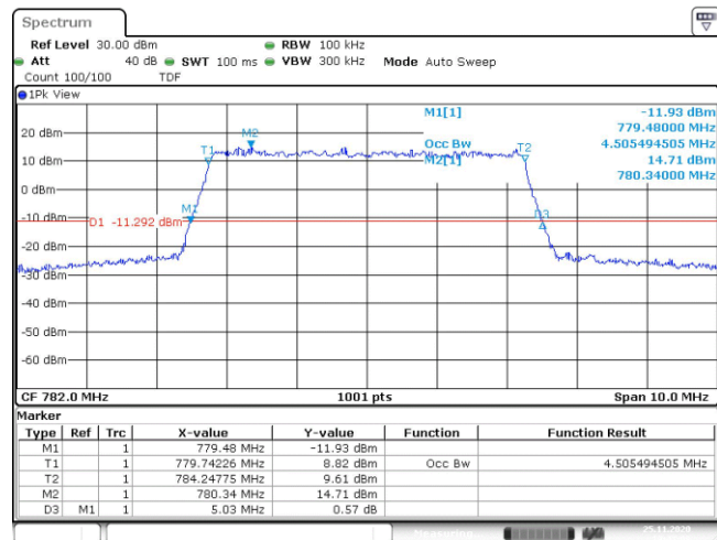
Band13-5MHz-QPSK-23230-25RB#0-4.505
