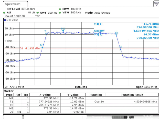
Band13-5MHz-QPSK-23205-25RB#0-4.505
