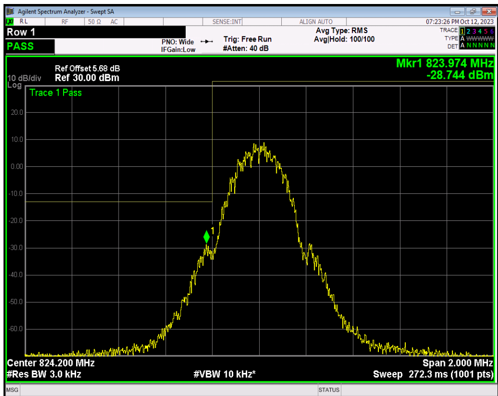
GSM850 Channel=128
