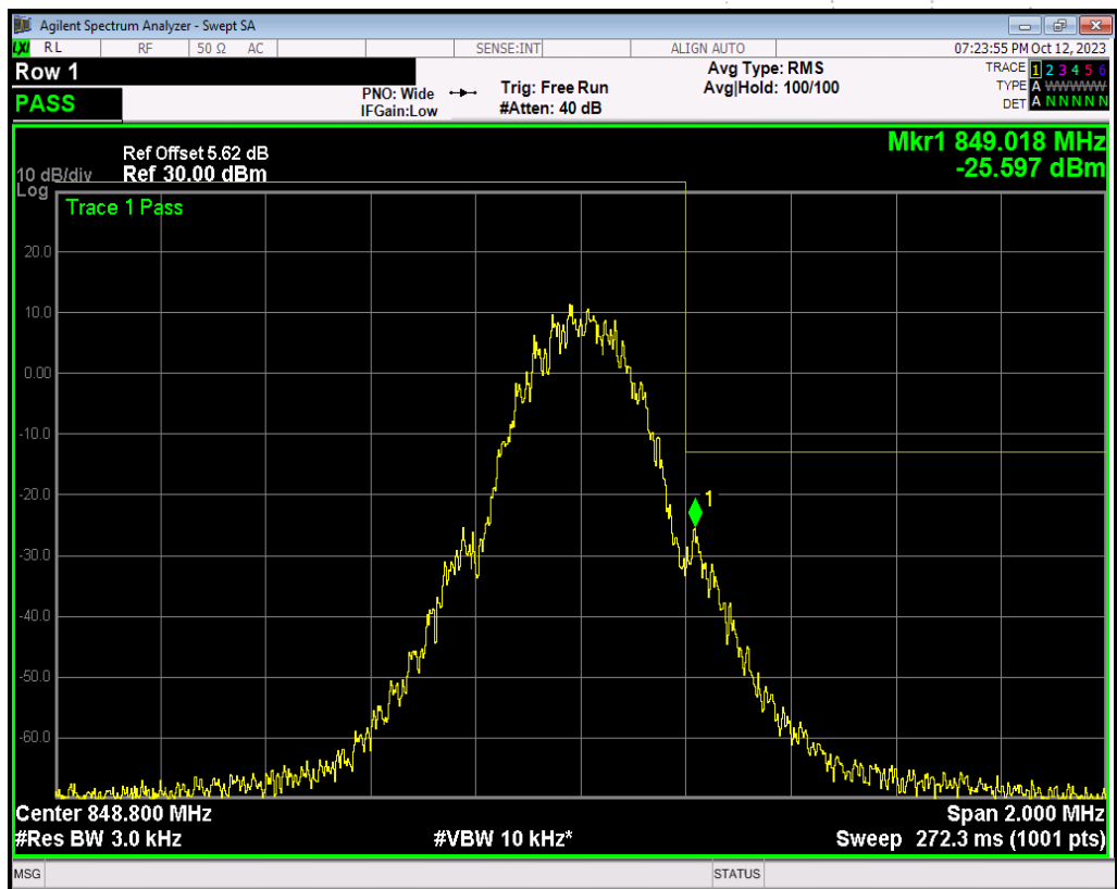
GSM850 Channel=251
