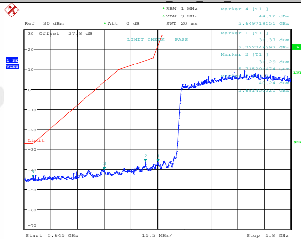
11AX80MIMO Ant2 Low 5775
