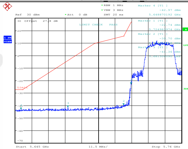
11AX20MIMO Ant2 Low 5745
