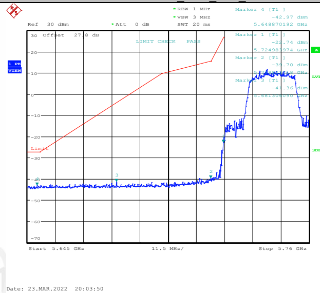
11AX20MIMO Ant2 Low 5745
