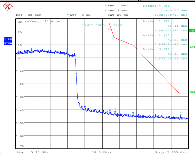
11AX80MIMO Ant1 High 5775
