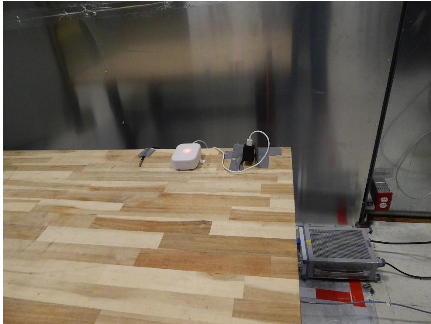
Figure 1.2-1: Conducted emissions
