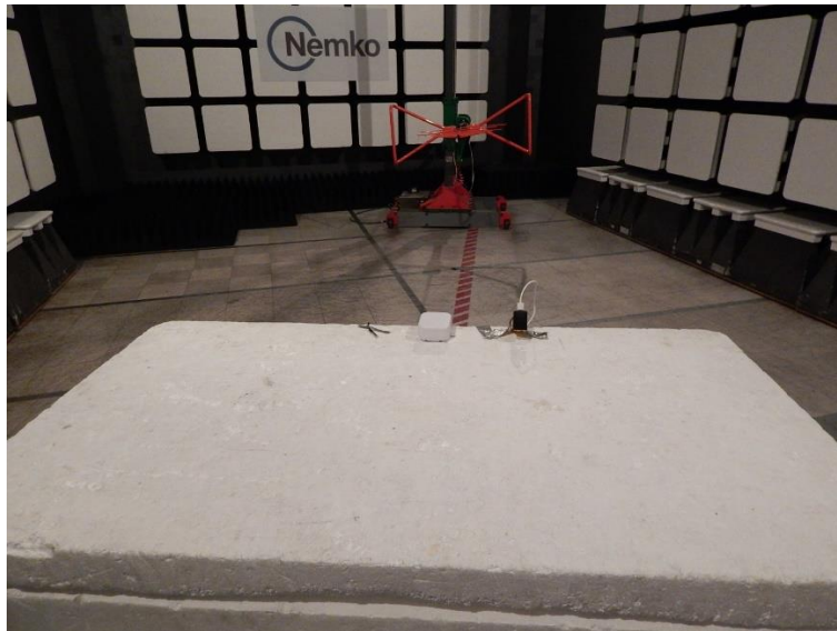
Figure 1.1-1: Radiated emissions 30 to 1000 MHz
