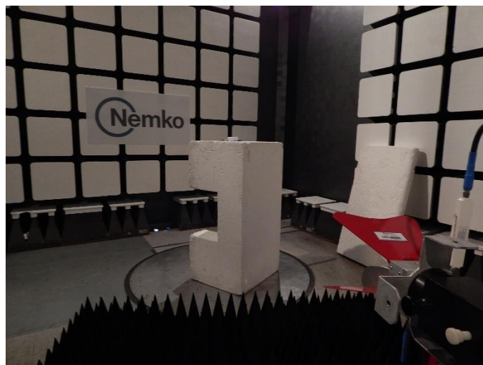
Figure 1.1-2: Radiated emissions above 1 GHz
