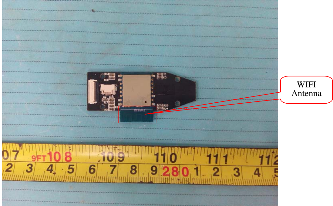
EUT – Main Board 2 Bottom View
