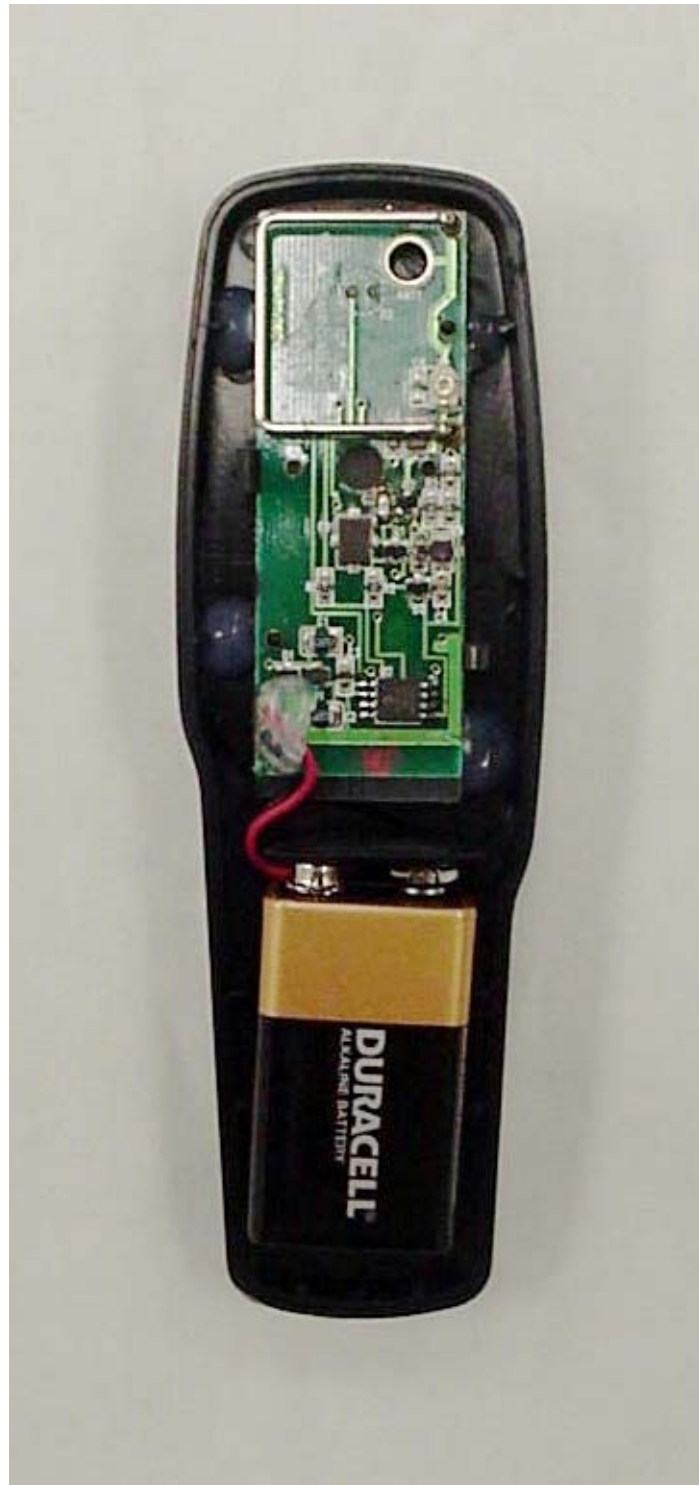
Photo 3. Internal View, Cover Removed
