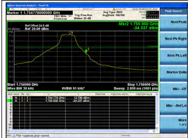
Band4 / 1.4MHz / High CH / QPSK / 1 RB
