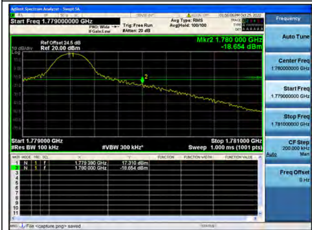
Band66 / 10MHz / High CH / QPSK / 1 RB
