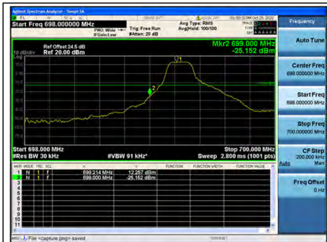
Band12 / 3MHz / Low CH / QPSK / 1 RB
