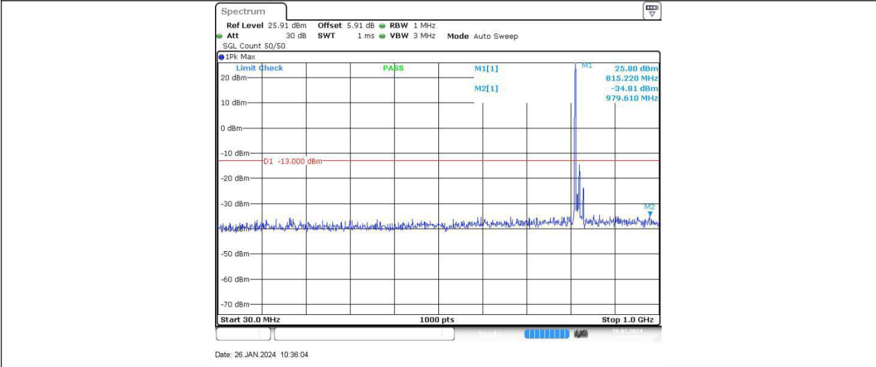
Band26-10MHz-16QAM-26740-1RB#0-Range1:30~1000MHz
