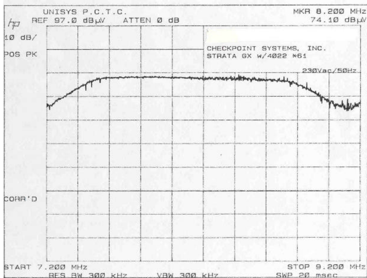
Photo 6 – Bandwidth Plot
