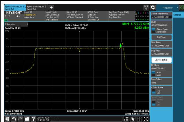
Channel 151 (5755MHz)
