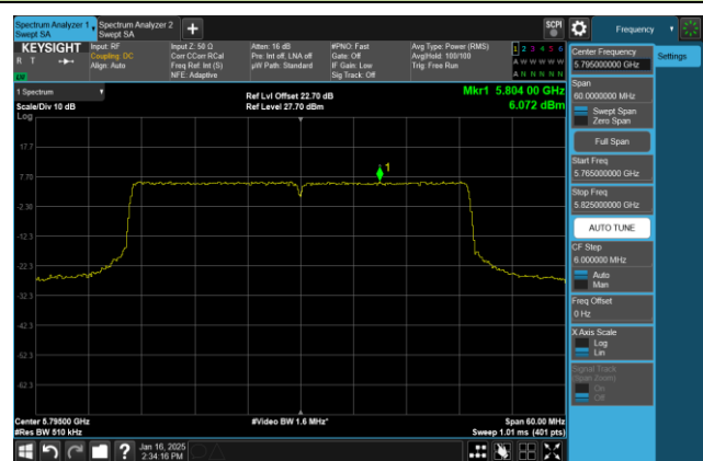
Channel 159 (5795MHz)
