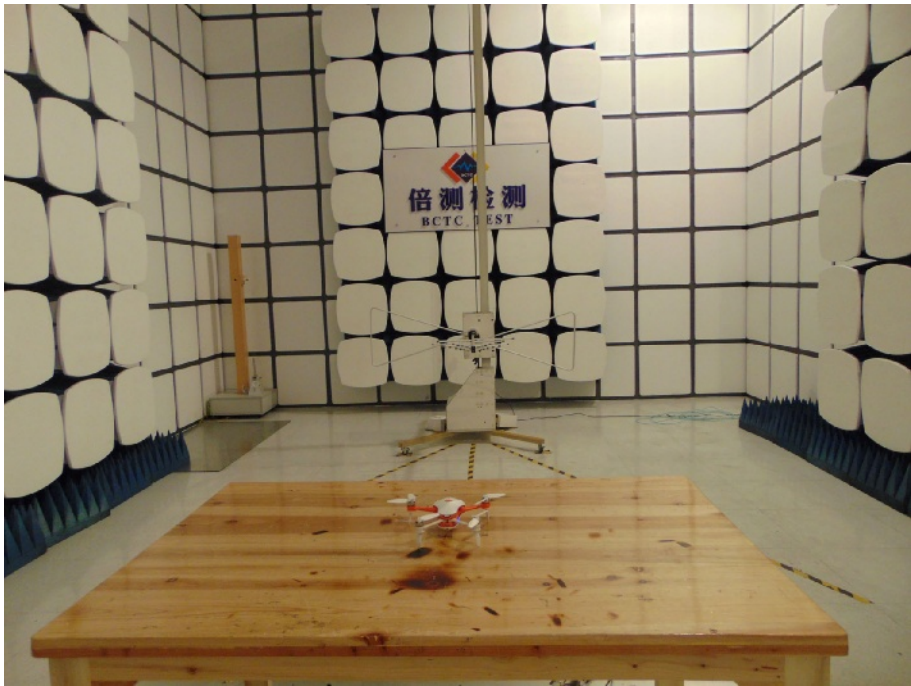
Radiated Emission
