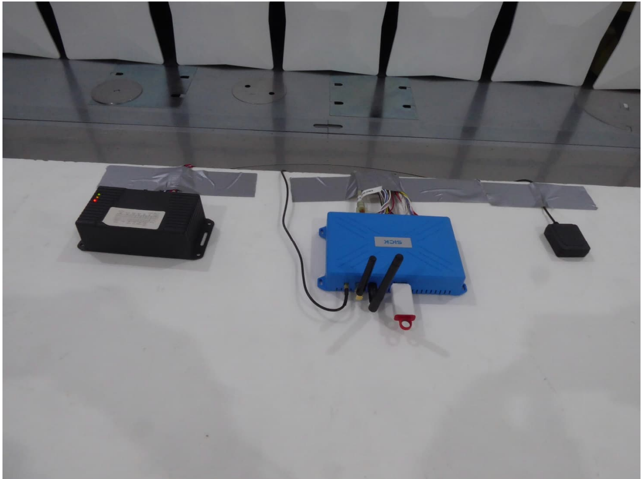
Test setup semi anechoic chamber M276 30 MHz – 14 GHz
