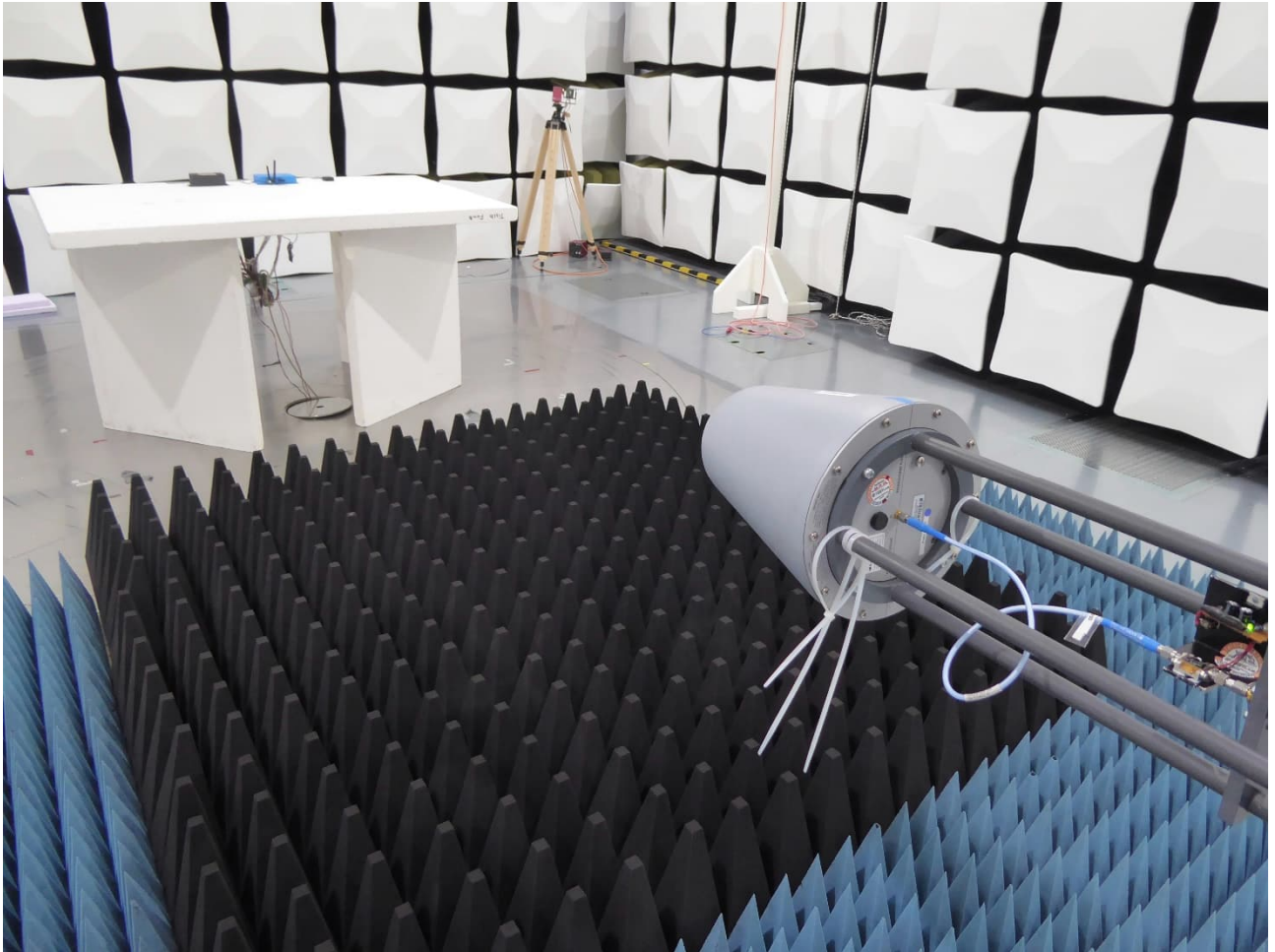
Test setup semi anechoic chamber M276, 1 GHz – 14 GHz
