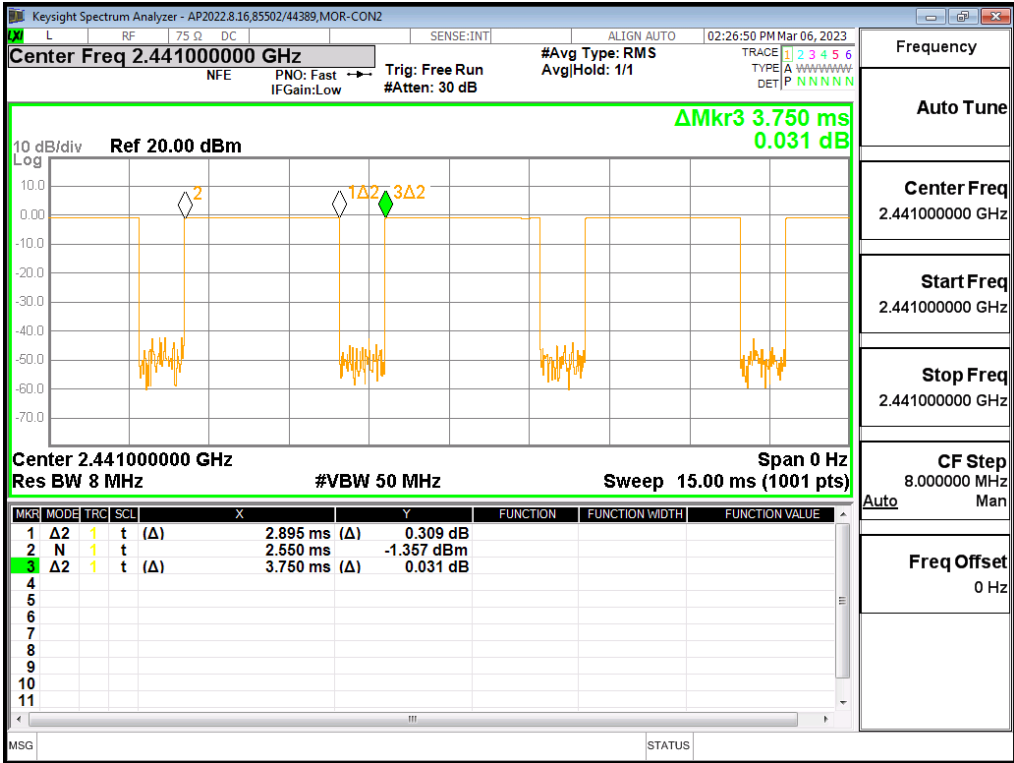
Plot 1: Bluetooth GFSK
