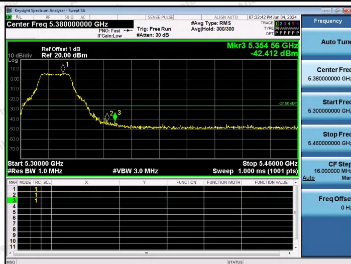
11AC20SISO-Ant1-5320-PASS
