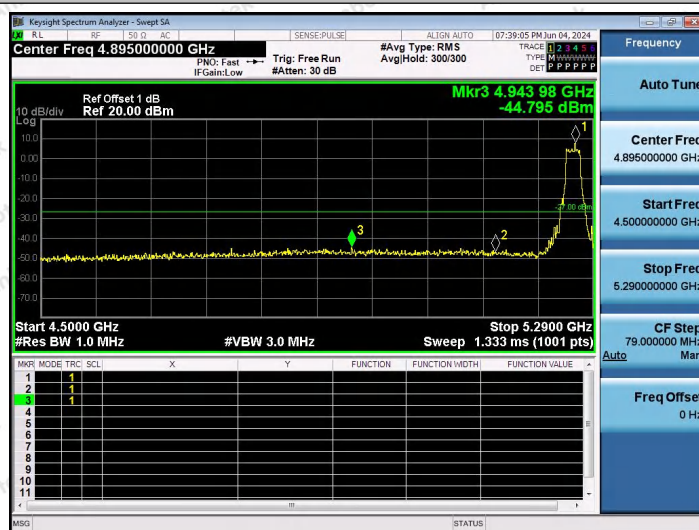
11AX20SISO-Ant1-5260-PASS
