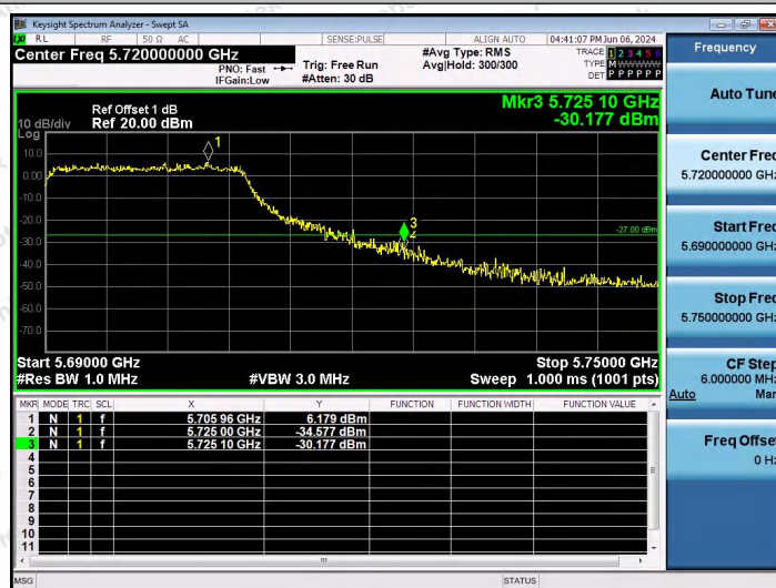
11AX20SISO-Ant1-5700-PASS
