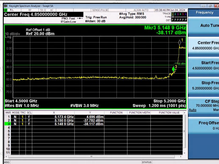
11AX40SISO-Ant1-5190-PASS
