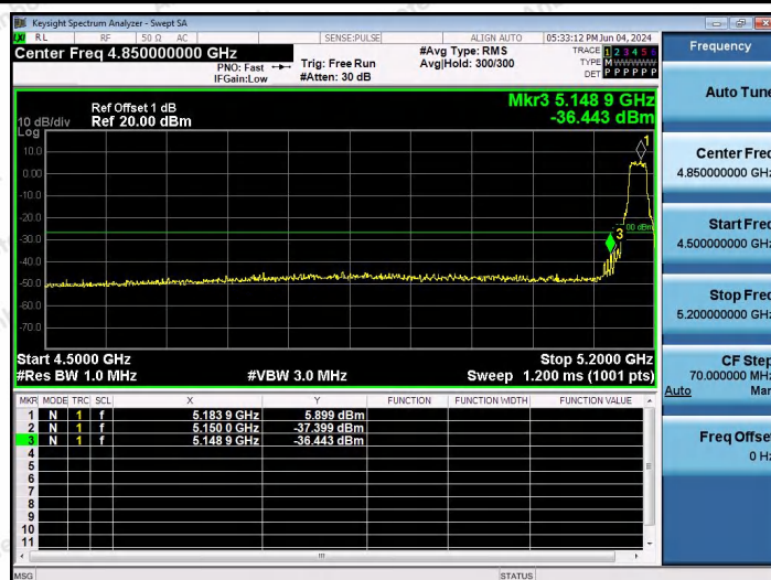
11AX20SISO-Ant1-5180-PASS
