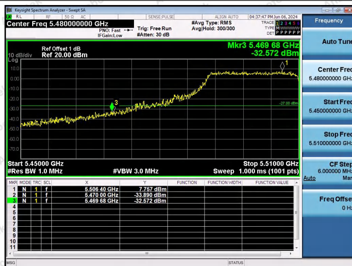
11AX20SISO-Ant1-5500-PASS
