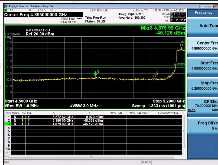
11AX40SISO-Ant1-5270-PASS
