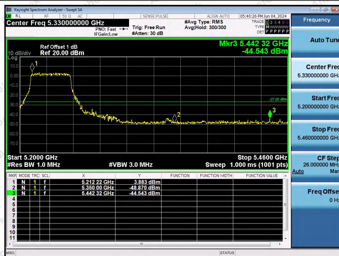
11AX40SISO-Ant1-5230-PASS
