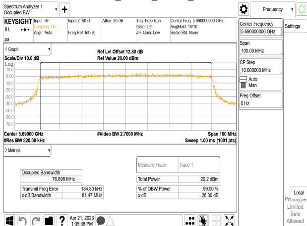
802.11ax_80MHz_Chain0_5690MHz
