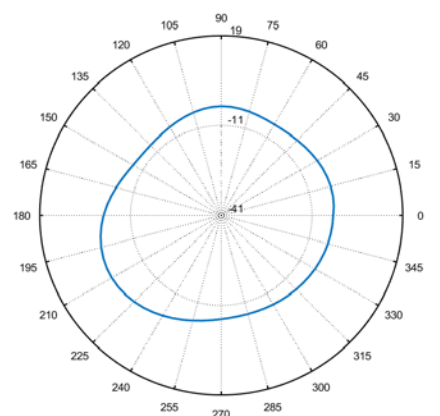
Total_Polar_E2_2.5GHz
