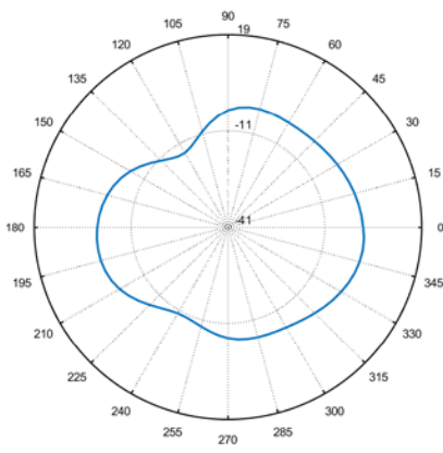
Total_Polar_H_2.5GHz
