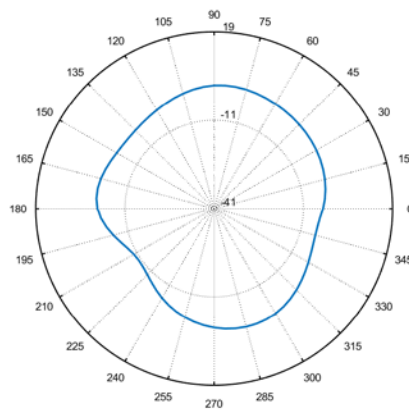
Total_Polar_E1_2.5GHz
