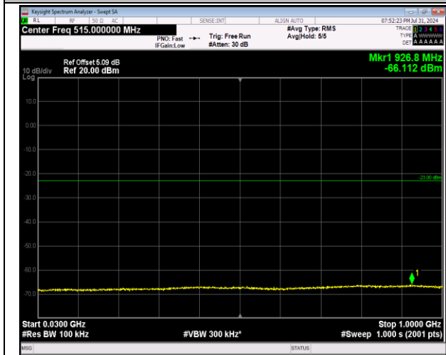
2-2-20MHz-20MHz-64QAM-64QAM-18801-18999-100RB #0-100RB#0-30~1000MHz-PASS
