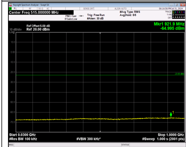
2-2-5MHz-20MHz-64QAM-64QAM-18983-19100-1RB#0-0 ORB#0-30~1000MHz-PASS
