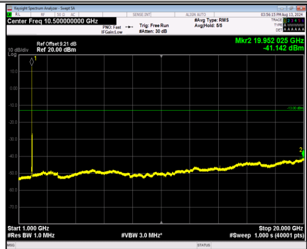
2-2-20MHz-20MHz-16QAM-16QAM-18902-19100-1RB#0-1 RB#99-1000~20000MHz-PASS
