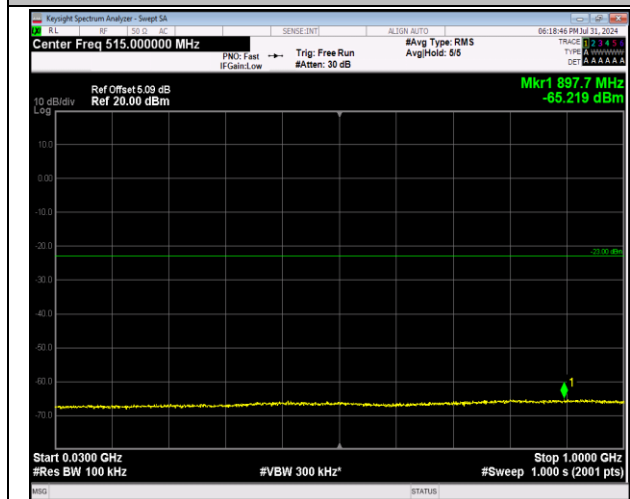
2-2-5MHz-20MHz-64QAM-64QAM-18983-19100-25RB#0-100RB#0-30~1000MHz-PASS
