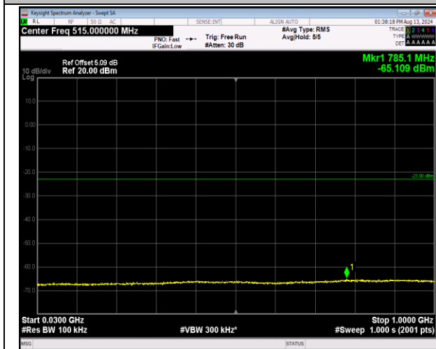
2-2-5MHz-20MHz-QPSK-QPSK-18983-19100-1RB#24-0 RB#0-30~1000MHz-PASS
