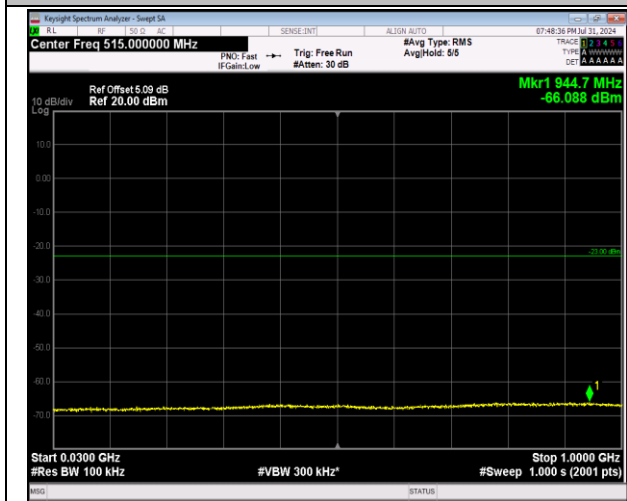
2-2-20MHz-20MHz-64QAM-64QAM-18700-18898-1RB#9 9-0RB#0-30~1000MHz-PASS
