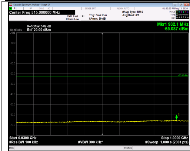
2-2-5MHz-20MHz-16QAM-16QAM-18808-18925-1RB#24 -ORB#0-30~1000MHz-PASS
