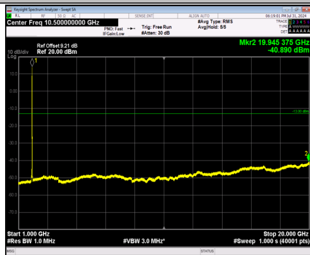
2-2-5MHz-20MHz-64QAM-64QAM-18983-19100-25RB#0-100RB#0-1000~20000MHz-PASS
