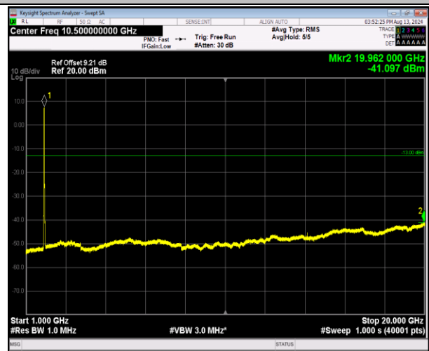
2-2-20MHz-20MHz-16QAM-16QAM-18801-18999-100RB#0 -100RB#0-1000~20000MHz-PASS
