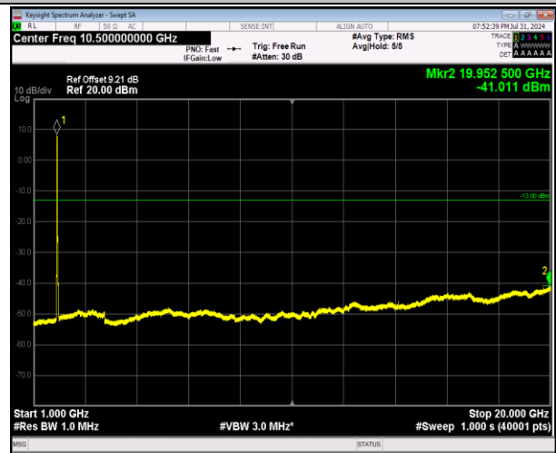
2-2-20MHz-20MHz-64QAM-64QAM-18801-18999-100RB#0 -100RB#0-1000~20000MHz-PASS
