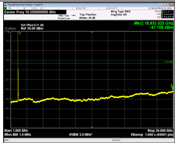
2-2-20MHz-20MHz-64QAM-64QAM-18801-18999-1RB#0-0 RB#0-1000~20000MHz-PASS
