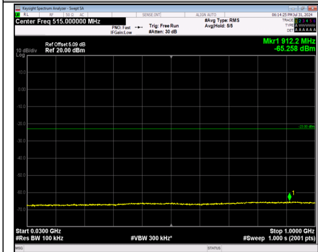
2-2-5MHz-20MHz-64QAM-64QAM-18808-18925-1RB#0-0 ORB#0-30~1000MHz-PASS
