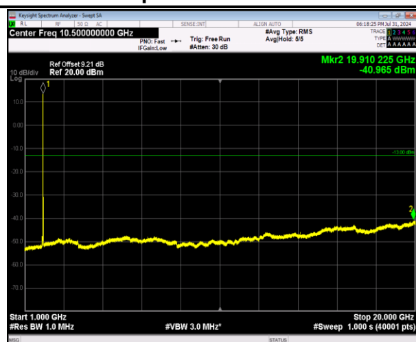
2-2-5MHz-20MHz-64QAM-64QAM-18983-19100-1RB#0-1RB#99-1000~20000MHz-PASS
