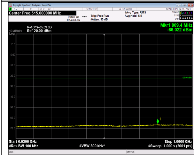
2-2-20MHz-20MHz-64QAM-64QAM-18801-18999-1RB#0 -ORB#0-30~1000MHz-PASS
