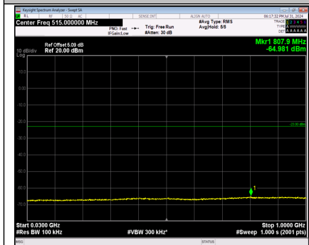
2-2-5MHz-20MHz-64QAM-64QAM-18983-19100-1RB#24-0RB#0-30~1000MHz-PASS
