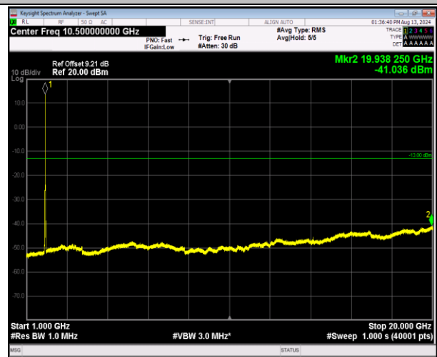
2-2-5MHz-20MHz-16QAM-16QAM-18808-18925-25RB#0-1 00RB#0-1000~20000MHz-PASS
