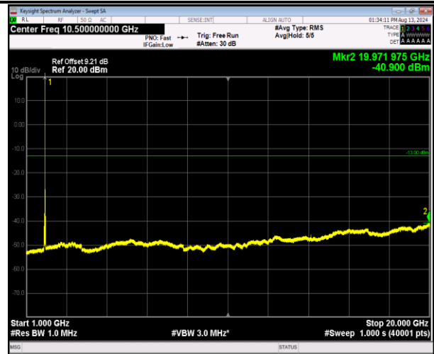
2-2-5MHz-20MHz-16QAM-16QAM-18808-18925-1RB#24-0 RB#0-1000~20000MHz-PASS
