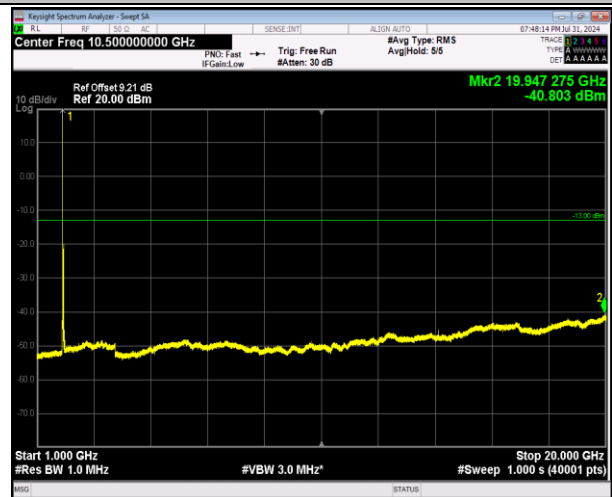
2-2-20MHz-20MHz-64QAM-64QAM-18700-18898-1RB#0-0 RB#0-1000~20000MHz-PASS
