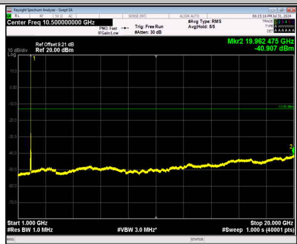
2-2-5MHz-20MHz-64QAM-64QAM-18808-18925-1RB#24-0RB#0-1000~20000MHz-PASS
