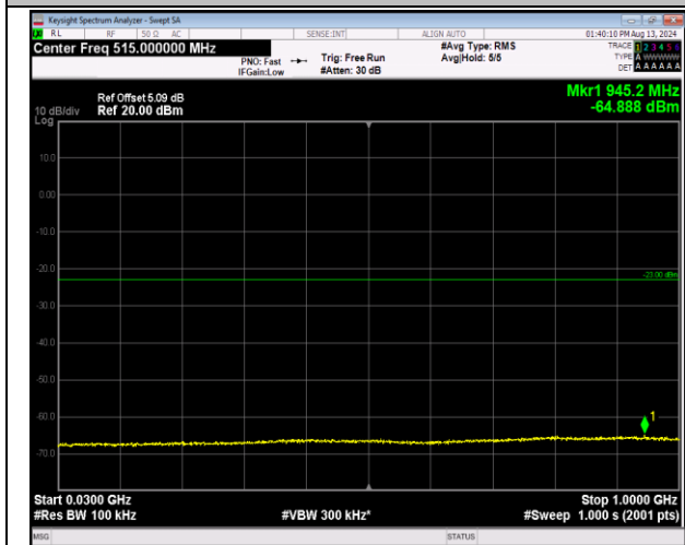
2-2-5MHz-20MHz-16QAM-16QAM-18983-19100-1RB#0-0 1RB#99-30~1000MHz-PASS
