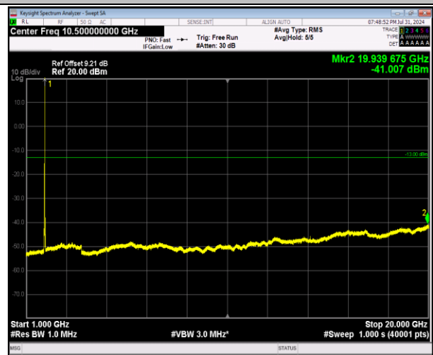
2-2-20MHz-20MHz-64QAM-64QAM-18700-18898-1RB#99- 0RB#0-1000~20000MHz-PASS
