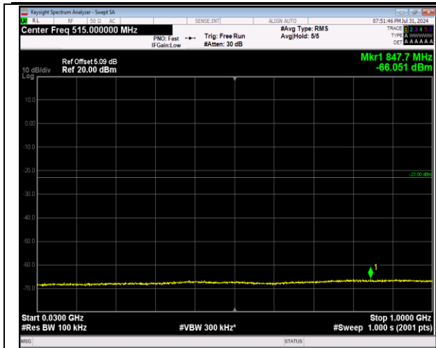
2-2-20MHz-20MHz-64QAM-64QAM-18801-18999-1RB#0 -1RB#99-30~1000MHz-PASS
