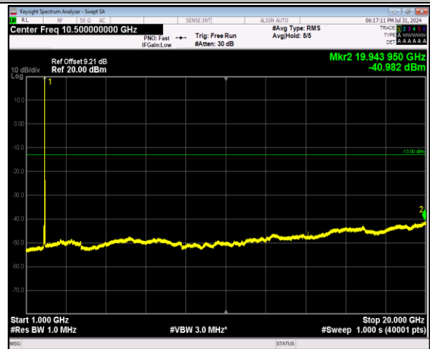
2-2-5MHz-20MHz-64QAM-64QAM-18983-19100-1RB#0-0R B#0-1000~20000MHz-PASS
