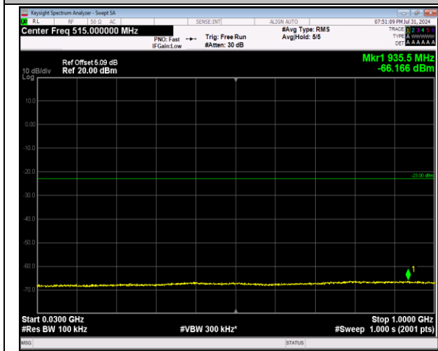
2-2-20MHz-20MHz-64QAM-64QAM-18801-18999-1RB#9 9-0RB#0-30~1000MHz-PASS
