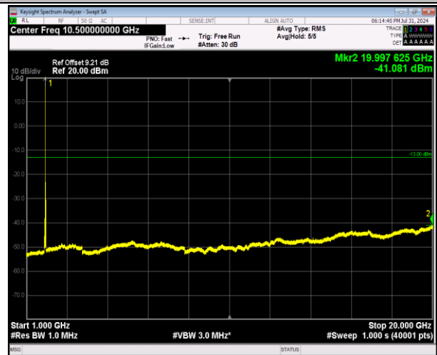
2-2-5MHz-20MHz-64QAM-64QAM-18808-18925-1RB#0-0R B#0-1000~20000MHz-PASS
