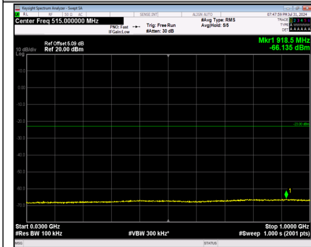
2-2-20MHz-20MHz-64QAM-64QAM-18700-18898-1RB#0 -ORB#0-30~1000MHz-PASS
