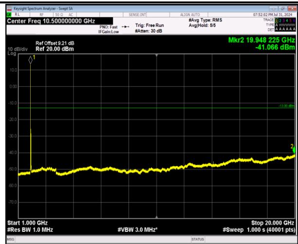
2-2-20MHz-20MHz-64QAM-64QAM-18801-18999-1RB#0-1 RB#99-1000~20000MHz-PASS
