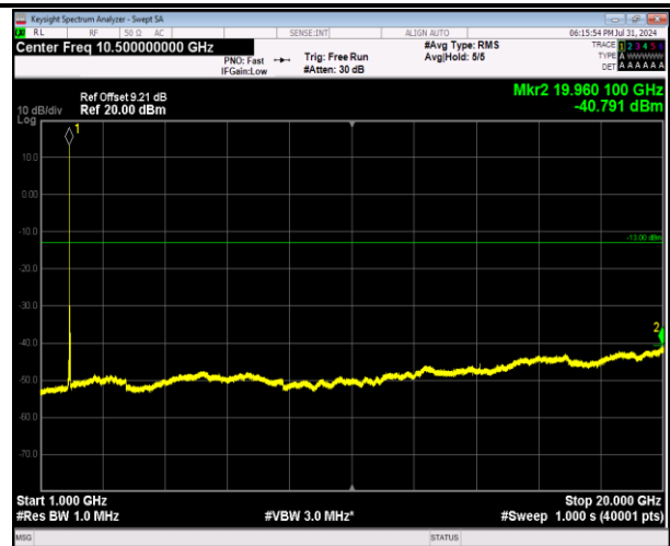
2-2-5MHz-20MHz-64QAM-64QAM-18808-18925-1RB#0-1RB#99-1000~20000MHz-PASS
