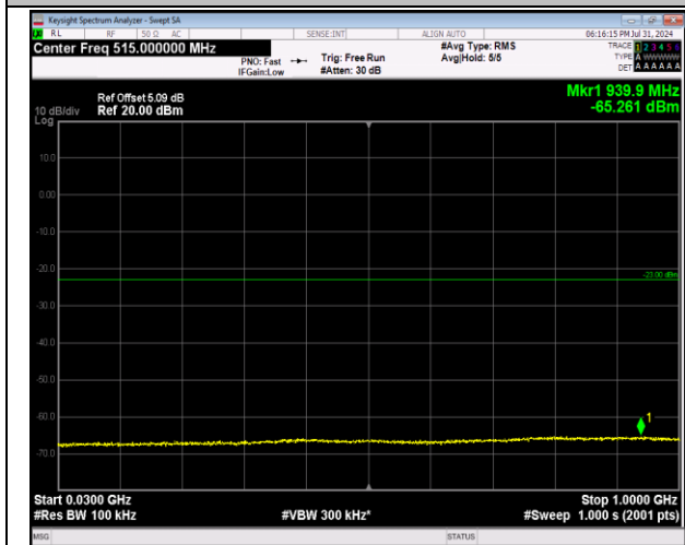
2-2-5MHz-20MHz-64QAM-64QAM-18808-18925-25RB#0-100RB#0-30~1000MHz-PASS
