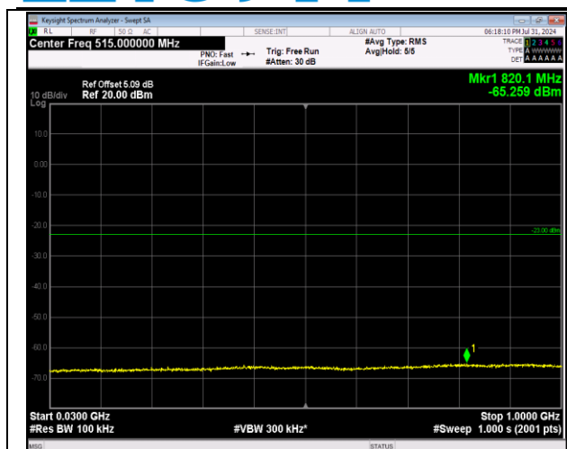
2-2-5MHz-20MHz-64QAM-64QAM-18983-19100-1RB#0-1RB#99-30~1000MHz-PASS
