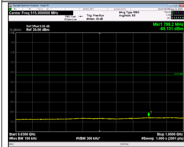
2-2-20MHz-20MHz-16QAM-16QAM-18700-18898-100RB #0-100RB#0-30~1000MHz-PASS
