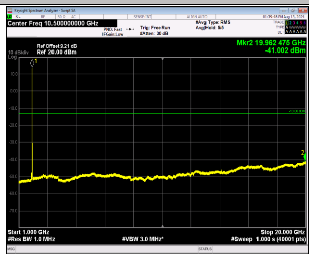
2-2-5MHz-20MHz-QPSK-QPSK-18983-19100-1RB#0-1RB# 99-1000~20000MHz-PASS
