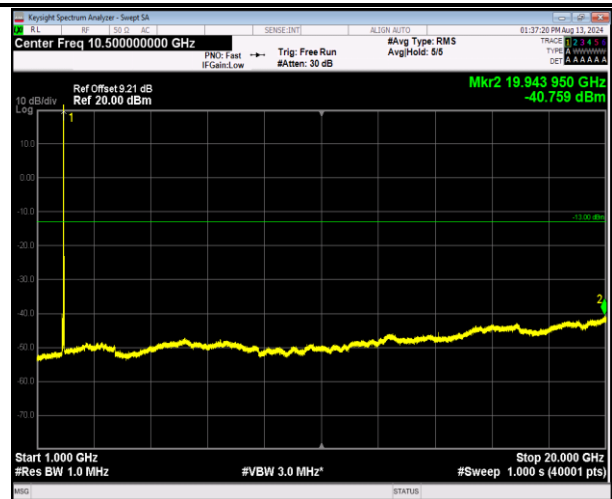
2-2-5MHz-20MHz-QPSK-QPSK-18983-19100-1RB#0-0RB# 0-1000~20000MHz-PASS
