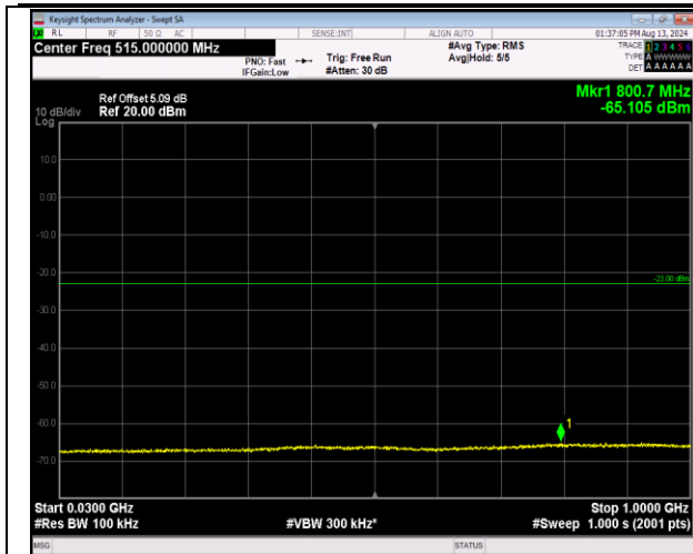
2-2-5MHz-20MHz-QPSK-QPSK-18983-19100-1RB#0-0R B#0-30~1000MHz-PASS
