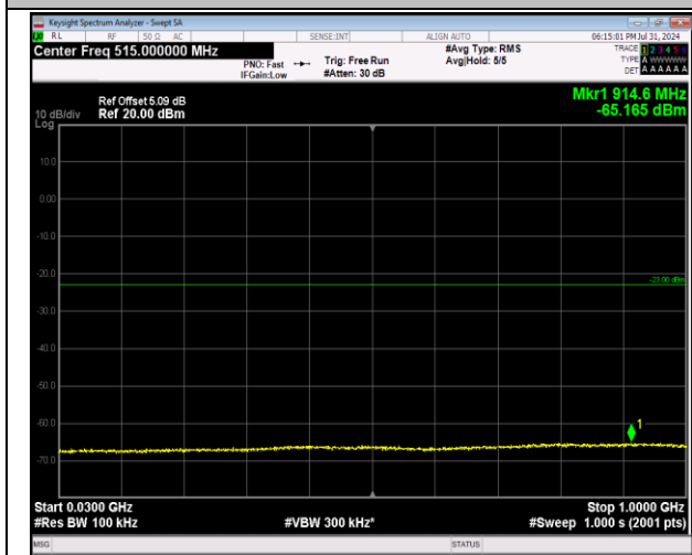
2-2-5MHz-20MHz-64QAM-64QAM-18808-18925-1RB#24-0RB#0-30~1000MHz-PASS
