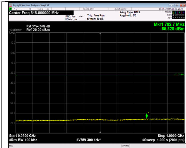
2-2-5MHz-20MHz-64QAM-64QAM-18808-18925-1RB#0-1RB#99-30~1000MHz-PASS
