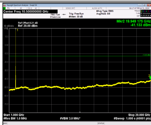
2-2-5MHz-20MHz-64QAM-64QAM-18983-19100-1RB#24-0RB#0-1000~20000MHz-PASS
