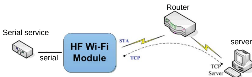
Figure 10. HF-LPT230 STA Network Structure
