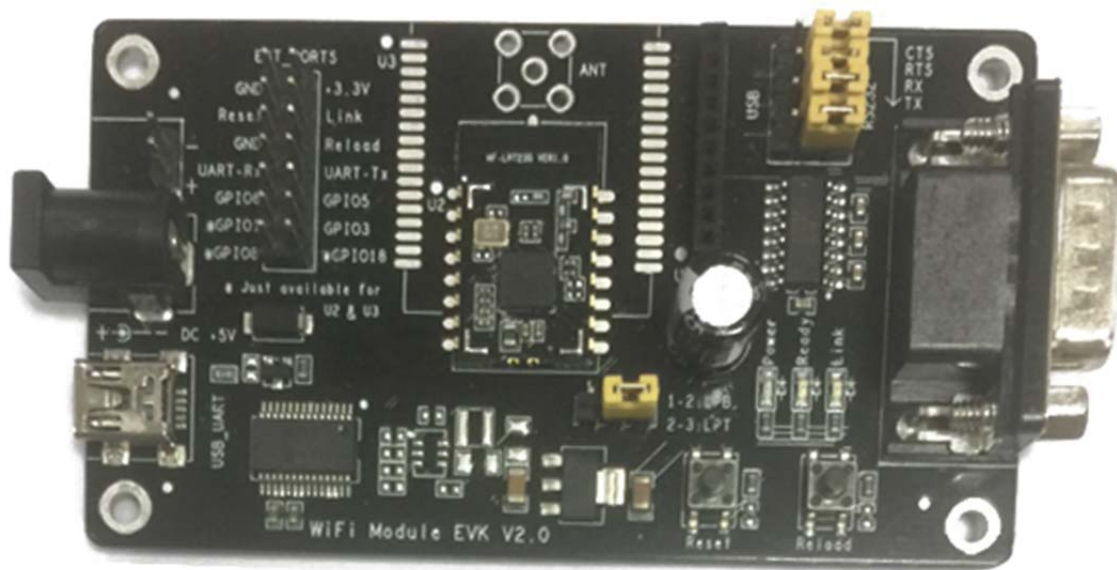
Figure 5. LPT120/LPT220 EVK
