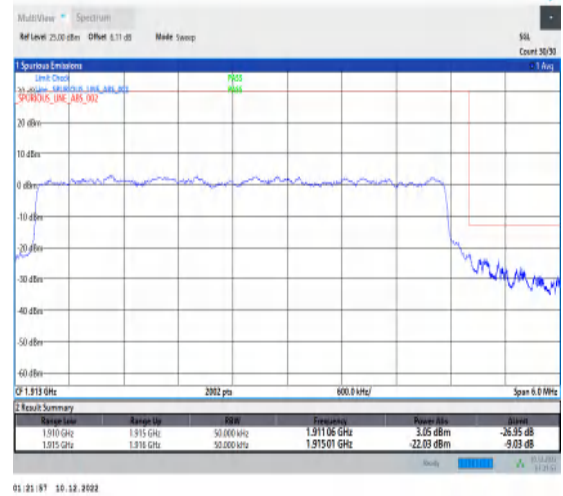
1-N25-15-5-H-3-DFT-PI2BPSK-Outer_Full-25@0-Ant1-1-seegraph-PASS-see graph
