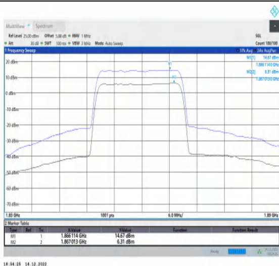
1-N25-15-20-L-1-DFT-256QAM-Outer_Full-100@0-A nt1-8.36-100%-0.00-8.36-PASS-≤13
