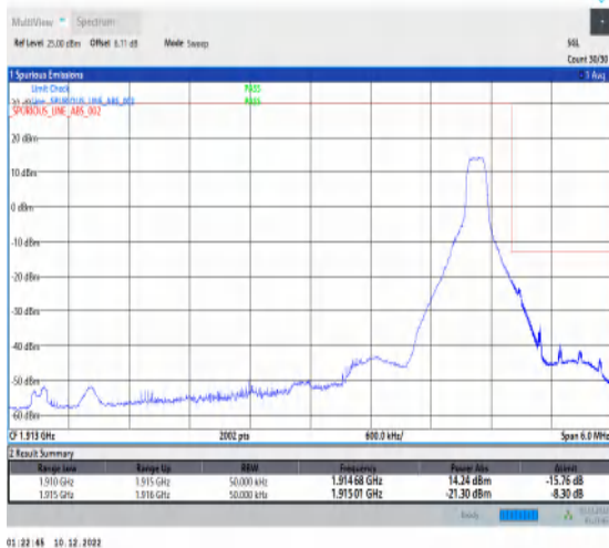
1-N25-15-5-H-5-CP-QPSK-Edge_1RB_Right-1@24-Ant1-1-seegraph-PASS-see graph
