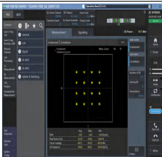
1-N25--15-40-M-7-CP-16QAM-Outer_Full-216@0-Ant1-see graph-PASS
