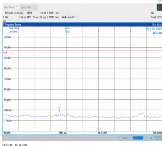
1-N25-15-20-L-1-DFT-PI2BPSK-Inner_1RB_Left-1 @1-0.009-0.15-Ant1-0.06--101.15--43-PASS
