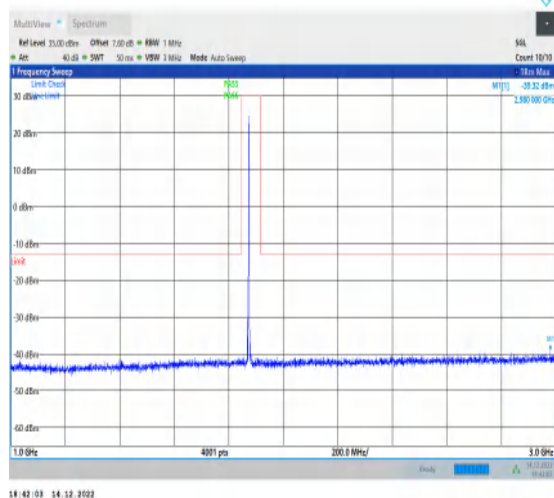
1-N25-15-20-M-1-DFT-PI2BPSK-Inner_1RB_Left-1@ 1-1000-3000-Ant1-2980.00--39.32--13-PASS
