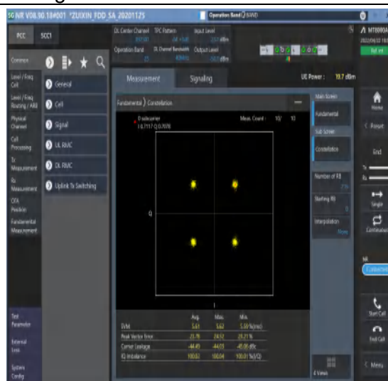
1-N25--15-40-M-6-CP-QPSK-Outer_Full-216@0-Ant1-see graph-PASS
