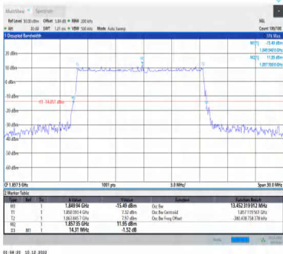
1-N25-15-15-L-5-DFT-256QAM-Outer_Full-75@0-Ant 1-13.452-14.310≤15-PASS
