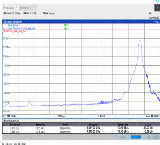
1-N25-15-10-H-5-CP-QPSK-Edge_1RB_Right-1@51-Ant1-1-seegraph-PASS-see graph
