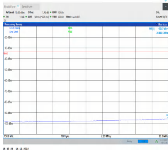
1-N25-15-20-H-1-DFT-PI2BPSK-Inner_1RB_Left-1@ 1-0.15-30-Ant1-29.88--95.87--33-PASS
