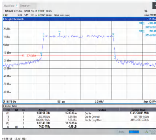
1-N25-15-15-L-4-DFT-64QAM-Outer_Full-75@0-Ant 1-13.453-14.250≤15-PASS
