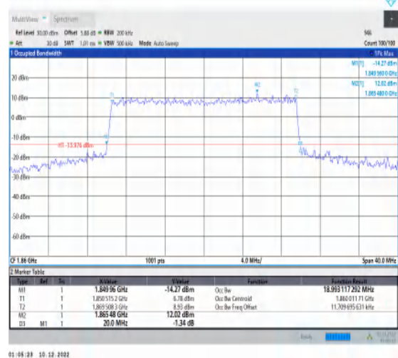
1-N25-15-20-L-7-CP-16QAM-Outer_Full-106@0-Ant 1-18.993-20.000-≤20-PASS
