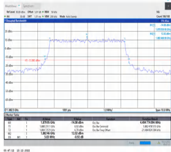
1-N25-15-5-M-3-DFT-16QAM-Outer_Full-25@0-Ant1 -4.495-5.030-≤5-PASS
