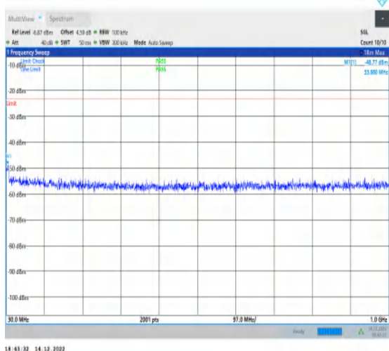
1-N25-15-20-H-1-DFT-PI2BPSK-Inner_1RB_Left-1 @1-30-1000-Ant1-33.88--48.77--23-PASS
