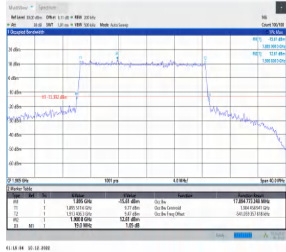
1-N25-15-20-H-3-DFT-16QAM-Outer_Full-100@0-A nt1-17.895-19.000-<20-PASS
