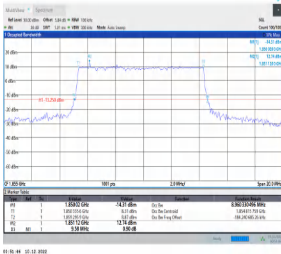
1-N25-15-10-L-4-DFT-64QAM-Outer_Full-50@0-Ant 1-8.96-9.580-≤10-PASS
