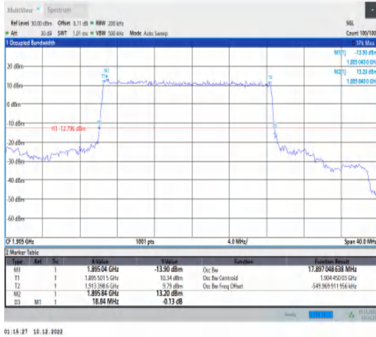
1-N25-15-20-H-2-DFT-PI2BPSK-Outer_Full-100@0-A Ant1-17.897-18.840-<20-PASS
