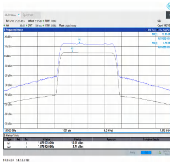
1-N25-15-20-M-2-CP-256QAM-Outer_Full-106@0-A nt1-9.17-100%-0.00-9.17-PASS-≤13
