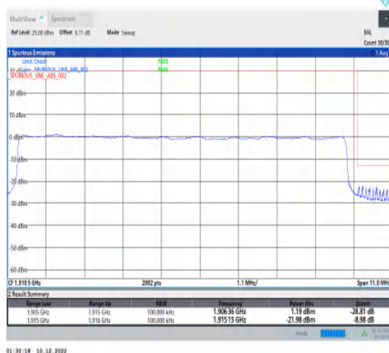
1-N25-15-10-H-6-CP-QPSK-Outer_Full-52@0-Ant1-1-seegraph-PASS-see graph
