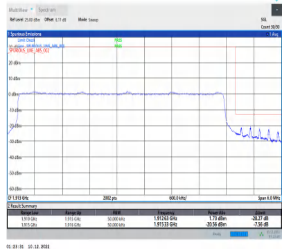
1-N25-15-5-H-6-CP-QPSK-Outer_Full-25@0-Ant1-1-seegraph-PASS-see graph
