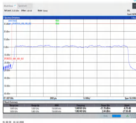
1-N25-15-15-L-3-DFT-PI2BPSK-Outer_Full-75@0-Ant1-1-seegraph-PASS-see graph
