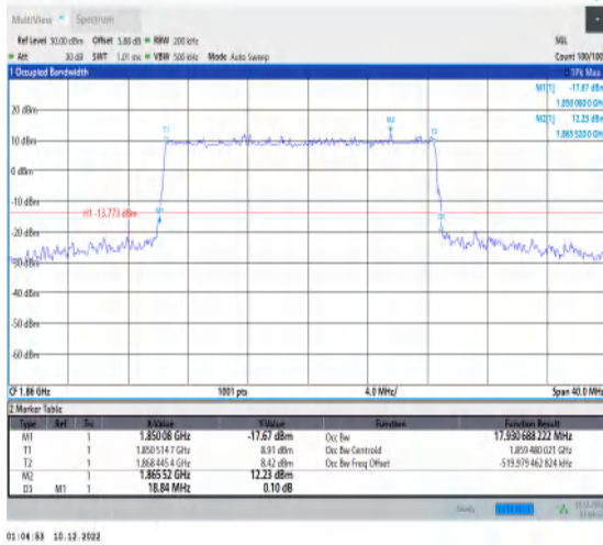
1-N25-15-20-L-4-DFT-64QAM-Outer_Full-100@0-An t1-17.931-18.840-≤20-PASS
