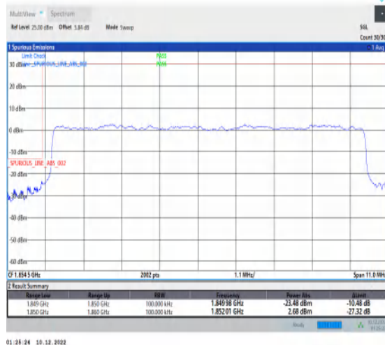
1-N25-15-10-L-3-DFT-PI2BPSK-Outer_Full-50@0-Ant1-1-seegraph-PASS-see graph
