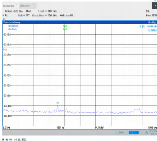
1-N25-15-20-M-1-DFT-PI2BPSK-Inner_1RB_Left-1 @1-0.009-0.15-Ant1-0.06--100.84--43-PASS
