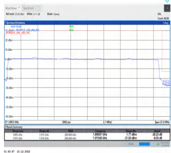
1-N25-15-20-H-6-CP-QPSK-Outer_Full-106@0-Ant1-1-seegraph-PASS-see graph
