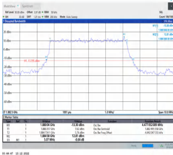
1-N25-15-5-M-2-DFT-P12BPSK-Outer_Full-25@0-An t1-4.477-5.070-≤5-PASS
