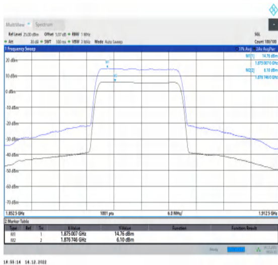
1-N25-15-20-M-1-DFT-256QAM-Outer_Full-100@0-A Ant1-8.66-100%-0.00-8.66-PASS-≤13
