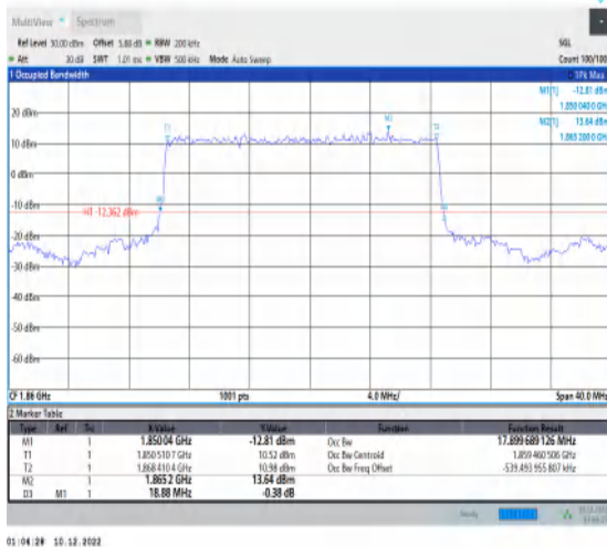
1-N25-15-20-L-2-DFT-PI2BPSK-Outer_Full-100@0-Ant 1-17.9-18.880-≤20-PASS
