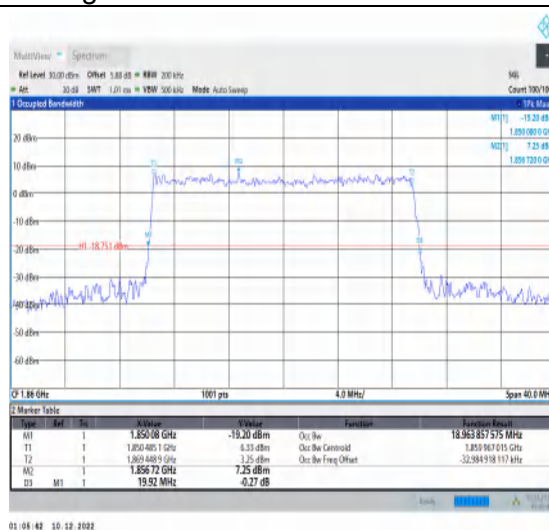
1-N25-15-20-L-9-CP-256QAM-Outer_Full-106@0-An t1-18.964-19.920-≤20-PASS
