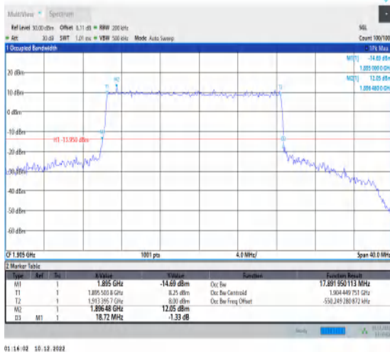
1-N25-15-20-H-4-DFT-64QAM-Outer_Full-100@0-A nt1-17.892-18.720-<20-PASS
