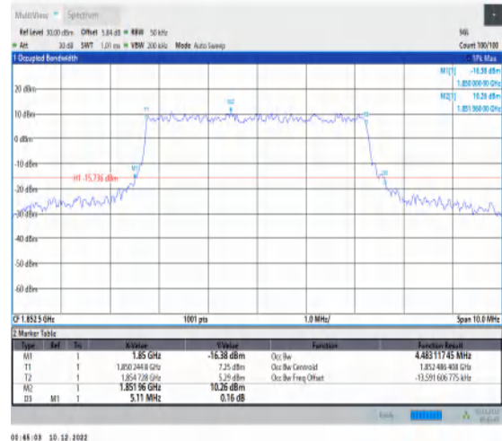
1-N25-15-5-L-4-DFT-64QAM-Outer_Full-25@0-Ant1-4 4.483-5.110-≤5-PASS
