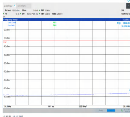
1-N25-15-20-L-1-DFT-PI2BPSK-Inner_1RB_Left-1@ 1-0.15-30-Ant1-29.82--95.86--33-PASS
