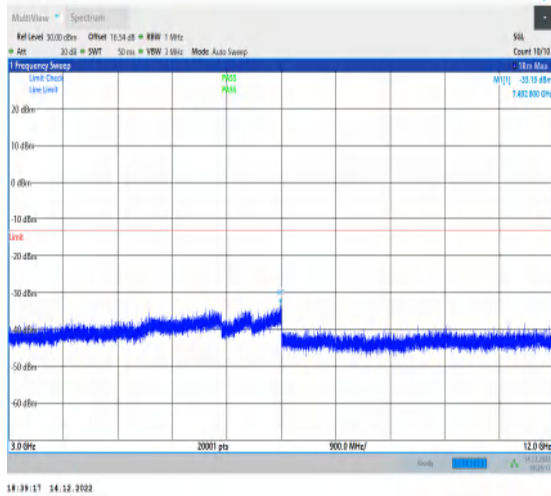
1-N25-15-20-L-1-DFT-PI2BPSK-Inner_1RB_Left-1 @1-3000-12000-Ant1-7492.80--33.19--13-PASS
