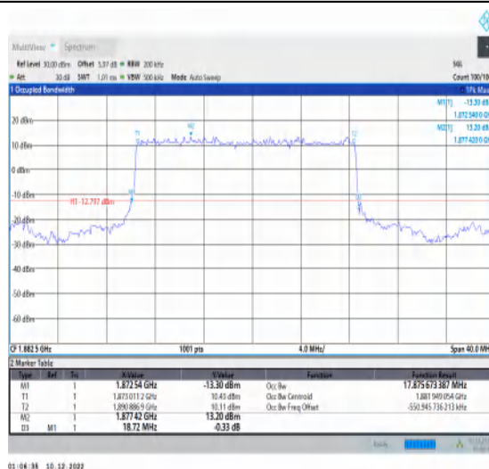
1-N25-15-20-M-2-DFT-PI2BPSK-Outer_Full-100@0-Ant 1-17.876-18.720-≤20-PASS
