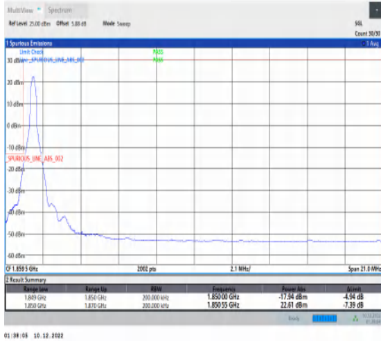
1-N25-15-20-L-1-DFT-PI2BPSK-Edge_1RB_Left-1@0-Ant1-1-seegraph-PASS-see graph
