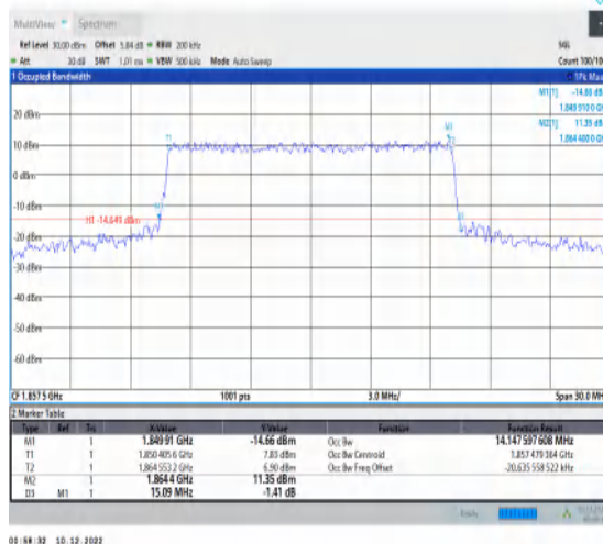
1-N25-15-15-L-6-CP-QPSK-Outer_Full-79@0-Ant1-1 4.148-15.090≤15-PASS
