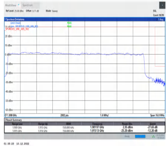
1-N25-15-15-H-3-DFT-PI2BPSK-Outer_Full-75@0-Ant1-1-seegraph-PASS-see graph
