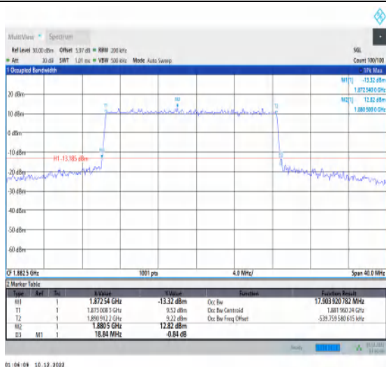
1-N25-15-20-M-1-DFT-QPSK-Outer_Full-100@0-Ant 1-17.904-18.840-≤20-PASS
