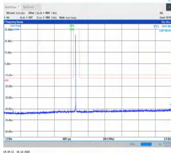
1-N25-15-20-L-1-DFT-PI2BPSK-Inner_1RB_Left-1@ 1-1000-3000-Ant1-2987.50--39.47--13-PASS
