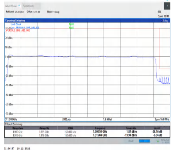
1-N25-15-15-H-6-CP-QPSK-Outer_Full-79@0-Ant1-1-seegraph-PASS-see graph
