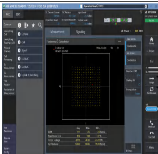
1-N25--15-40-M-5-DFT-256QAM-Outer_Full-216@0-Ant1-see graph-PASS
