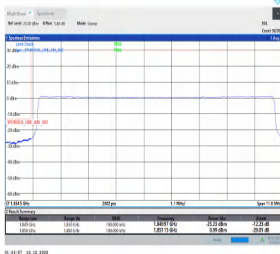
1-N25-15-10-L-6-CP-QPSK-Outer_Full-52@0-Ant1-1-seegraph-PASS-see graph
