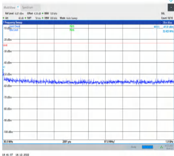
1-N25-15-20-M-1-DFT-PI2BPSK-Inner_1RB_Left-1 @ 1-30-1000-Ant1-32.43--47.31--23-PASS
