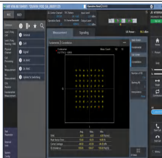
1-N25--15-40-M-8-CP-64QAM-Outer_Full-216@0-Ant1-see graph-PASS
