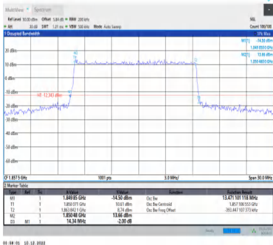
1-N25-15-15-L-3-DFT-16QAM-Outer_Full-75@0-Ant 1-13.471-14.340≤15-PASS
