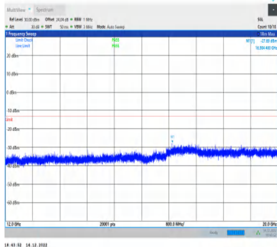
1-N25-15-20-H-1-DFT-PI2BPSK-Inner_1RB_Left-1@ 1-12000-20000-Ant1-16904.40--27.69--13-PASS
