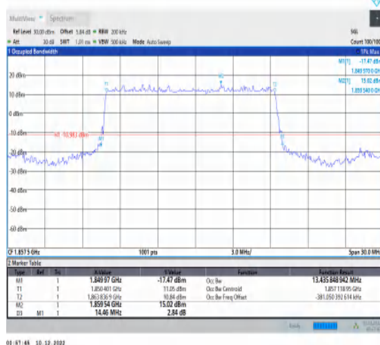
1-N25-15-15-L-2-DFT-PI2BPSK-Outer_Full-75@0-A nt1-13.436-14.460-≤15-PASS
