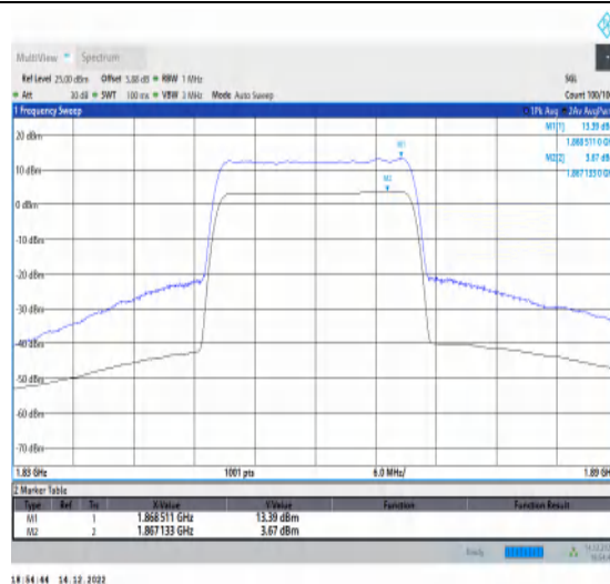
1-N25-15-20-L-2-CP-256QAM-Outer_Full-106@0-A nt1-9.72-100%-0.00-9.72-PASS-≤13
