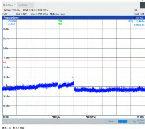
1-N25-15-20-H-1-DFT-PI2BPSK-Inner_1RB_Left-1 @1-3000-12000-Ant1-7459.05--33.46--13-PASS
