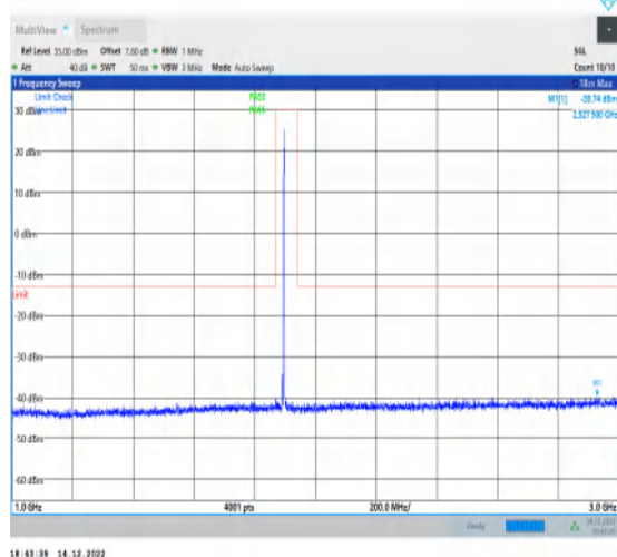
1-N25-15-20-H-1-DFT-PI2BPSK-Inner_1RB_Left-1@ 1-1000-3000-Ant1-2927.50--39.74--13-PASS
