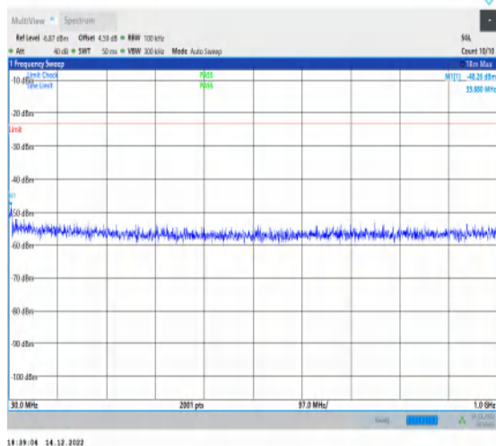
1-N25-15-20-L-1-DFT-PI2BPSK-Inner_1RB_Left-1 @1-30-1000-Ant1-33.88--48.26--23-PASS
