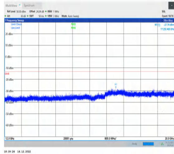
1-N25-15-20-L-1-DFT-PI2BPSK-Inner_1RB_Left-1@ 1-12000-20000-Ant1-17232.40--27.74--13-PASS
