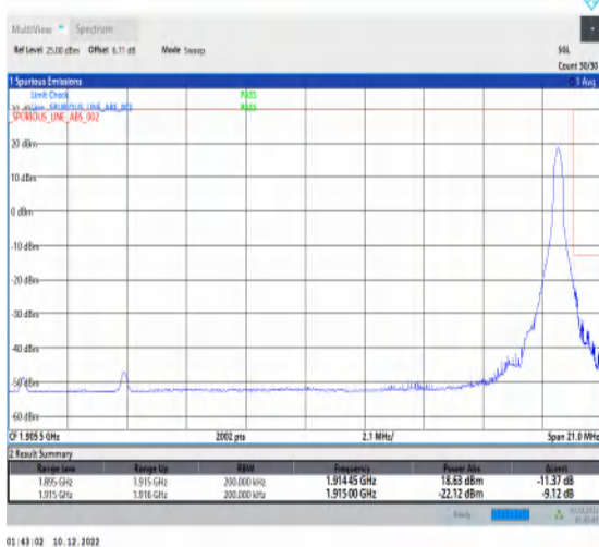
1-N25-15-20-H-5-CP-QPSK-Edge_1RB_Right-1@105-Ant1-1-seegraph-PASS-see graph
