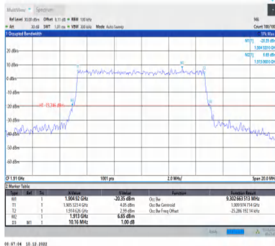
1-N25-15-10-H-9-CP-256QAM-Outer_Full-52@0-Ant 1-9.303-10.160-≤10-PASS
