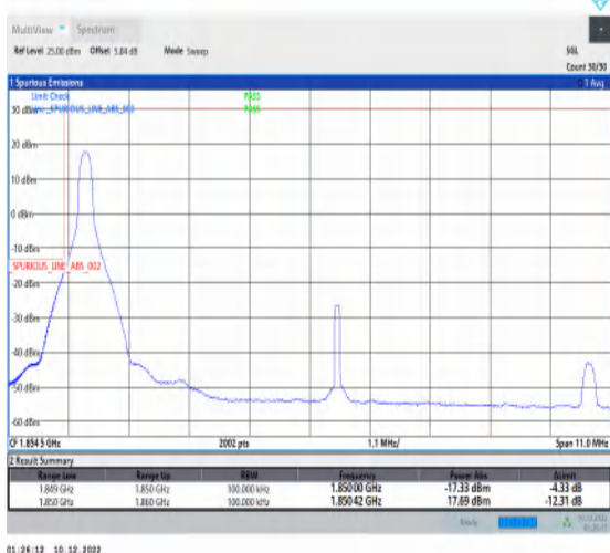
1-N25-15-10-L-4-CP-QPSK-Edge_1RB_Left-1@0-Ant1-1-seegraph-PASS-see graph
