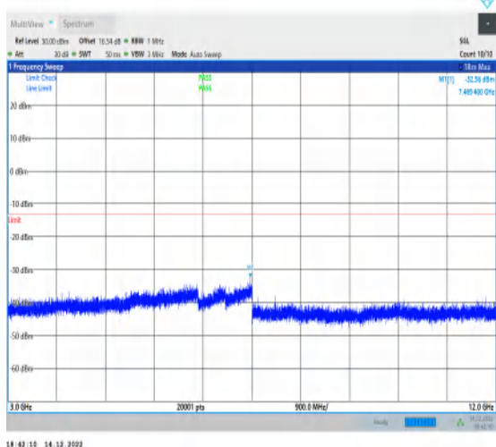
1-N25-15-20-M-1-DFT-PI2BPSK-Inner_1RB_Left-1 @ 1-3000-12000-Ant1-7469.40--32.56--13-PASS
