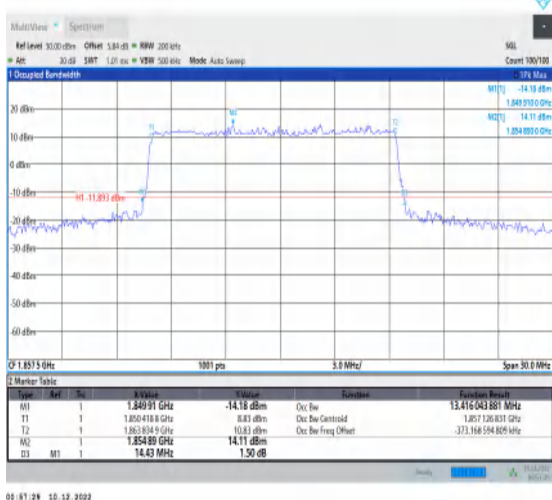
1-N25-15-15-L-1-DFT-QPSK-Outer_Full-75@0-Ant1- 13.416-14.430-≤15-PASS
