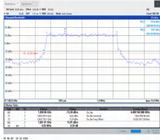
1-N25-15-5-L-2-DFT-PI2BPSK-Outer_Full-25@0-Ant1-4 1-4.49-4.930-≤5-PASS
