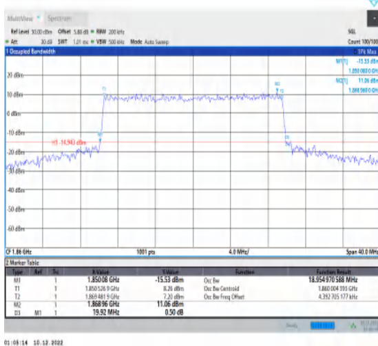
1-N25-15-20-L-6-CP-QPSK-Outer_Full-106@0-Ant1 -18.955-19.920-≤20-PASS
