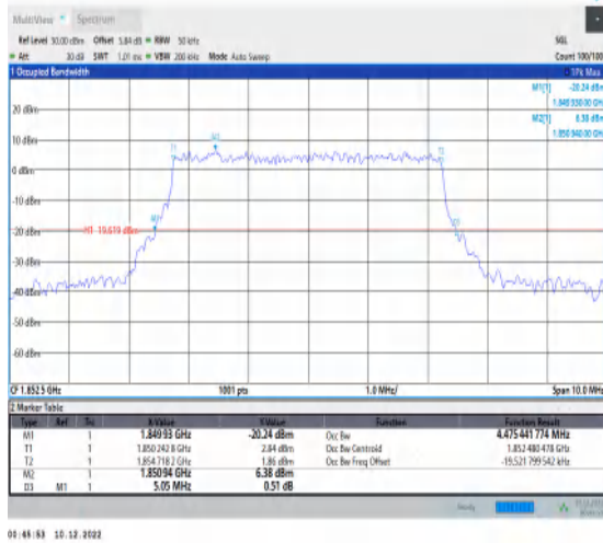
1-N25-15-5-L-9-CP-256QAM-Outer_Full-25@0-Ant1 -4.475-5.050-≤5-PASS
