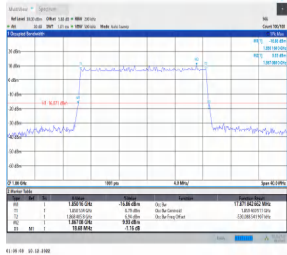
1-N25-15-20-L-5-DFT-256QAM-Outer_Full-100@0-A nt1-17.872-18.680-≤20-PASS
