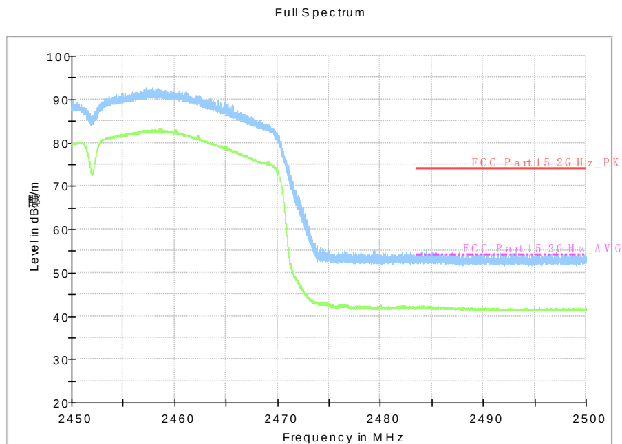
Fig.136 Transmitter Spurious Emission - Radiated (Power): 802.11n-HT40, ch9, 2.45 GHz - 2.50GHz
