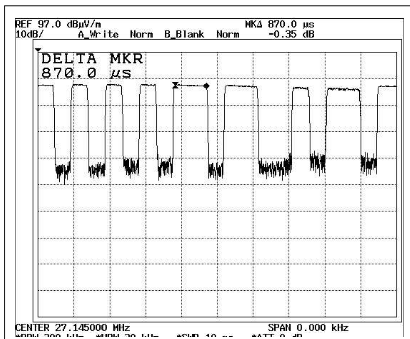
Duty Cycle 2
