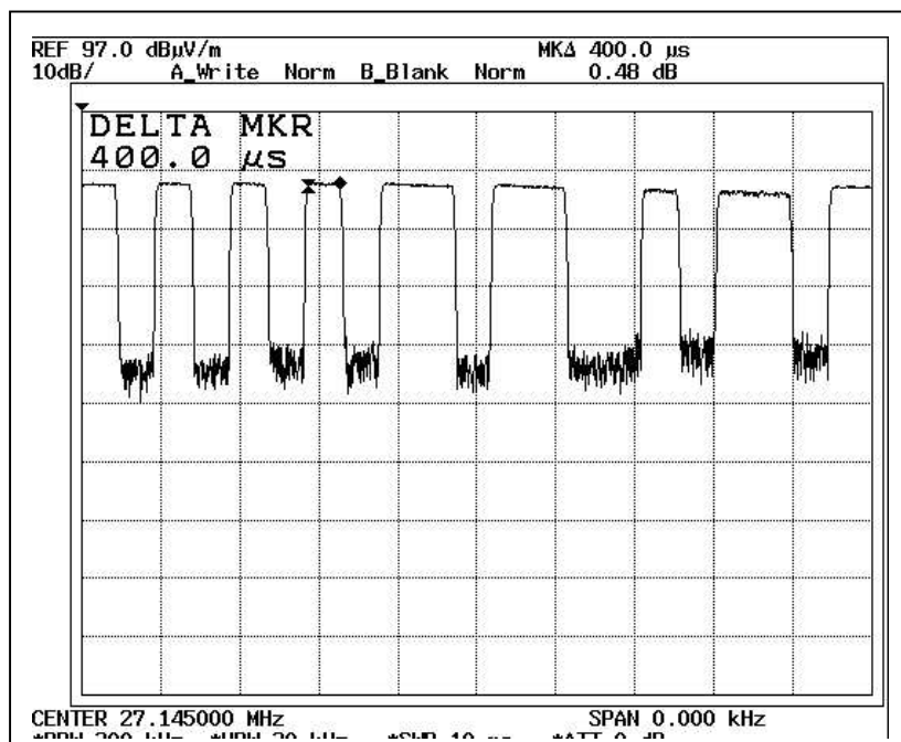
Duty Cycle 3
