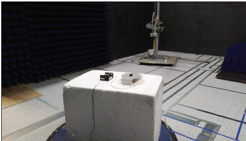
Figure 1: Radiated Emissions Test Setup Photo – 9kHz-30MHz
