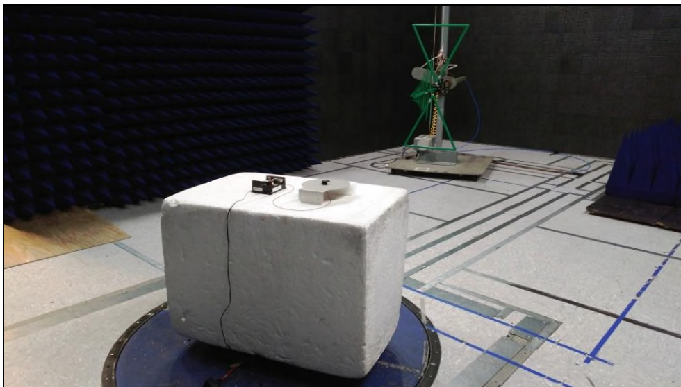
Figure 2: Radiated Emissions Test Setup Photo – 30MHz-1GHz
