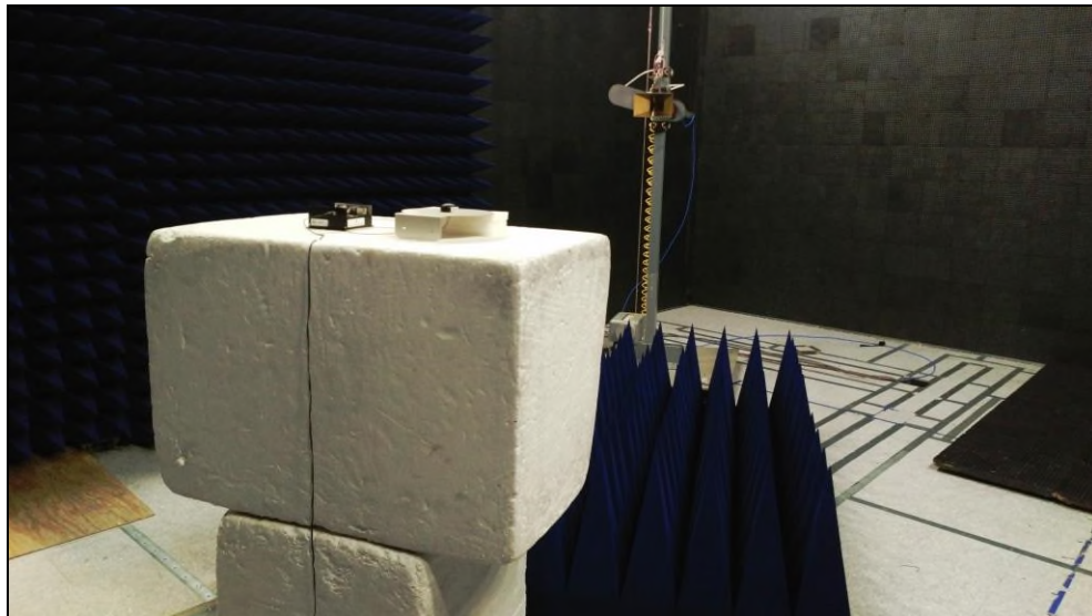
Figure 3: Radiated Emissions Test Setup Photo – Above 1GHz
