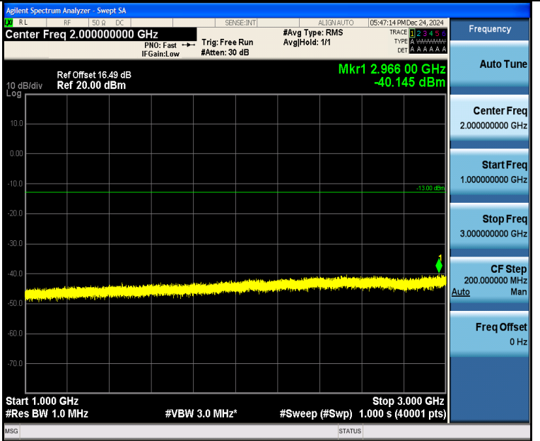
Band5_1.4MHz_QPSK_20643_1RB#5_1000~3000_1000~3000
