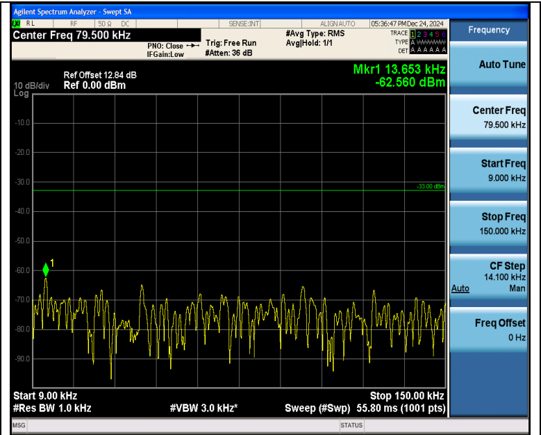
Band5_1.4MHz_16QAM_20407_6RB#0_0.009~0.15_0.009~0.15
