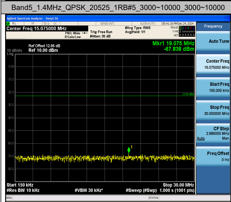
Band5_1.4MHz_QPSK_20525_1RB#5_3000~10000_3000~10000
