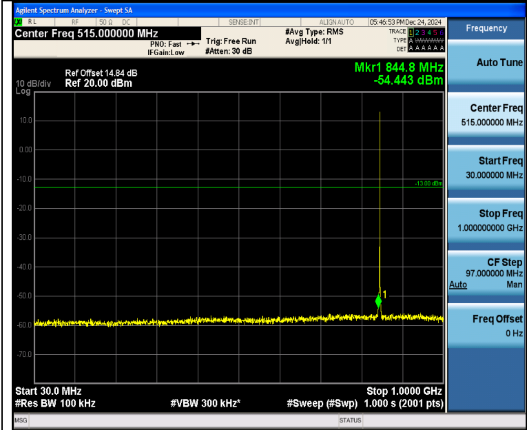
Band5_1.4MHz_QPSK_20643_1RB#5_30~1000_30~1000
