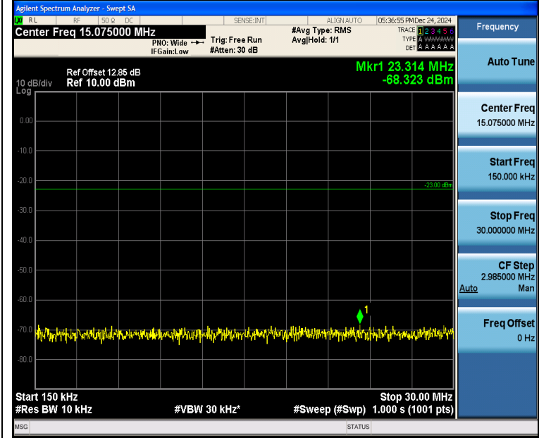
Band5_1.4MHz_16QAM_20407_6RB#0_0.15~30_0.15~30
