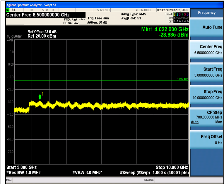
Band5_1.4MHz_QPSK_20407_6RB#0_3000~10000_3000~10000
