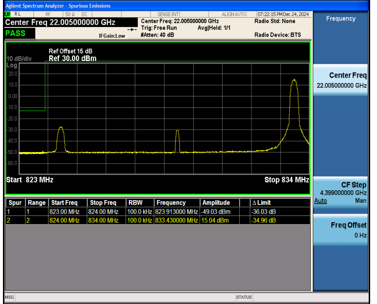
Band5_10MHz_16QAM_20450_1RB#49
