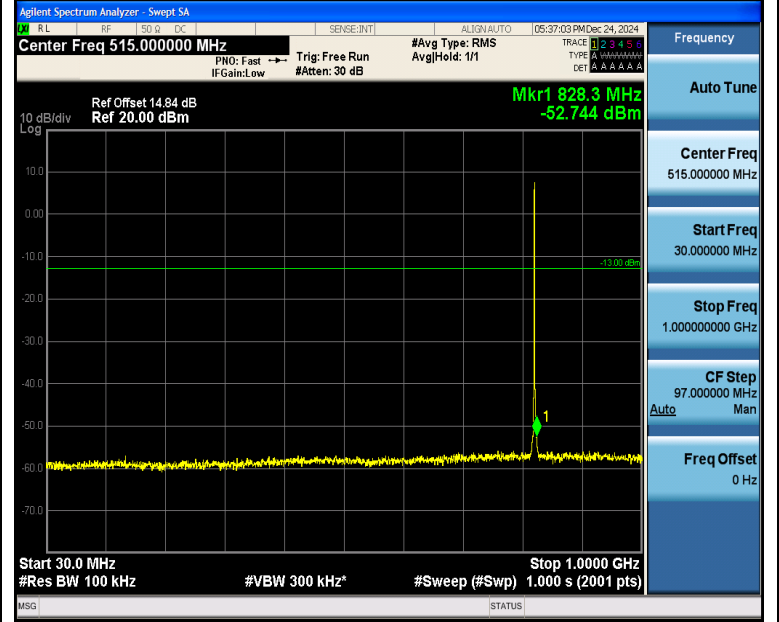
Band5_1.4MHz_16QAM_20407_6RB#0_30~1000_30~1000
