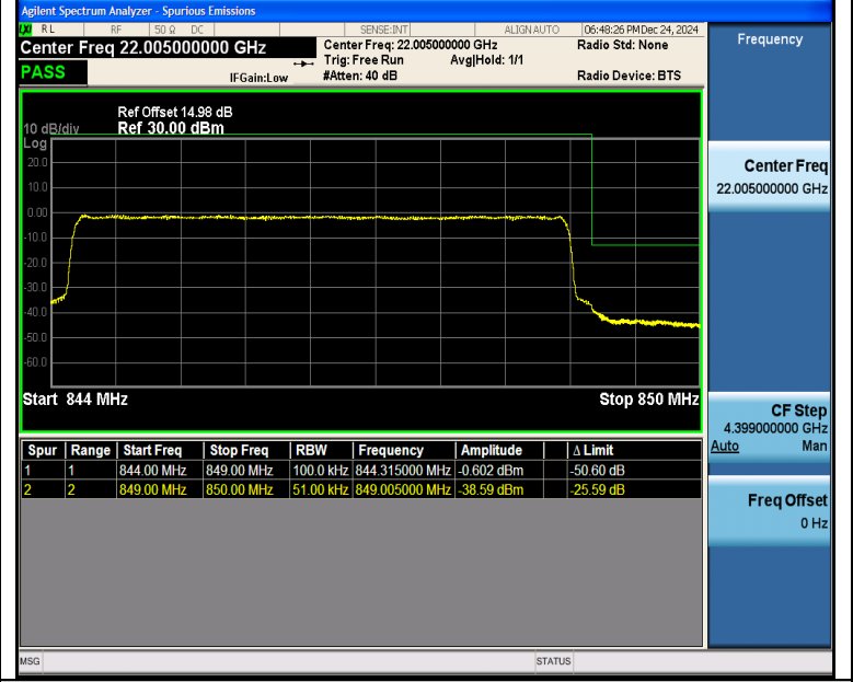
Band5_5MHz_16QAM_20625_25RB#0
