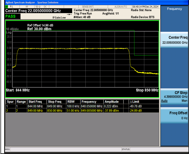
Band5_5MHz_QPSK_20625_25RB#0
