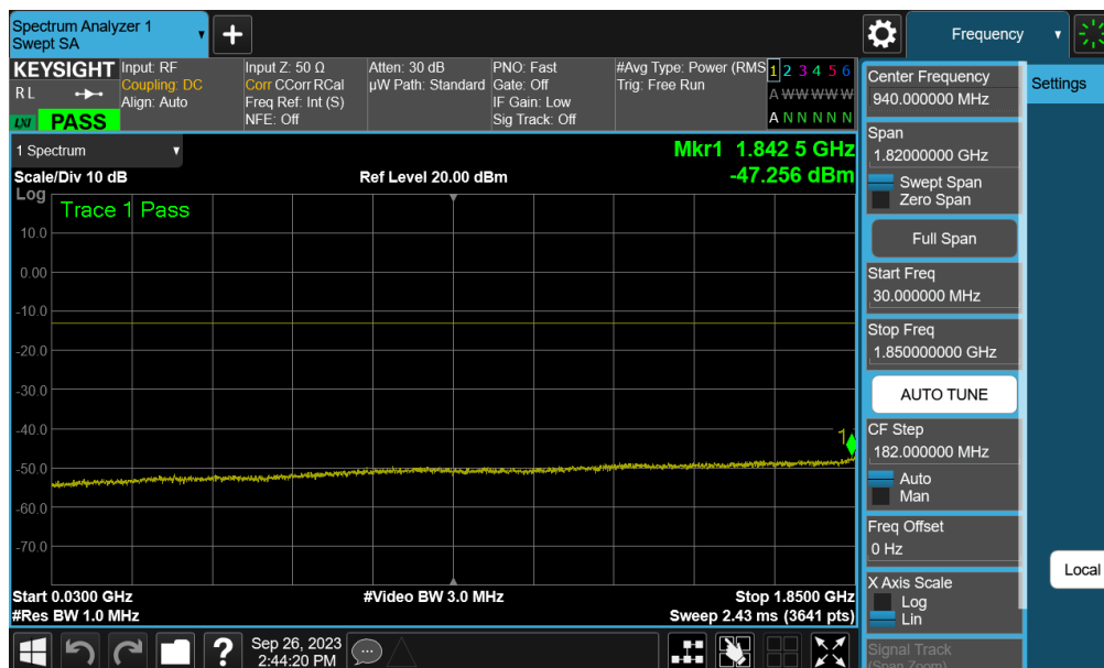
Plot 7-73. Conducted Spurious Plot (NR Band n25/2 - 40.0MHz - 1RB - Mid Channel - Ant M2)
