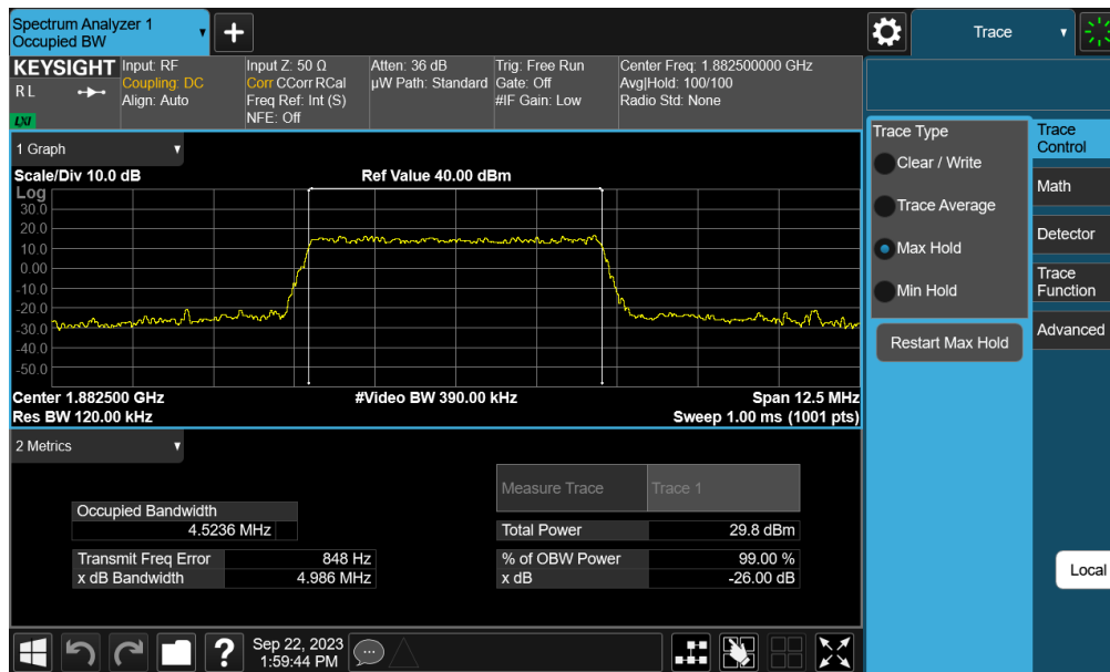
Plot 7-44. Occupied Bandwidth Plot (LTE Band 25/2 - 5MHz 16-QAM - Full RB - Ant M3)
