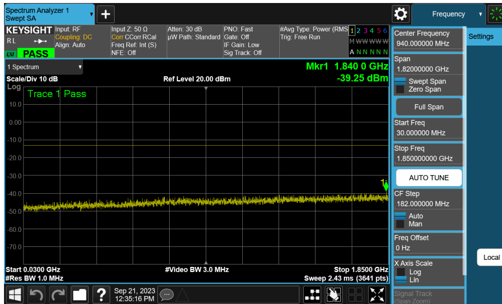
Plot 7-76. Conducted Spurious Plot (GPRS Ch. 661 - Ant M2)
