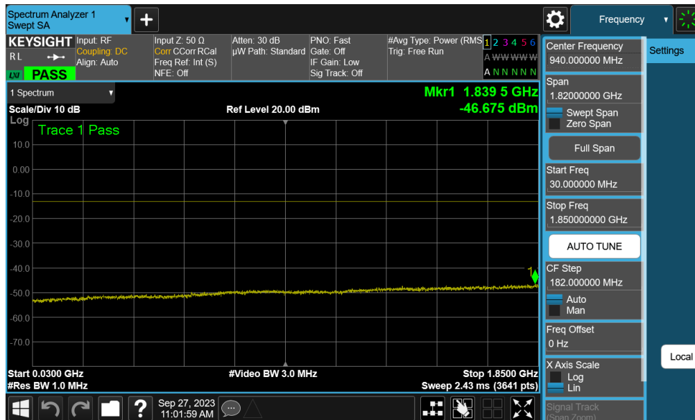
Plot 7-85. Conducted Spurious Plot (NR Band n2 - 20.0MHz - 1RB - Mid Channel - Ant M3)
