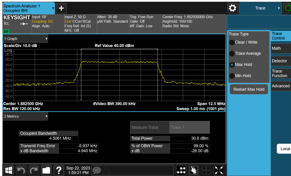
Plot 7-43. Occupied Bandwidth Plot (LTE Band 25/2 - 5MHz QPSK - Full RB - Ant M3)
