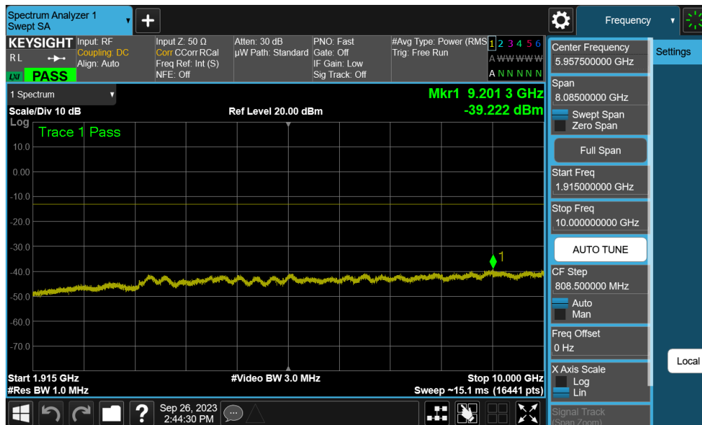
Plot 7-74. Conducted Spurious Plot (NR Band n25/2 - 40.0MHz - 1RB - Mid Channel - Ant M2)
