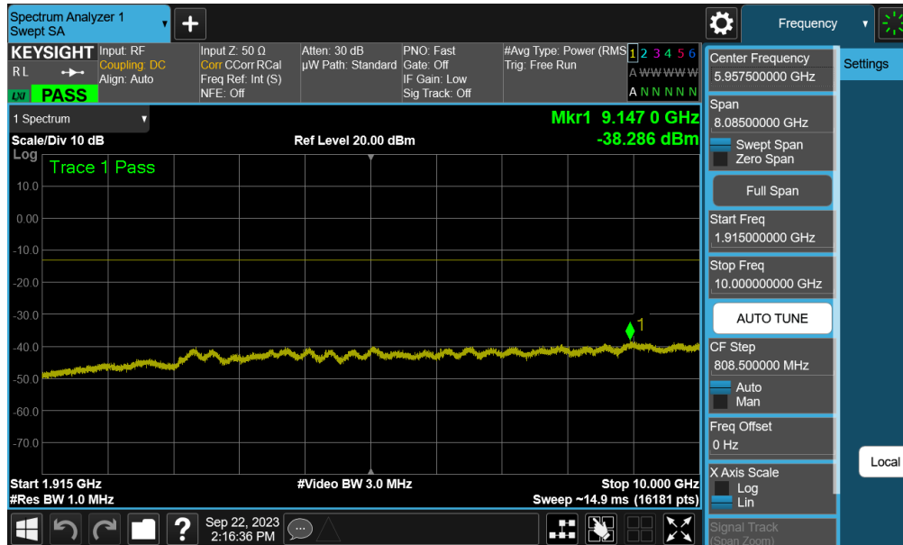
Plot 7-83. Conducted Spurious Plot (LTE Band 25/2 - 20MHz QPSK - 1RB - Mid Channel - Ant M3)
