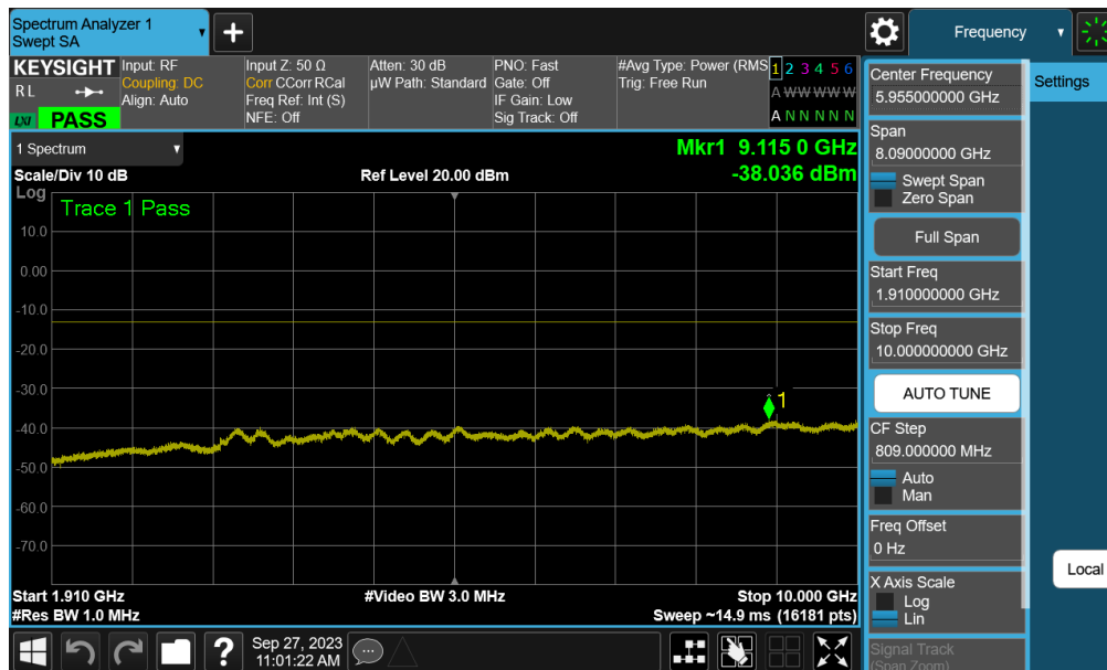
Plot 7-86. Conducted Spurious Plot (NR Band n2 - 20.0MHz - 1RB - Mid Channel - Ant M3)
