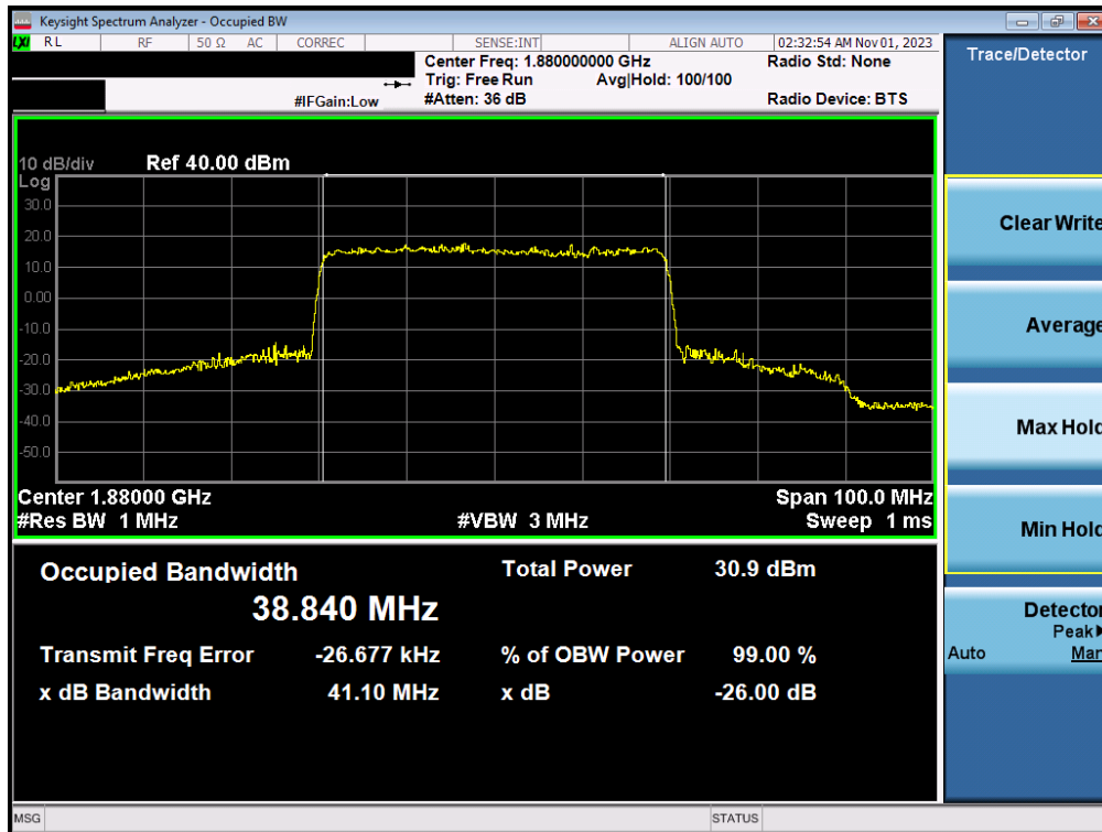
Plot 7-51. Occupied Bandwidth Plot (NR Band n2 - 40.0MHz CP-OFDM 16QAM - Full RB - ANT M3)
