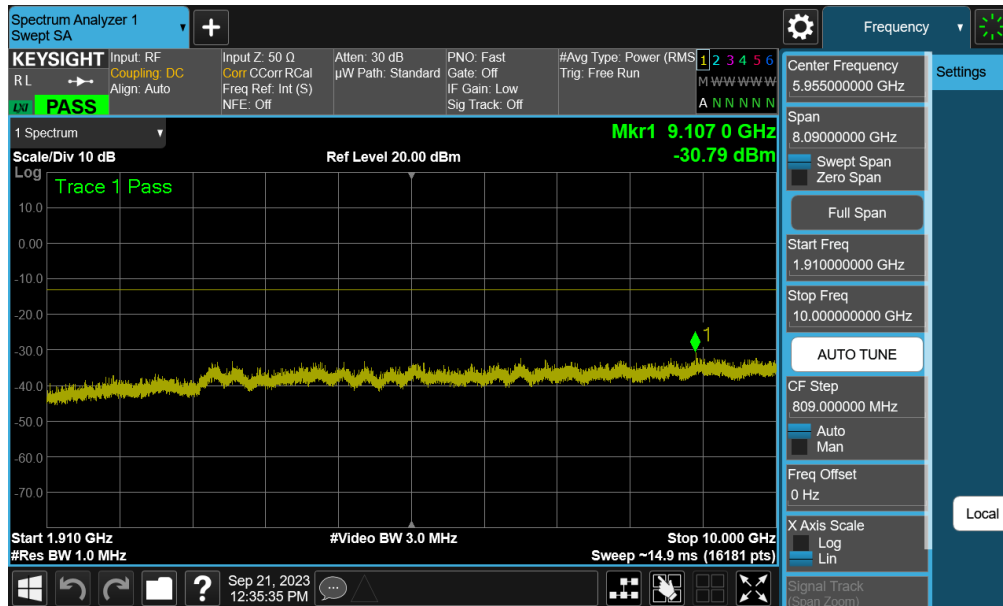
Plot 7-77. Conducted Spurious Plot (GPRS Ch. 661 - Ant M2)
