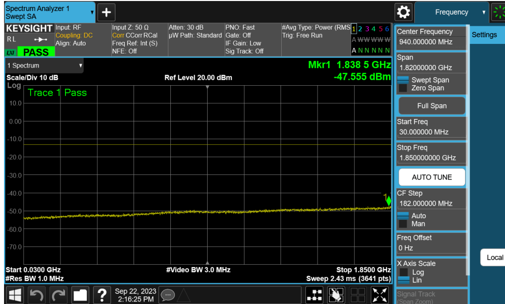
Plot 7-82. Conducted Spurious Plot (LTE Band 25/2 - 20MHz QPSK - 1RB - Mid Channel - Ant M3)
