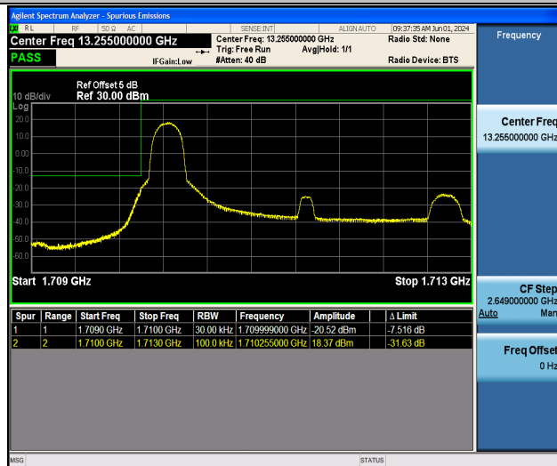
Band4_3MHz_16QAM_19965_1RB#0
