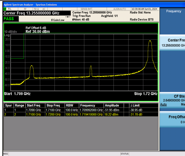
Band4_10MHz_16QAM_20000_1RB#49
