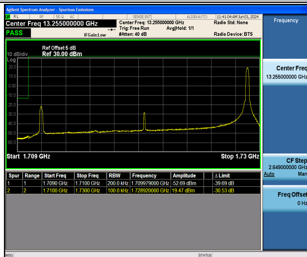
Band4_20MHz_QPSK_20050_1RB#99
