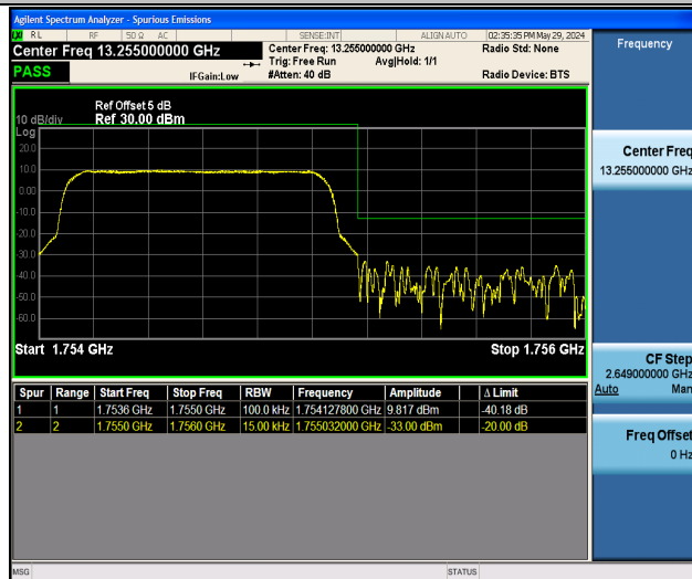
Band4_1.4MHz_QPSK_20393_6RB#0
