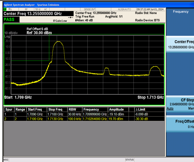
Band4_3MHz_QPSK_19965_1RB#0
