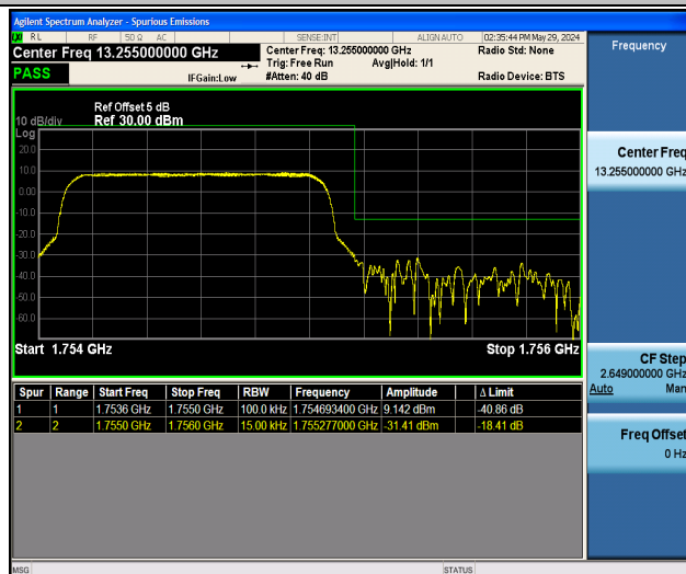
Band4_1.4MHz_16QAM_20393_6RB#0
