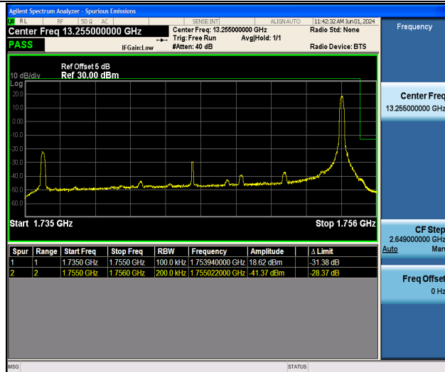
Band4_20MHz_16QAM_20300_1RB#99
