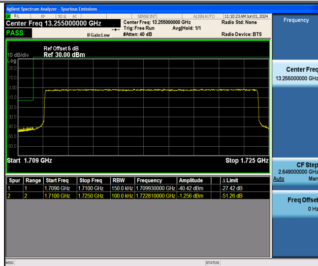
Band4_15MHz_QPSK_20025_75RB#0
