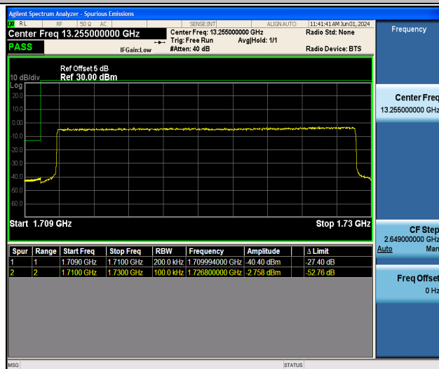
Band4_20MHz_16QAM_20050_100RB#0
