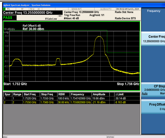
Band4_3MHz_QPSK_20385_1RB#14
