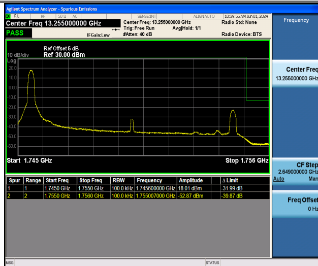
Band4_10MHz_16QAM_20350_1RB#0
