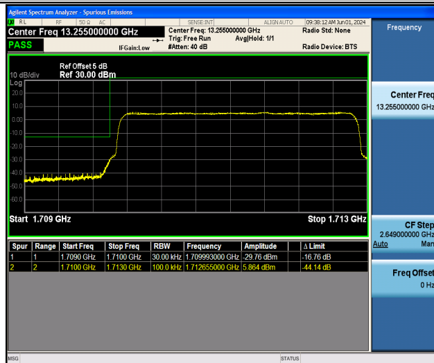
Band4_3MHz_QPSK_19965_15RB#0
