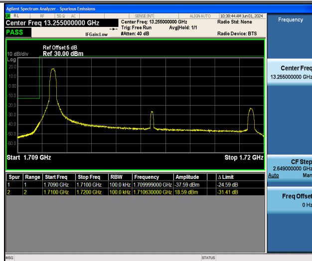
Band4_10MHz_16QAM_20000_1RB#0
