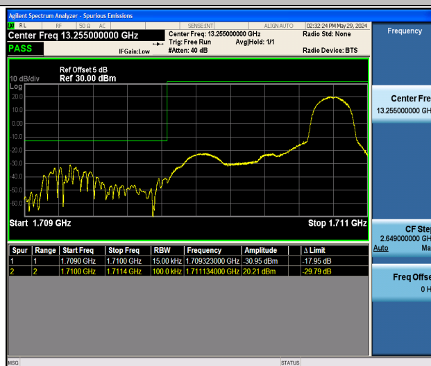
Band4_1.4MHz_QPSK_19957_1RB#5
