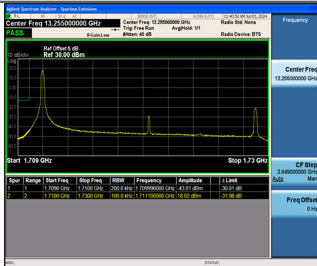
Band4_20MHz_16QAM_20050_1RB#0
