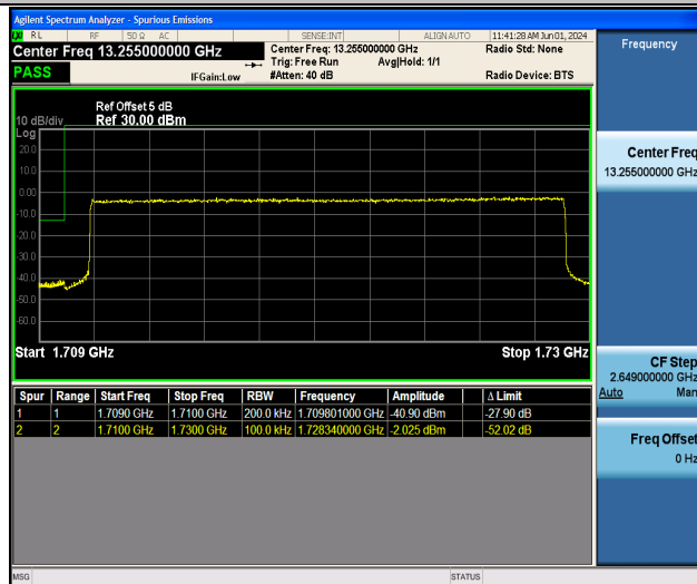
Band4_20MHz_QPSK_20050_100RB#0
