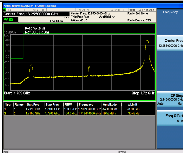
Band4_10MHz_QPSK_20000_1RB#49
