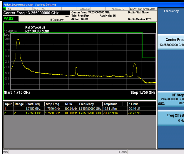
Band4_10MHz_QPSK_20350_1RB#0
