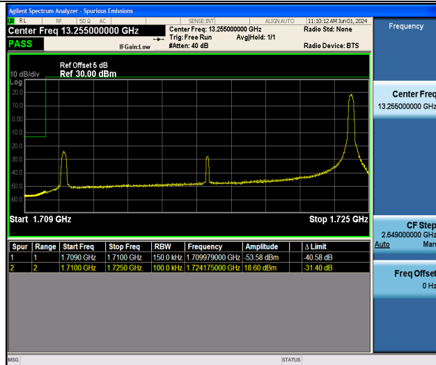
Band4_15MHz_16QAM_20025_1RB#74
