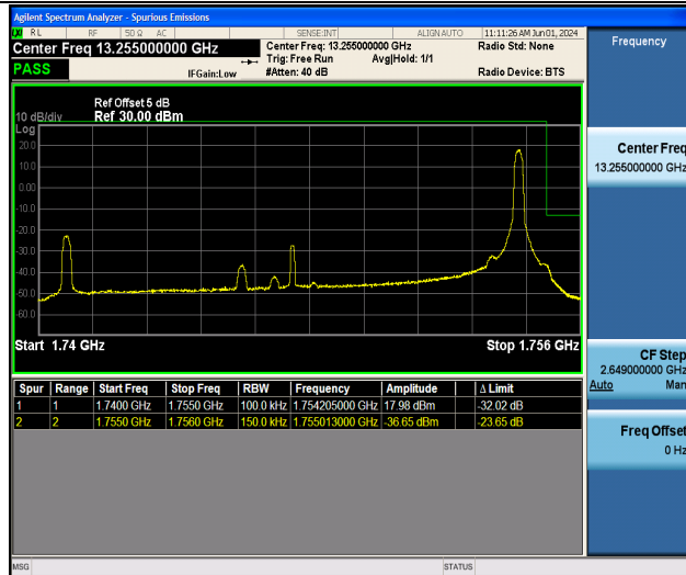
Band4_15MHz_16QAM_20325_1RB#74
