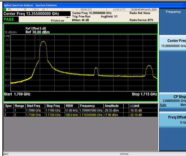
Band4_5MHz_16QAM_19975_1RB#0
