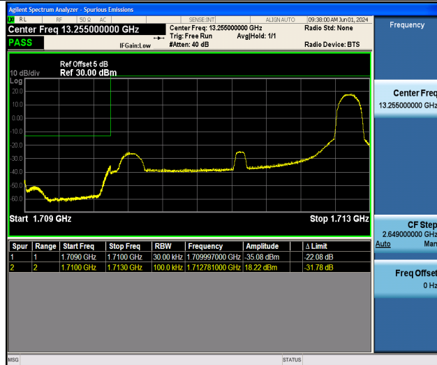
Band4_3MHz_16QAM_19965_1RB#14
