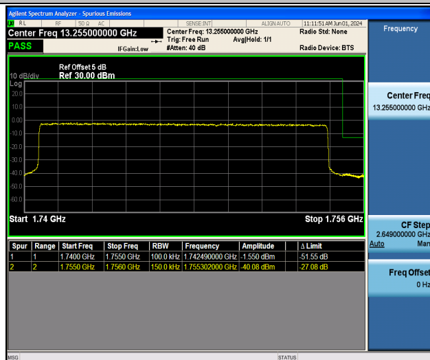
Band4_15MHz_16QAM_20325_75RB#0
