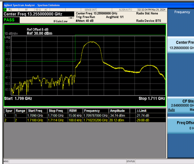
Band4_1.4MHz_QPSK_19957_1RB#0
