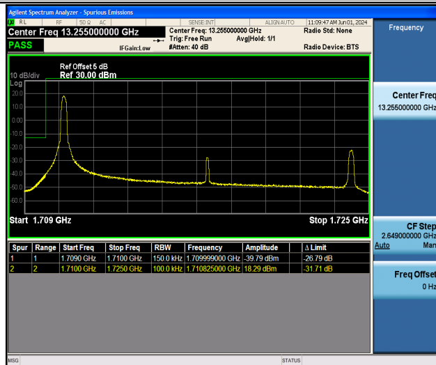
Band4_15MHz_16QAM_20025_1RB#0
