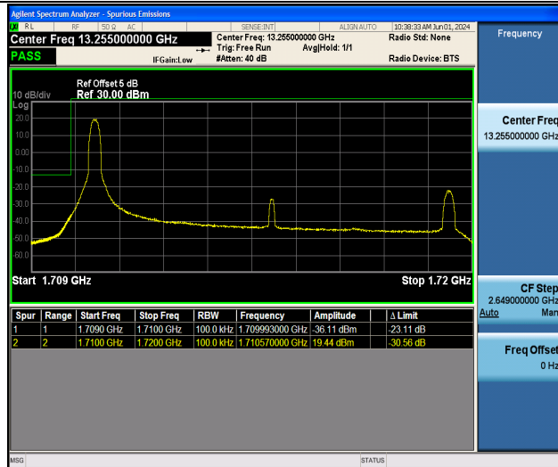
Band4_10MHz_QPSK_20000_1RB#0
