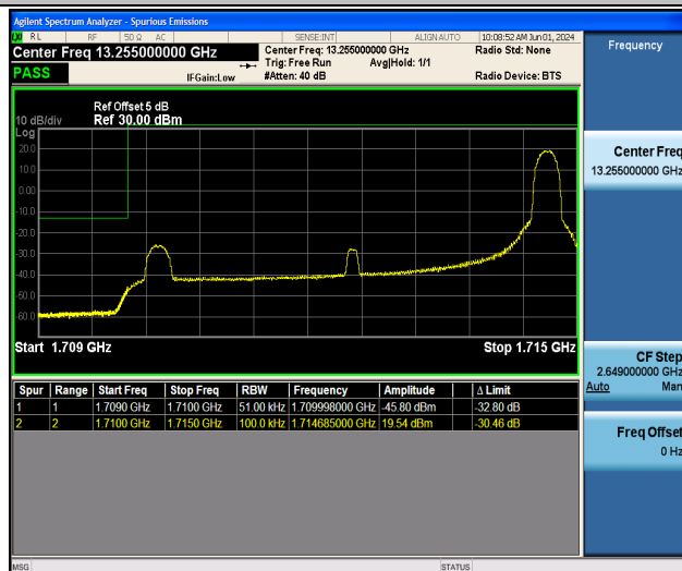
Band4_5MHz_QPSK_19975_1RB#24
