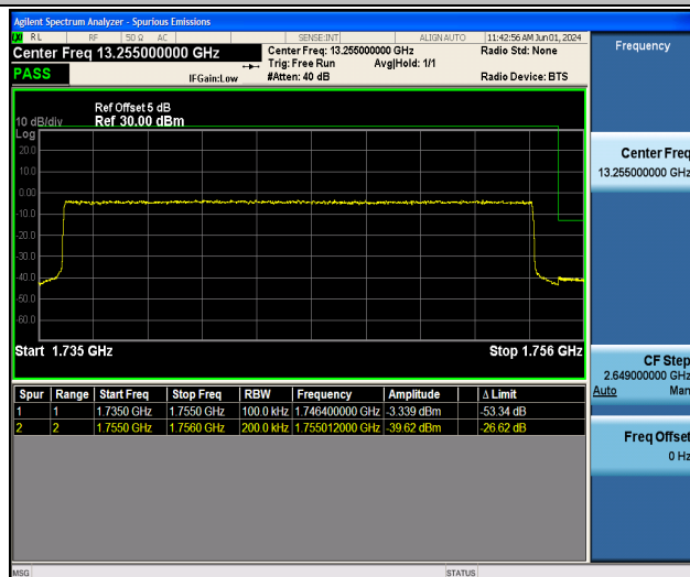
Band4_20MHz_16QAM_20300_100RB#0
