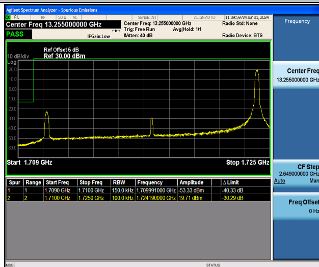
Band4_15MHz_QPSK_20025_1RB#74
