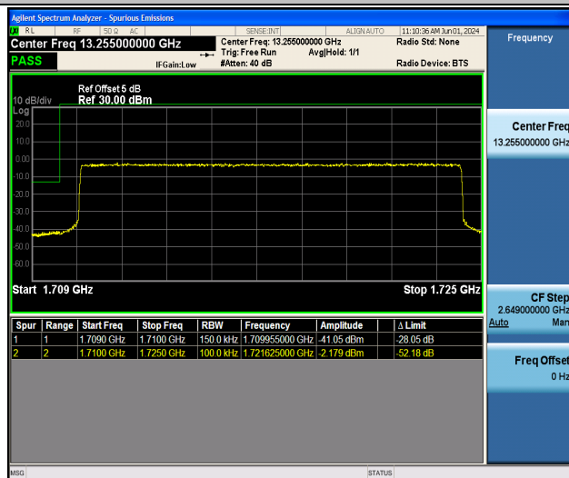
Band4_15MHz_16QAM_20025_75RB#0
