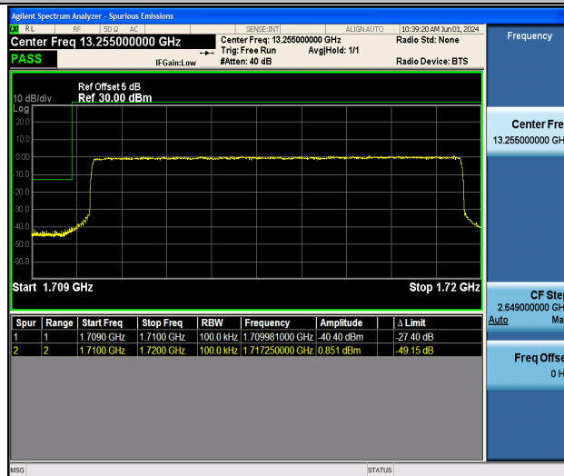
Band4_10MHz_QPSK_20000_50RB#0
