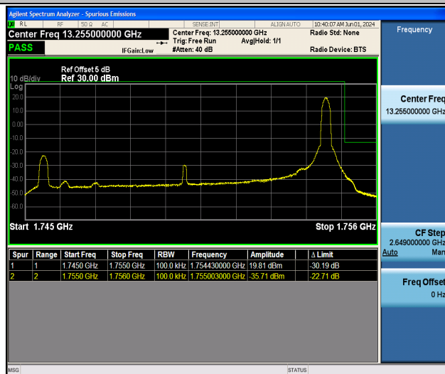
Band4_10MHz_QPSK_20350_1RB#49
