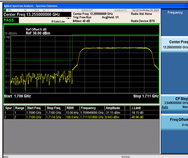
Band4_1.4MHz_16QAM_19957_6RB#0
