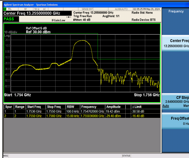
Band4_1.4MHz_16QAM_20393_1RB#5
