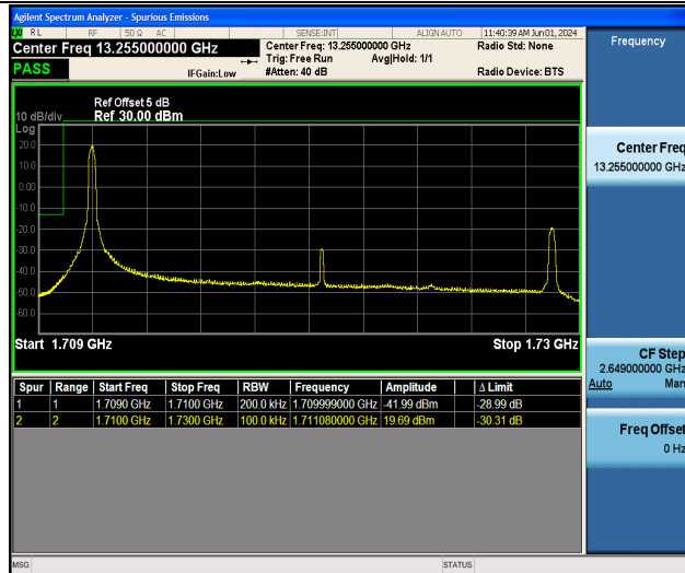
Band4_20MHz_QPSK_20050_1RB#0
