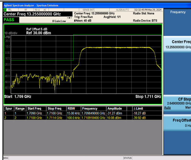
Band4_1.4MHz_QPSK_19957_6RB#0
