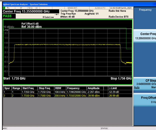
Band4_20MHz_QPSK_20300_100RB#0
