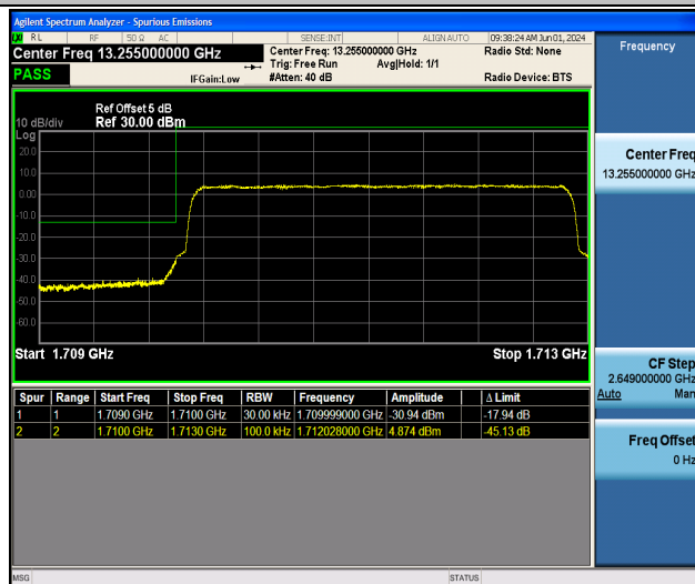
Band4_3MHz_16QAM_19965_15RB#0
