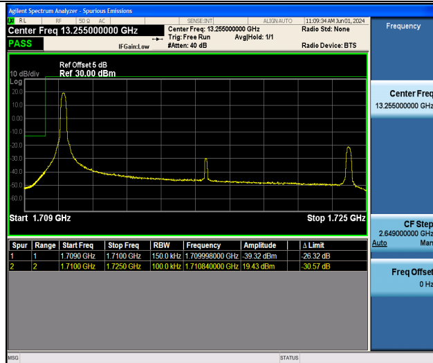
Band4_15MHz_QPSK_20025_1RB#0
