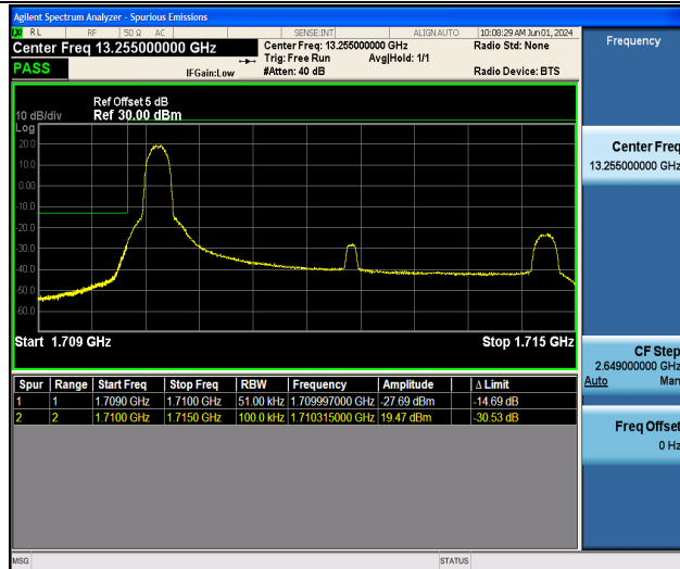
Band4_5MHz_QPSK_19975_1RB#0
