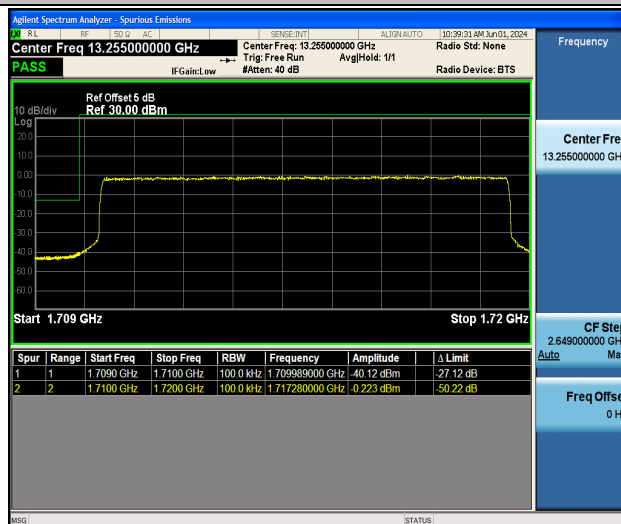
Band4_10MHz_16QAM_20000_50RB#0
