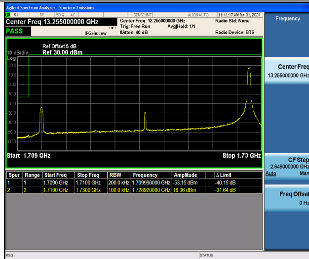
Band4_20MHz_16QAM_20050_1RB#99
