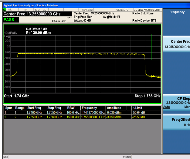
Band4_15MHz_QPSK_20325_75RB#0
