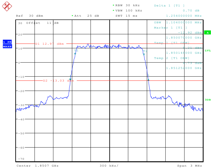
Band 2_1.4 MHz_Low_QPSK_RB6#0
