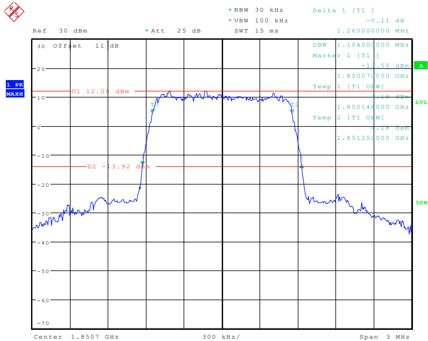
Band 2_1.4 MHz_Low_16QAM_RB6#0
