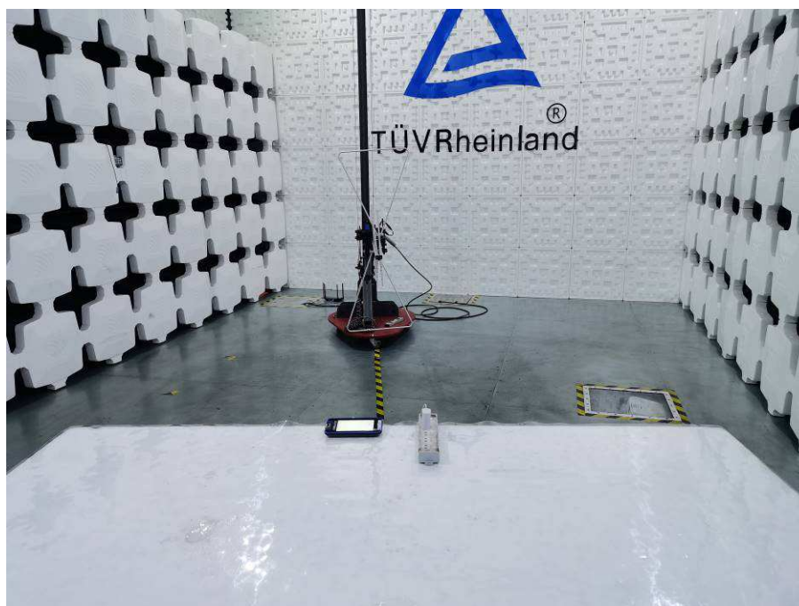
Photograph 3: Set-up photo for Radiated Emissions Below 1GHz
