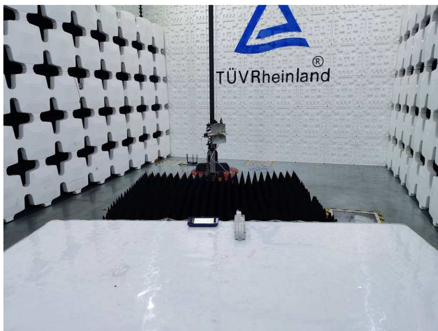
Photograph 4: Set-up photo for Radiated Emissions Above 1GHz
