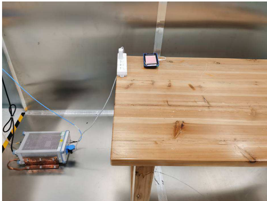
Photograph 5: Set-up photo for Conducted Emission on AC Mains
