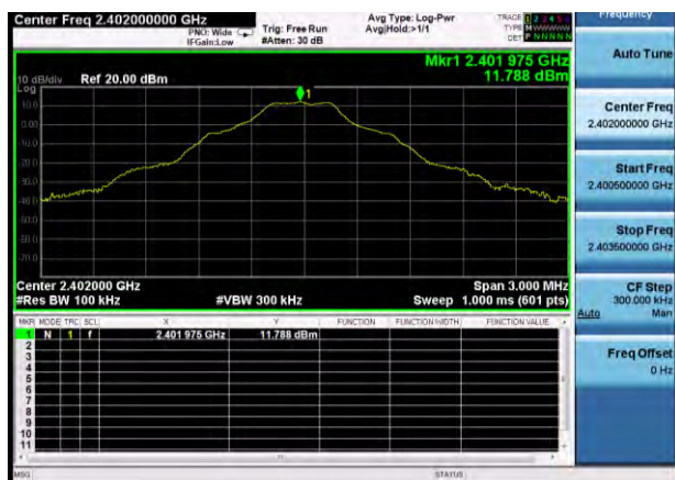
GFSK LOW CHANNEL, CARRIER LEVEL
