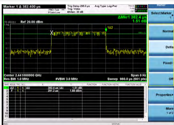
8-DPSK 3DH1
