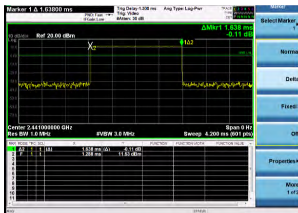
GFSK DH3
