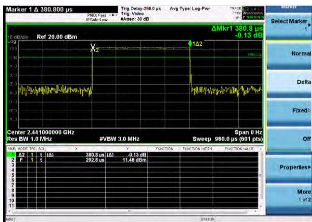
GFSK DH1
