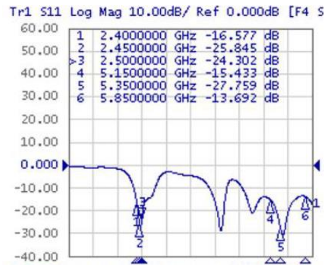
Figure 1 Return Loss
