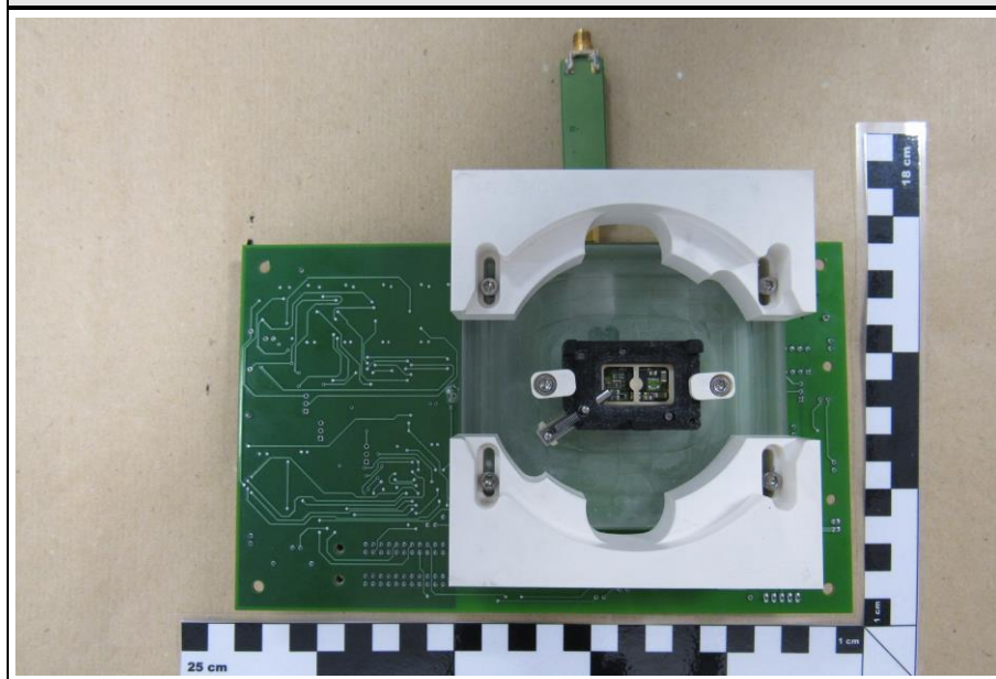
BM2 Module test Fixture bottom
