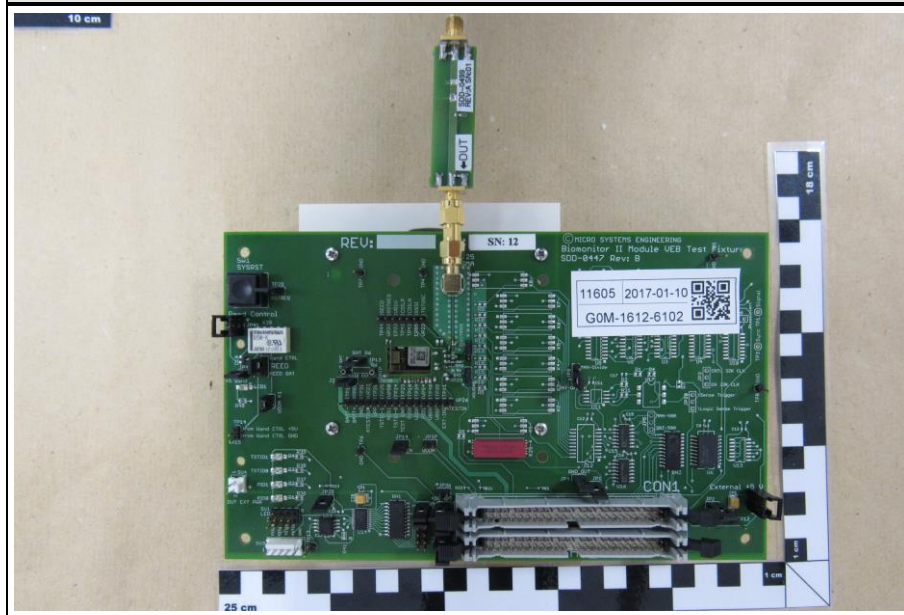
BM2 Module test Fixture top
