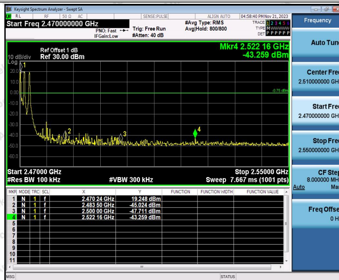
2.4G_Ant1_High_Hop_2472.94
