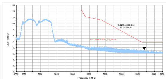
802.11n HT40-Channel 159: Peak
