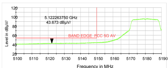
802.11a-Channel 36: Average
