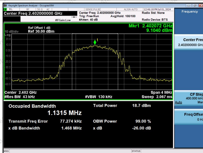
BLE_1M-Ant1-2402
