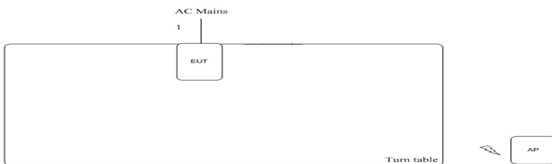
Test Setup Diagram - Radiated Test <1G
