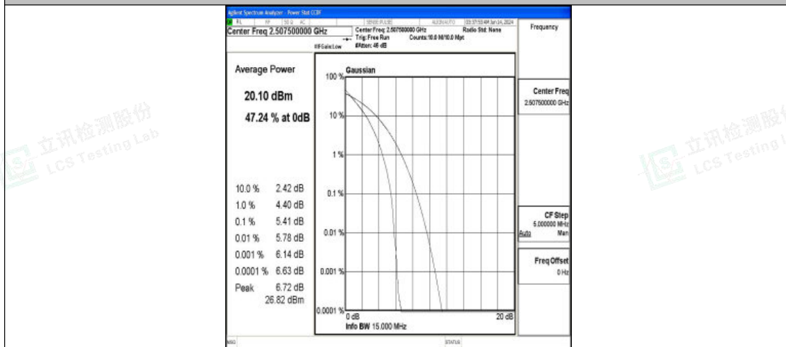
Band7-15MHz-QPSK-20825-75RB#0-PASS
