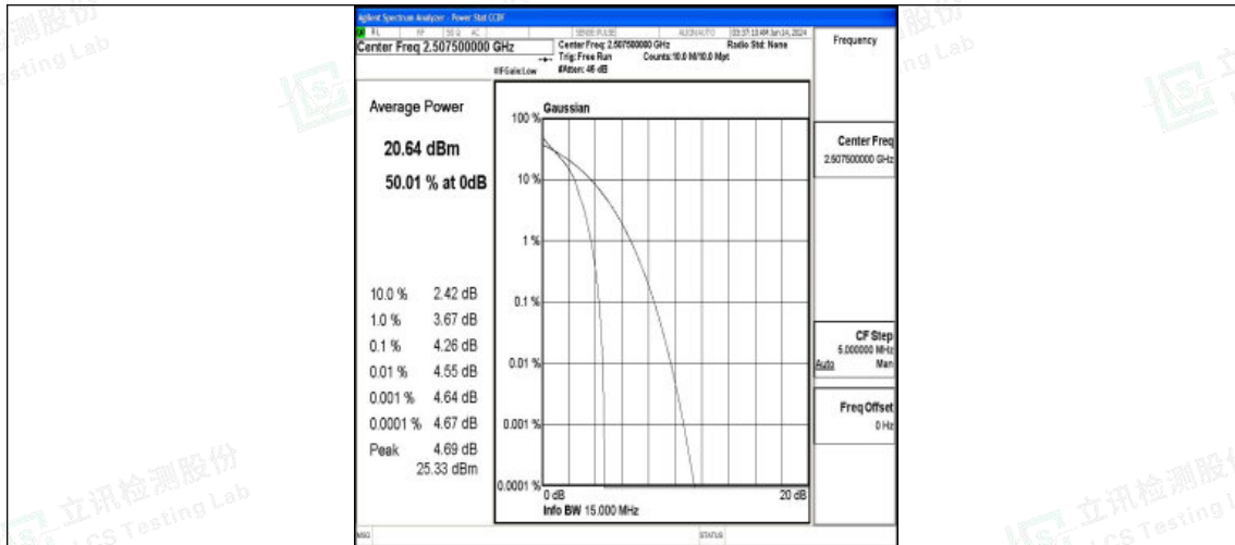
Band7-15MHz-QPSK-20825-1RB#0-PASS
