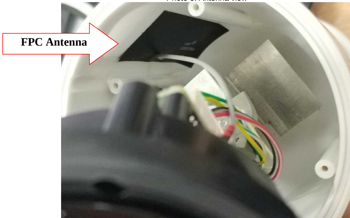
Photo 6. Antenna view
