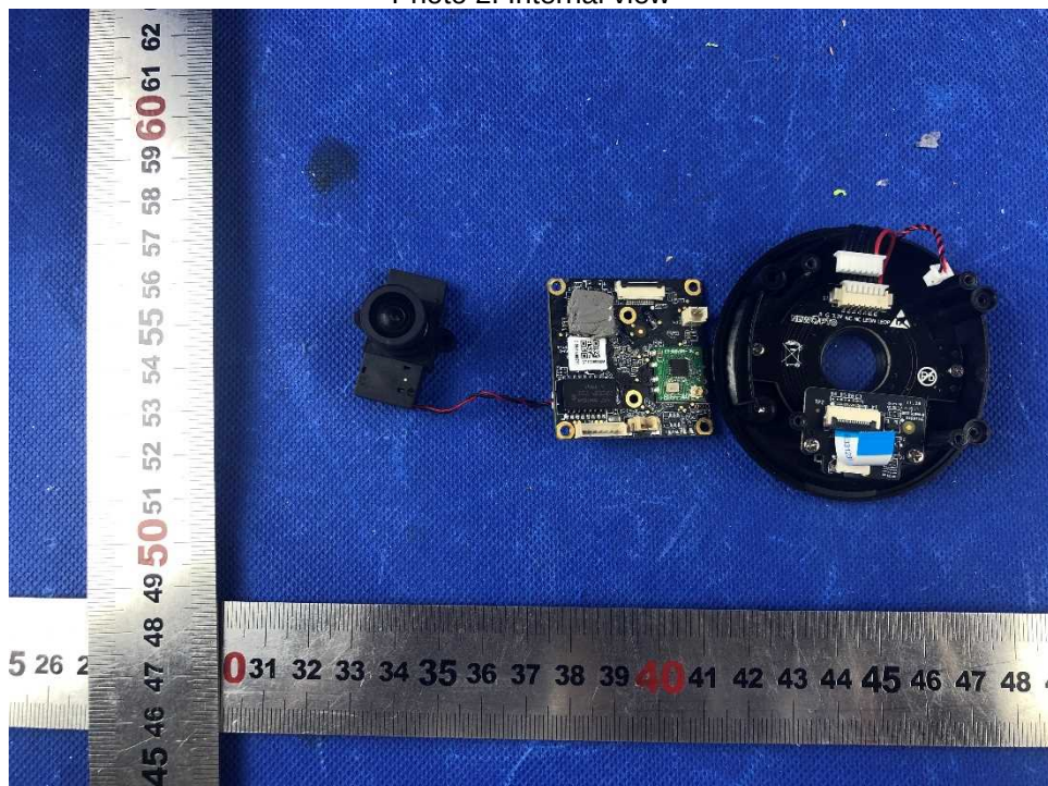
Photo 2. Internal view
