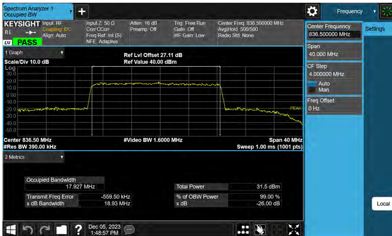
Sub6 n5. Occupied Bandwidth Plot (20 M BW Ch.167300 QPSK_ Full RB _0)
