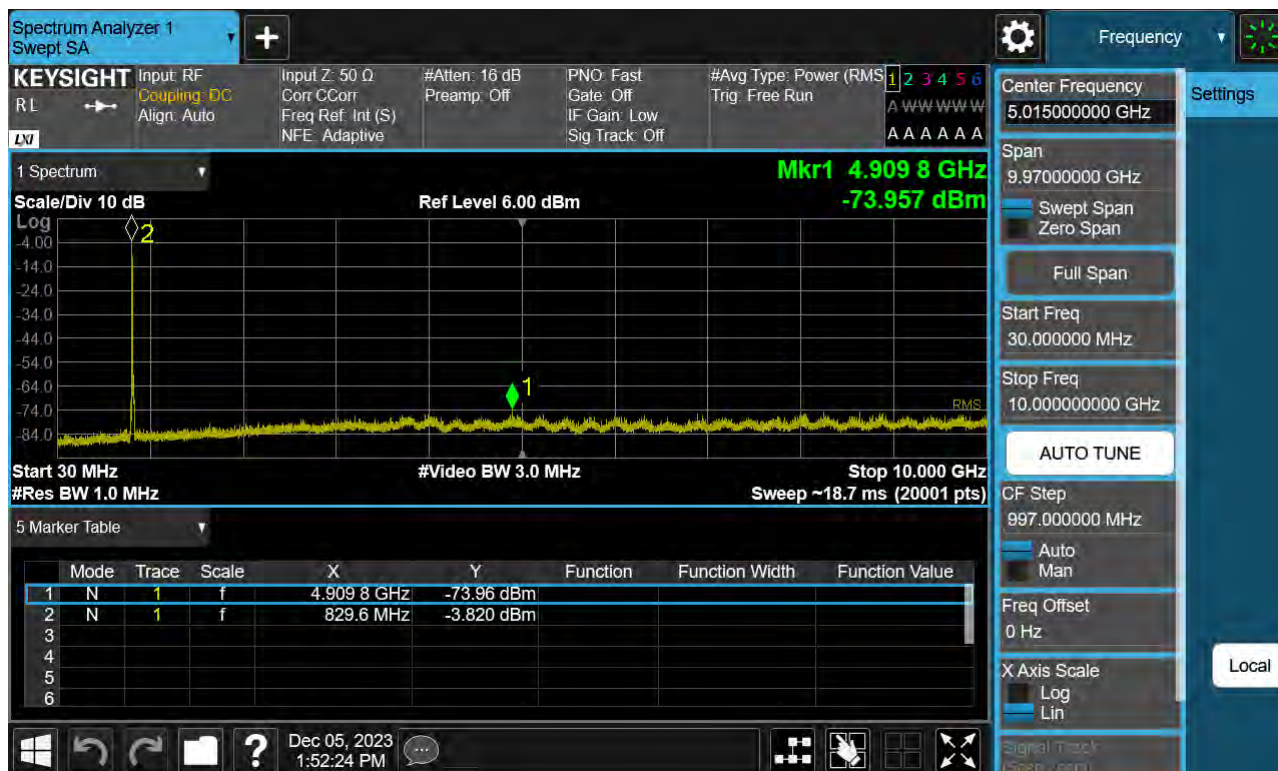
Sub6 n5. Conducted Spurious Plot (167800ch_20 MHz_BPSK_RB 1_1)
