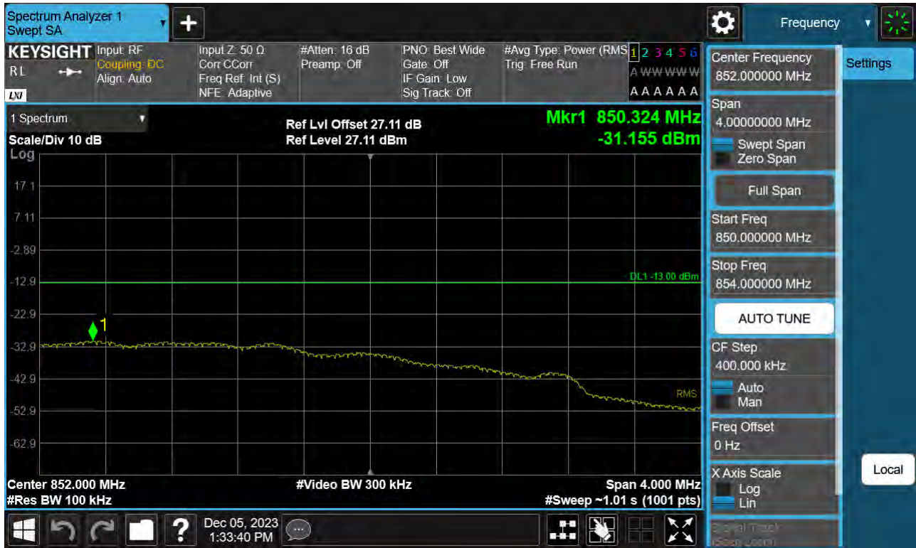
Sub6 n5. Upper Extended Band Edge Plot (5 M BW Ch.169300 BPSK_RB25_0)
