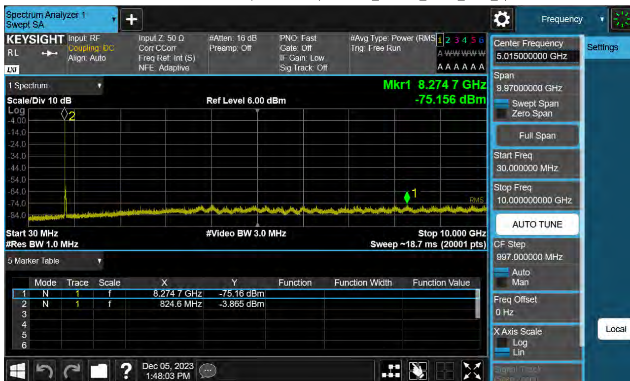
Sub6 n5. Conducted Spurious Plot (166800ch_20 MHz_BPSK_RB 1_1)
