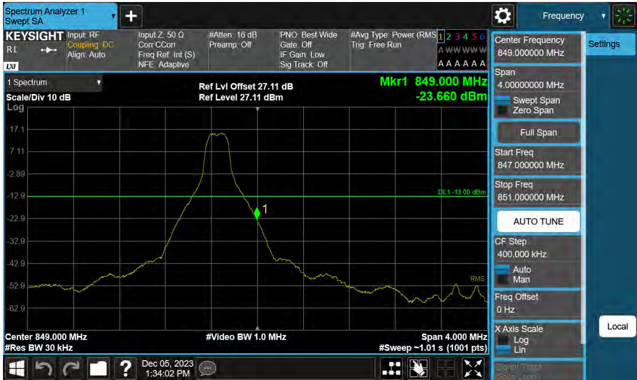
Sub6 n5. Upper Band Edge Plot (5 M BW Ch.169300 BPSK_RB1_Offset 24)
