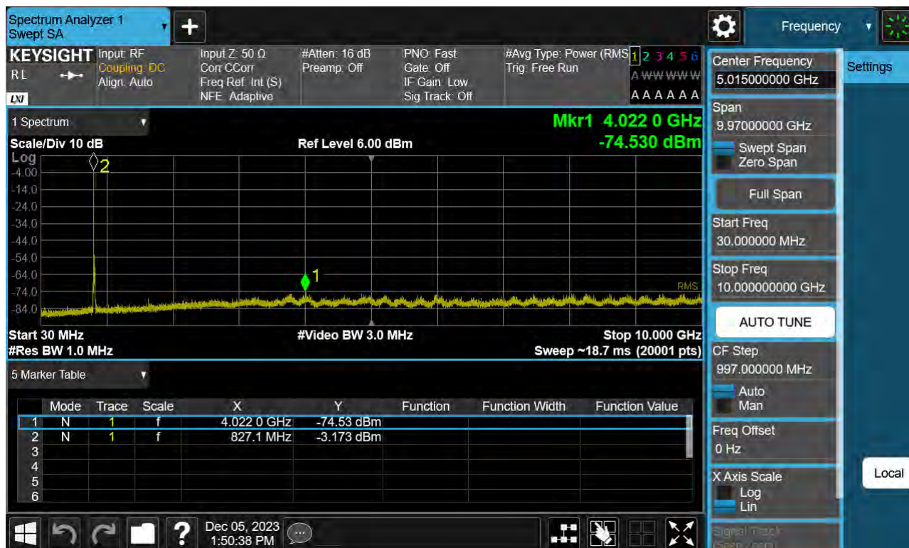
Sub6 n5. Conducted Spurious Plot (167300ch_20 MHz_BPSK_RB 1_1)
